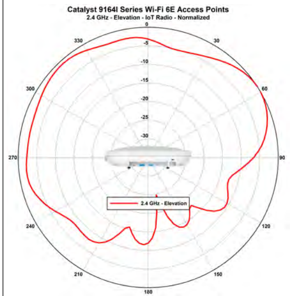
Figure 16: CW9164I - IoT (BLE) Antenna-Normalized Radiation Pattern (2.4-GHz Elevation)
