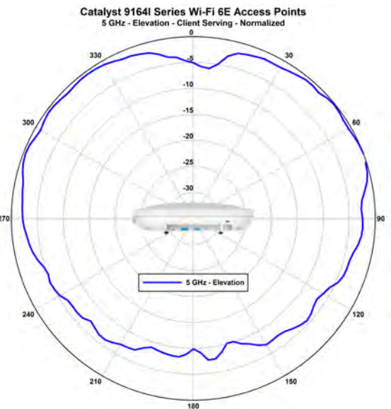
Figure 6: CW9164I - Client-Serving Normalized Radiation Pattern (5-GHz Elevation)
