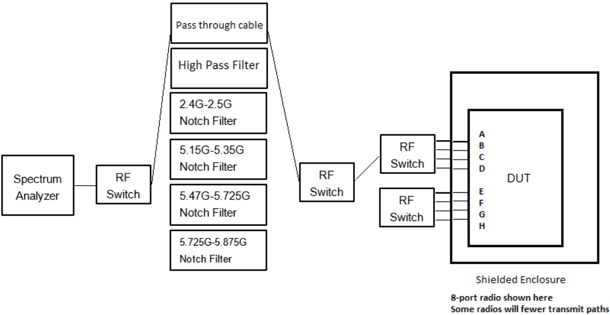
Conducted Test Setup Diagram
