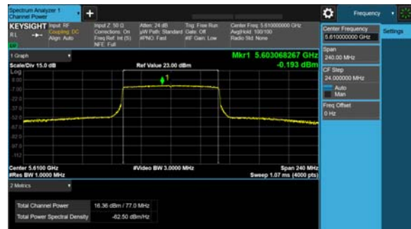
Antenna B
