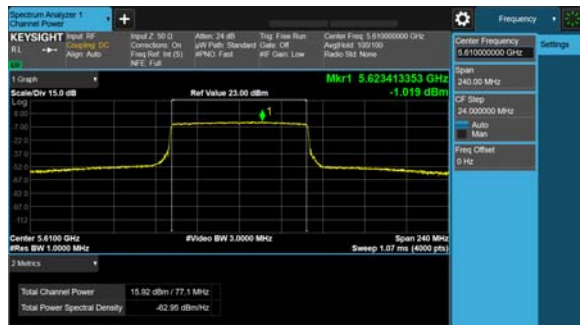
Antenna C
