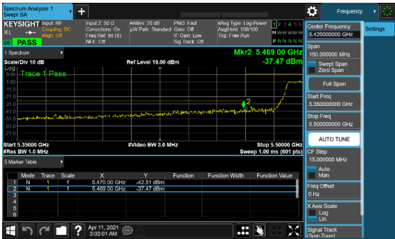
Antenna B
