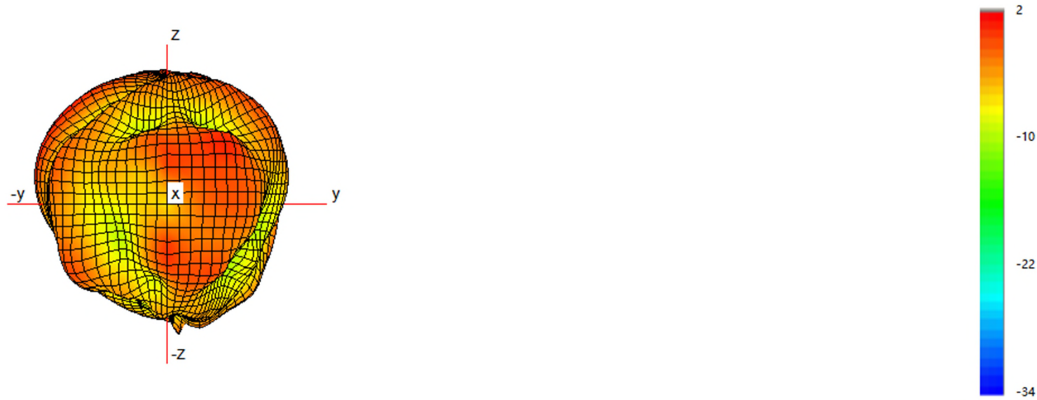
@2.45GHz
