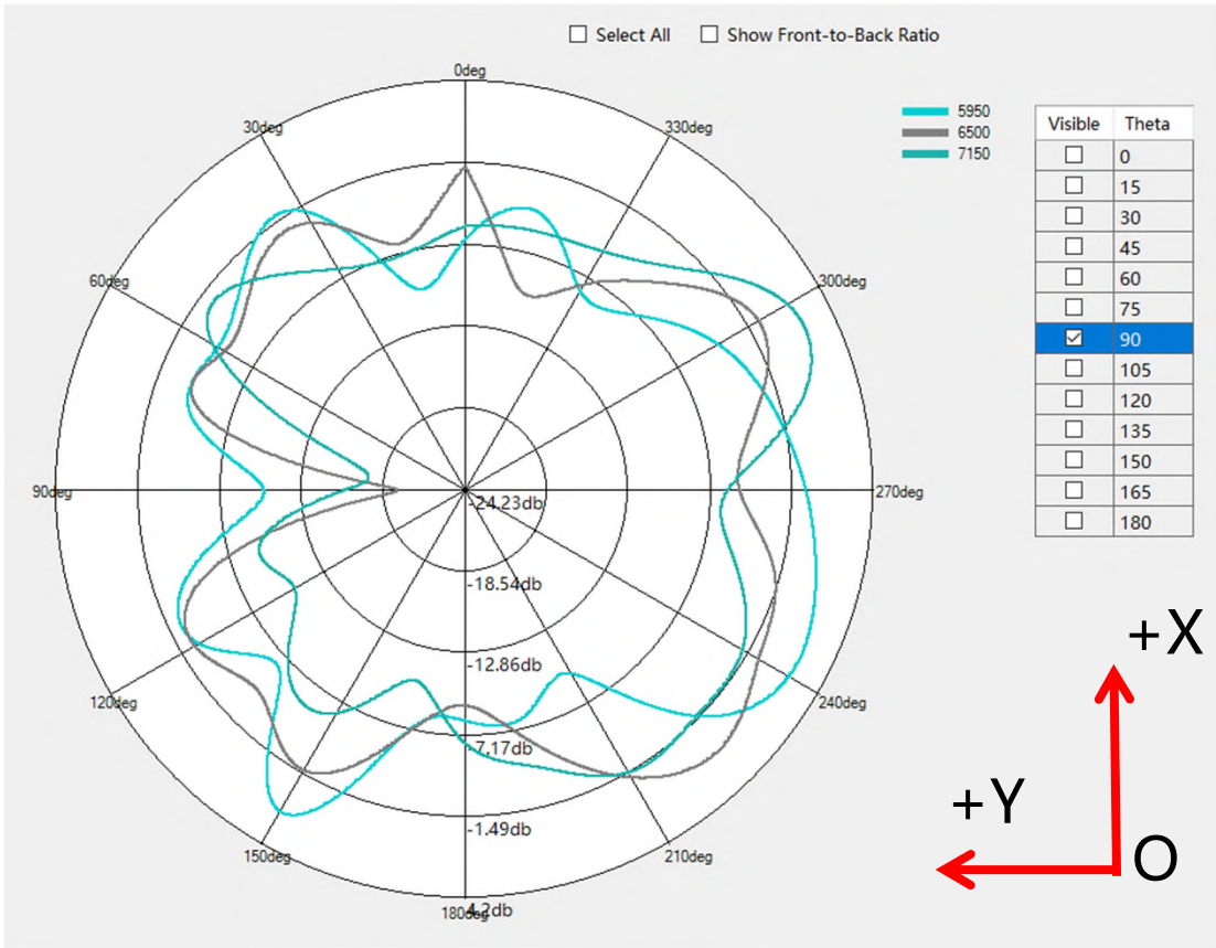
XOY plane
