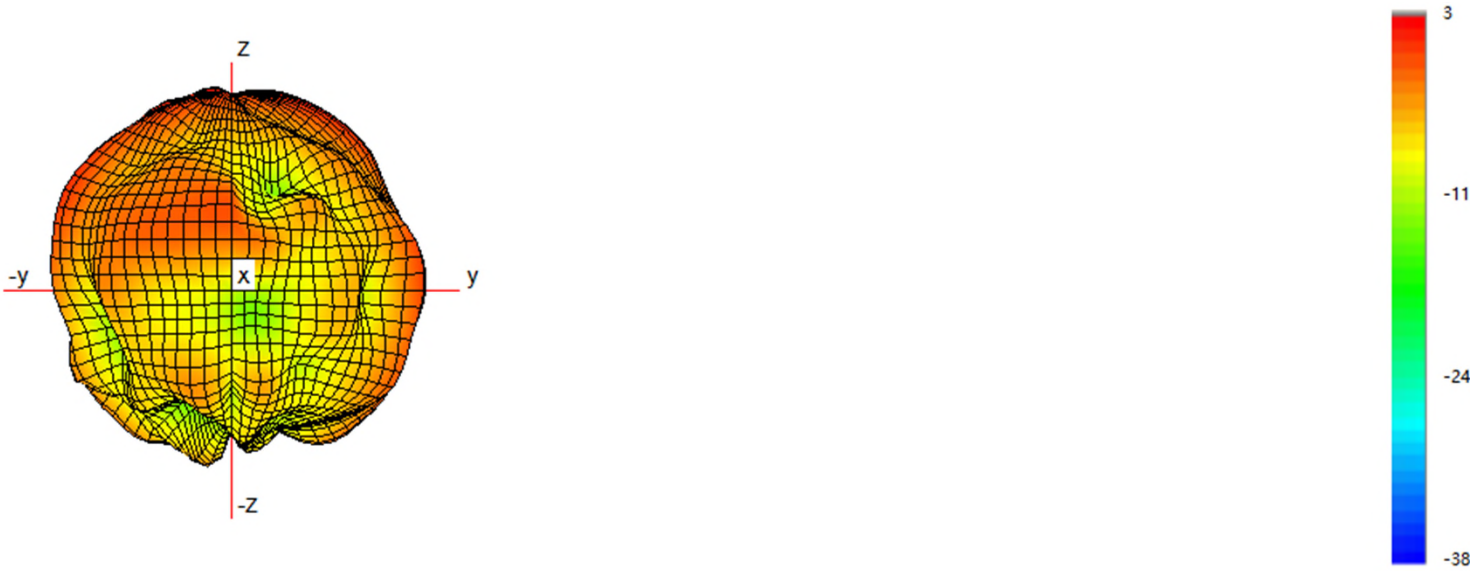
@5.5GHz
