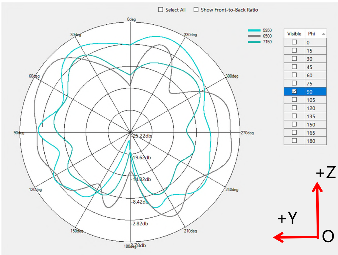
YOZ plane
