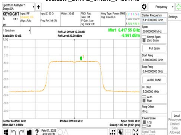
802.11ax_20MHz_Chain0_6415MHz_RU26_8
