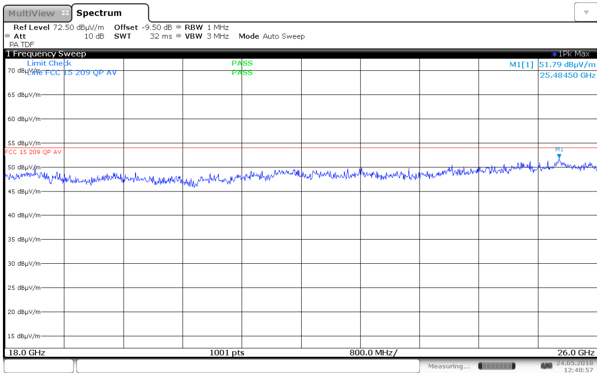
Radiated Emissions, 18.0 – 26.0GHz, 5580 MHz, 802.11a 6M, Ant 1, VP, @1m
