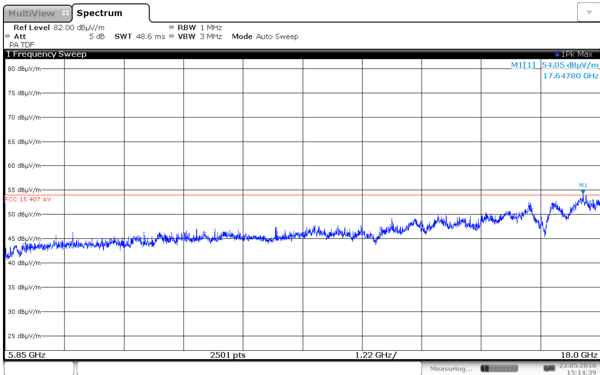
Radiated Emissions, 5850 – 18000 MHz, 5785 MHz, 802.11a 6M, Ant0, VP
