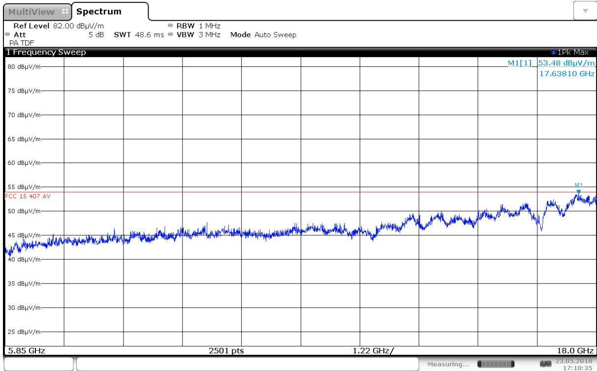
Radiated Emissions, 5850 – 18000 MHz, 5785 MHz, 802.11a 6M, Ant1, HP
