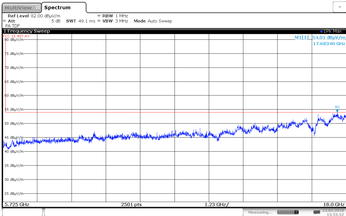
Radiated Emissions, 5725 – 18000 MHz, 5700 MHz, 802.11n HT20, MIMO, VP
