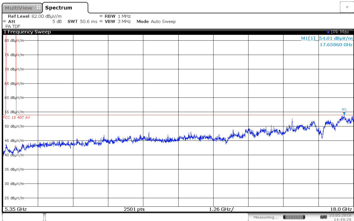
Radiated Emissions, 5350 – 18000 MHz, 5260 MHz, 802.11a 6M, Ant0, VP
