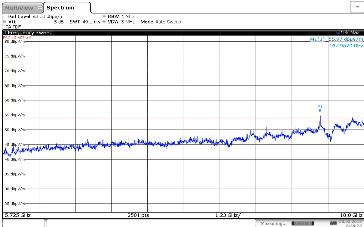
Radiated Emissions, 5725 – 18000 MHz, 5500 MHz, 802.11a 6M, Ant0, HP (Emission detected at 16.5 GHz is not in a Restricted Band)
