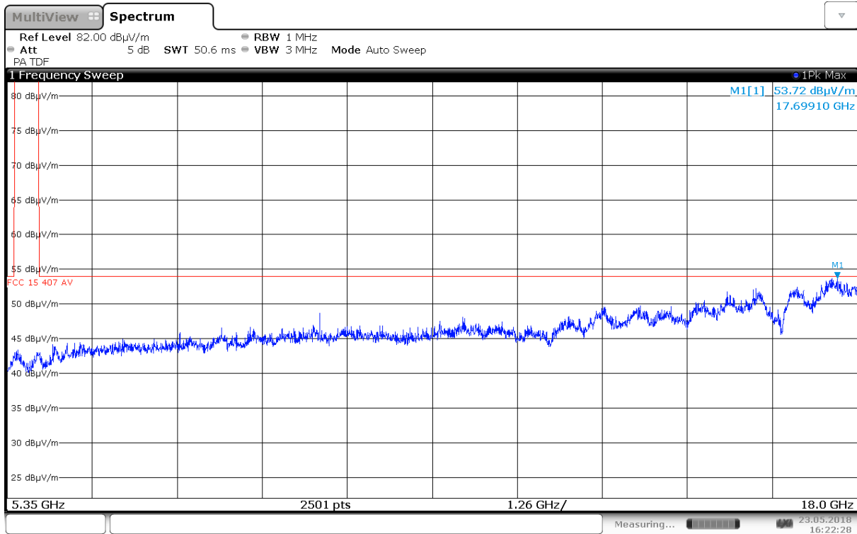
Radiated Emissions, 5350 – 18000 MHz, 5240 MHz, 802.11n HT20, MIMO, HP
