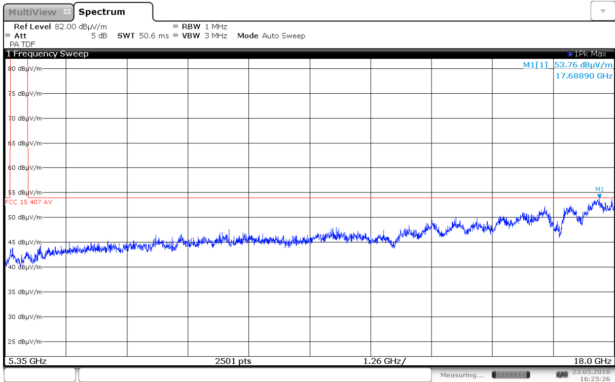
Radiated Emissions, 5350 – 18000 MHz, 5180 MHz, 802.11n HT20, MIMO, HP
