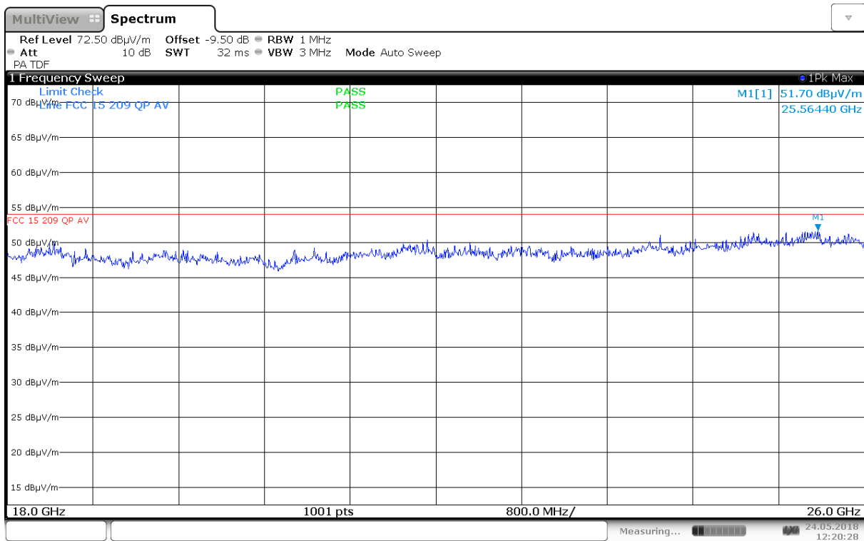
Radiated Emissions, 18.0 – 26.0GHz, 5300 MHz, 802.11a 6M, Ant 1, VP, @1m
