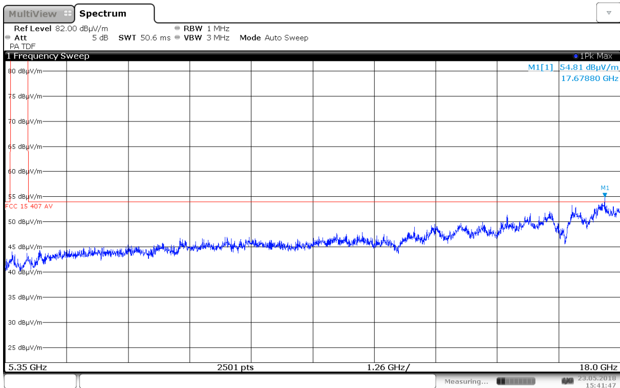
Radiated Emissions, 5350 – 18000 MHz, 5240 MHz, 802.11n HT20, MIMO, VP
