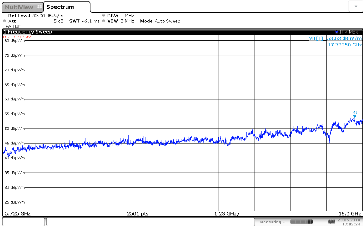
Radiated Emissions, 5725 – 18000 MHz, 5700 MHz, 802.11a 6M, Ant0, HP
