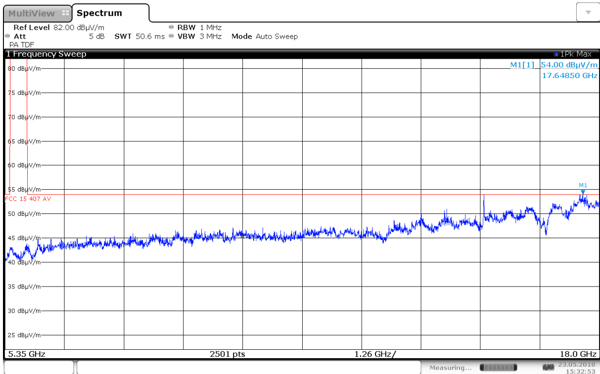
Radiated Emissions, 5350 – 18000 MHz, 5180 MHz, 802.11a 6M, Ant1, VP
