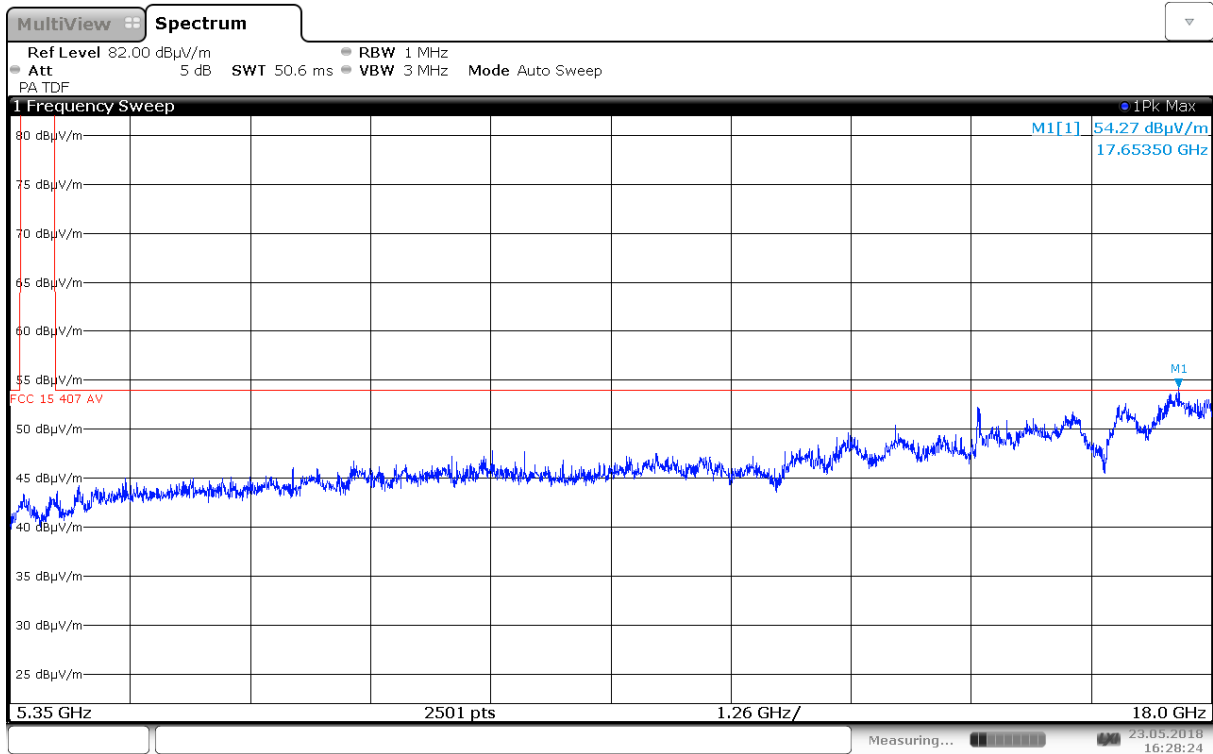
Radiated Emissions, 5350 – 18000 MHz, 5180 MHz, 802.11a 6M, Ant0, HP
