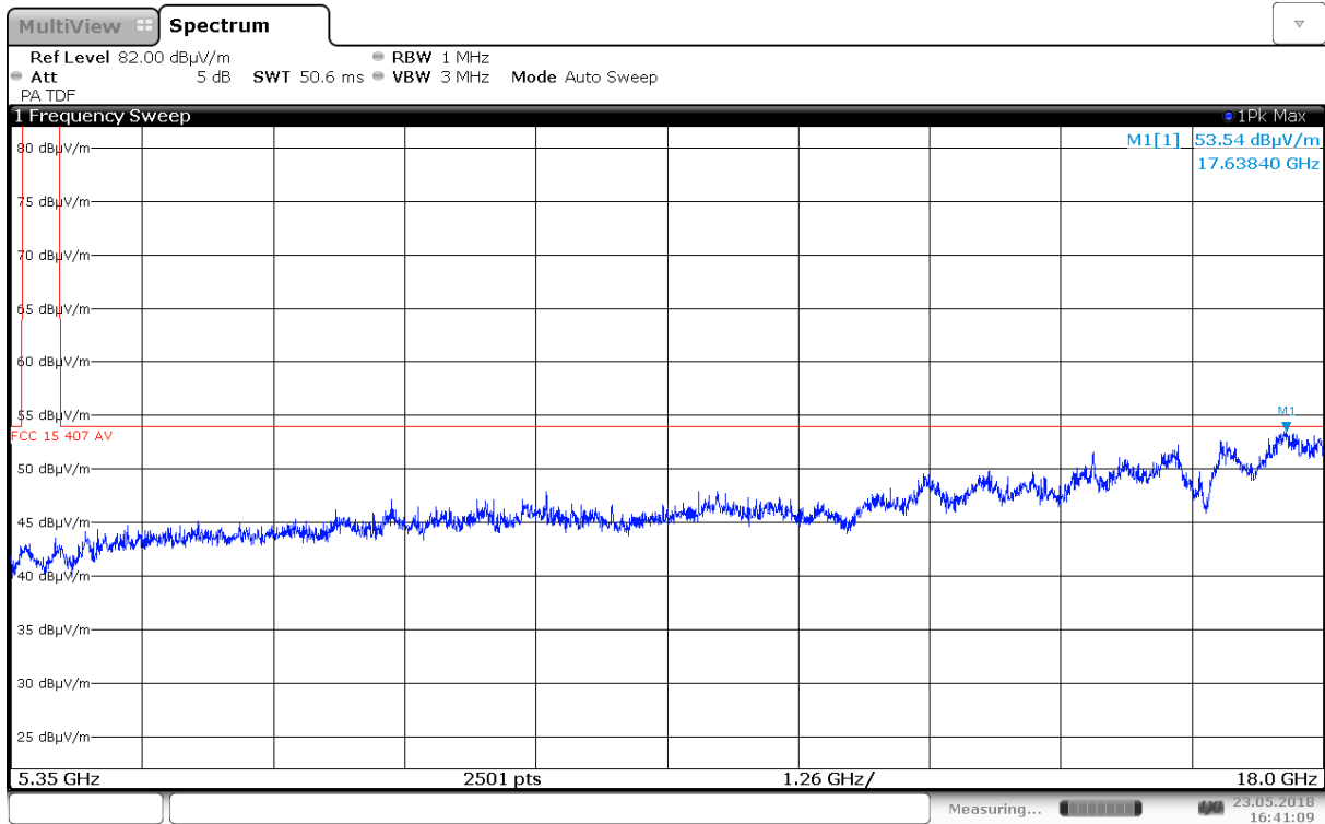
Radiated Emissions, 5350 – 18000 MHz, 5260 MHz, 802.11a 6M, Ant0, HP
