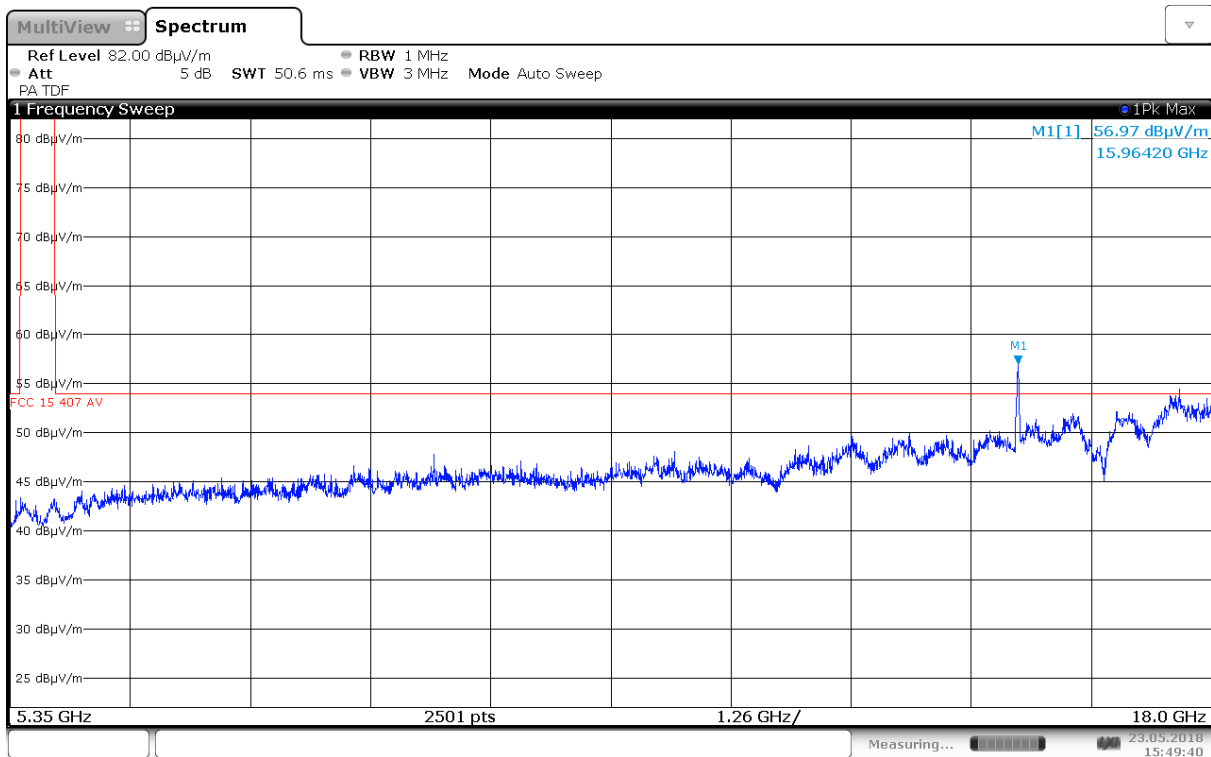
Radiated Emissions, 5350 – 18000 MHz, 5320 MHz, 802.11n HT20, MIMO, VP
