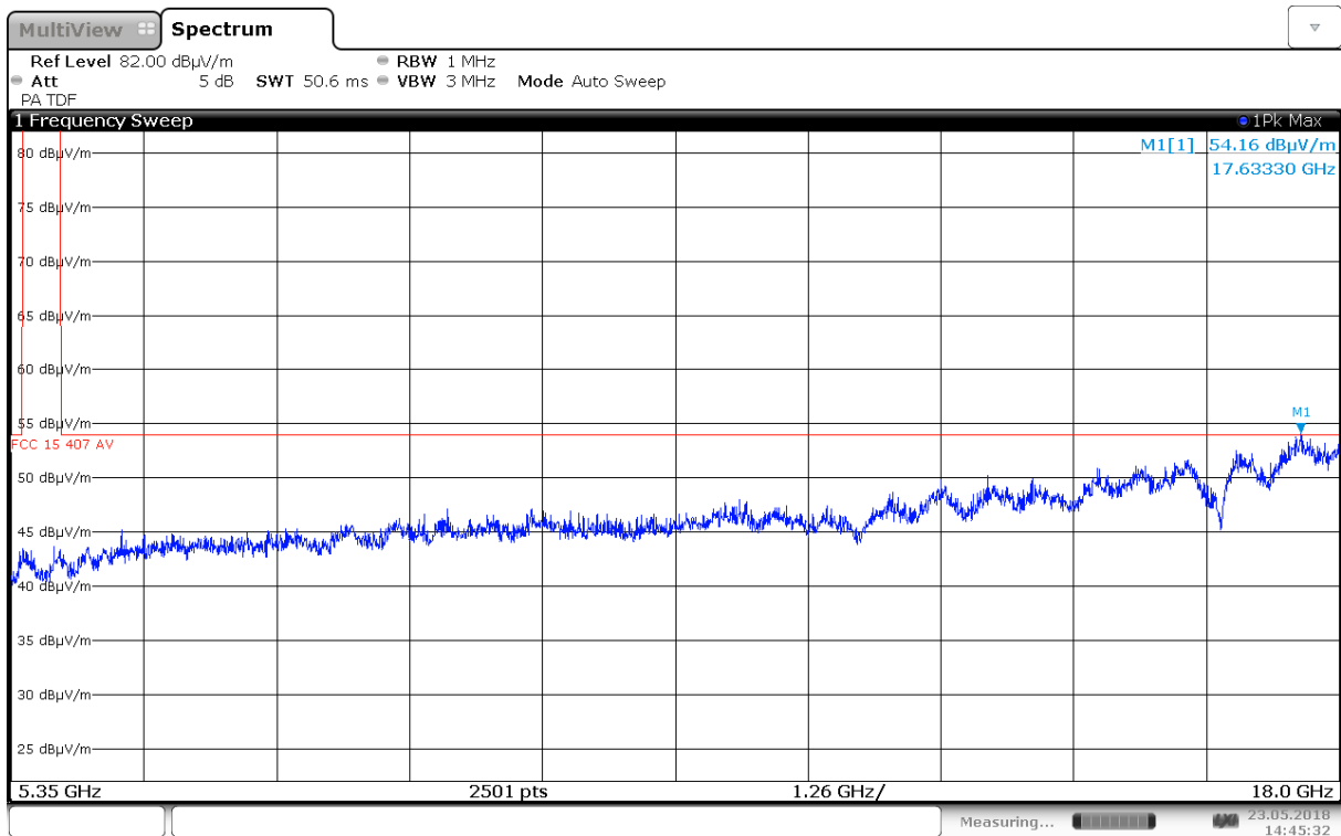
Radiated Emissions, 5350 – 18000 MHz, 5240 MHz, 802.11a 6M, Ant0, VP
