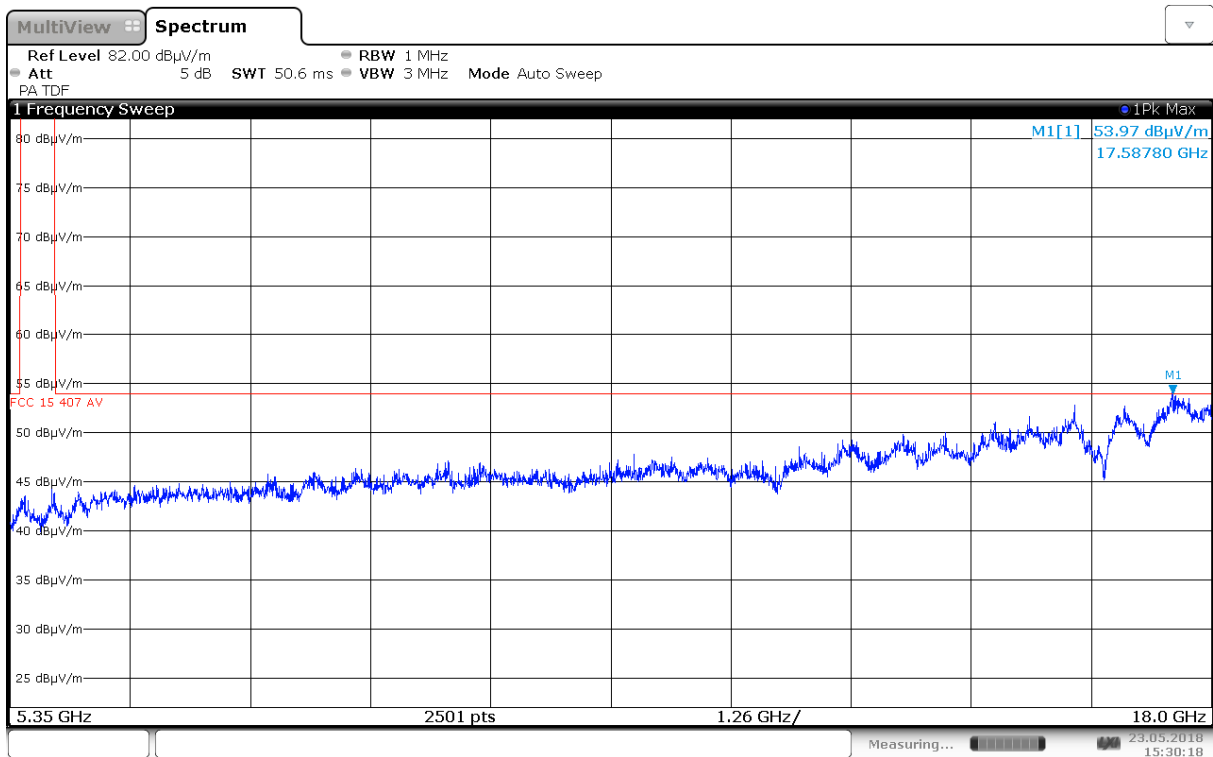
Radiated Emissions, 5350 – 18000 MHz, 5240 MHz, 802.11a 6M, Ant1, VP
