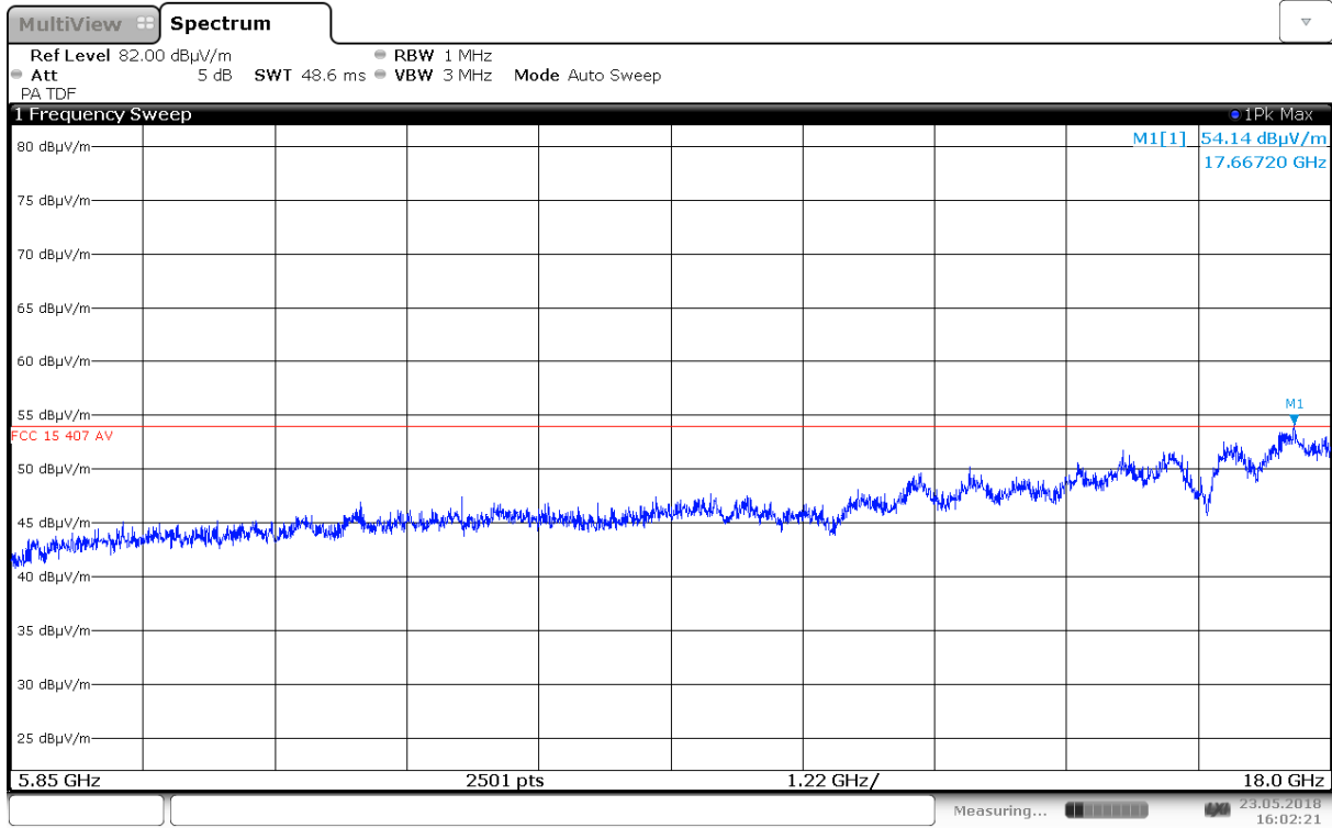
Radiated Emissions, 5850 – 18000 MHz, 5785 MHz, 802.11n HT20, MIMO, HP
