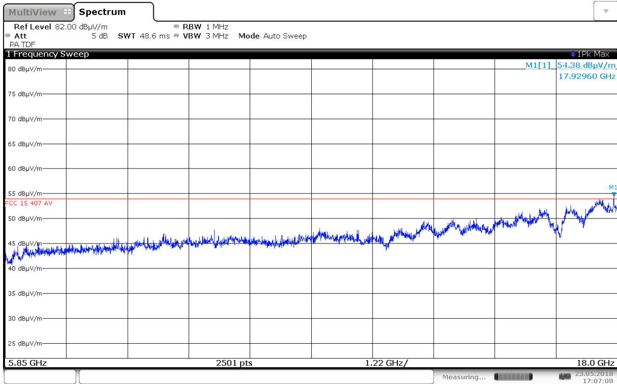
Radiated Emissions, 5850 – 18000 MHz, 5785 MHz, 802.11a 6M, Ant0, HP
