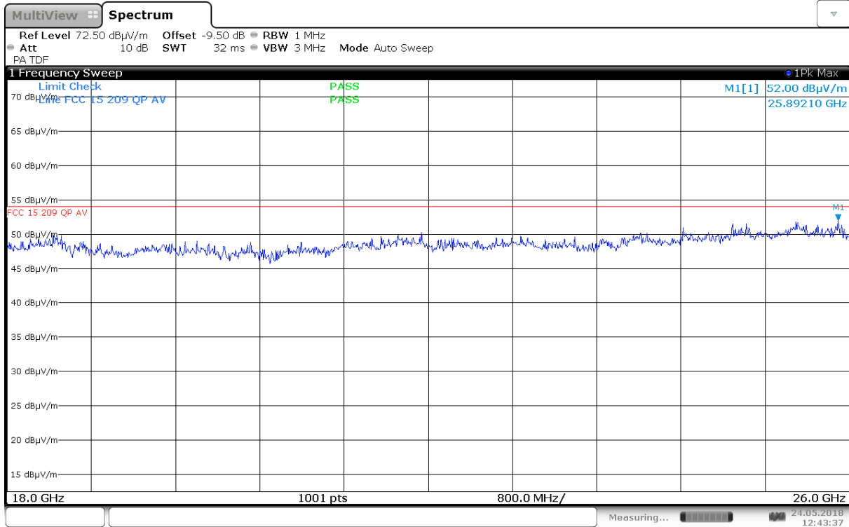
Radiated Emissions, 18.0 – 26.0GHz, 5580 MHz, 802.11a 6M, Ant 1, HP, @1m
