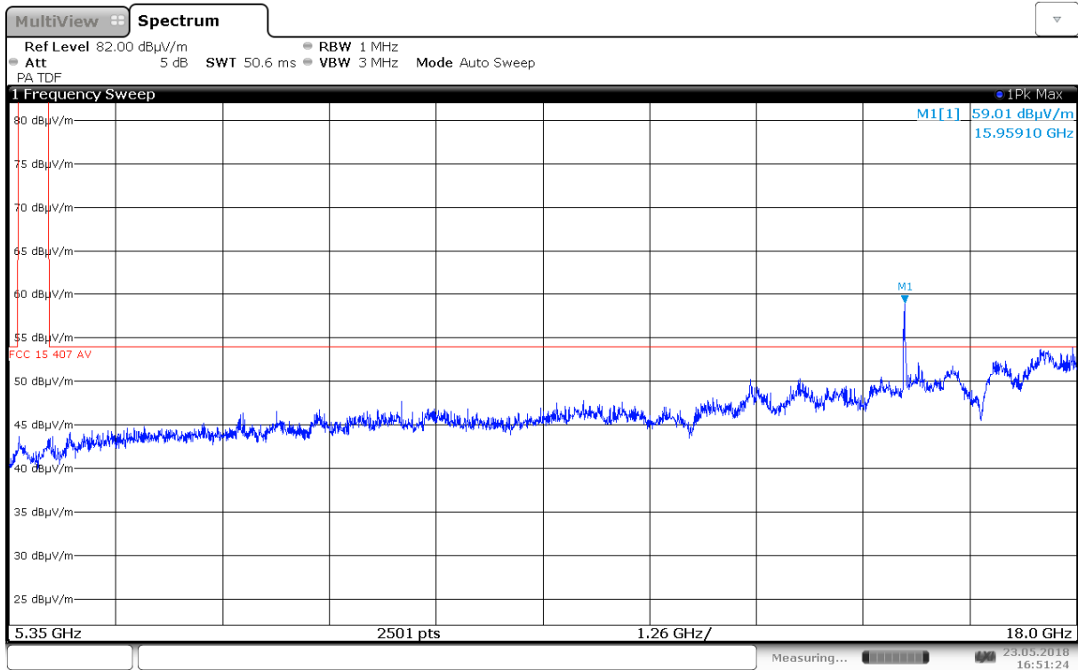
Radiated Emissions, 5350 – 18000 MHz, 5320 MHz, 802.11a 6M, Ant1, HP
