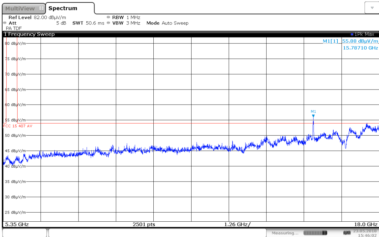
Radiated Emissions, 5350 – 18000 MHz, 5260 MHz, 802.11n HT20, MIMO, VP
