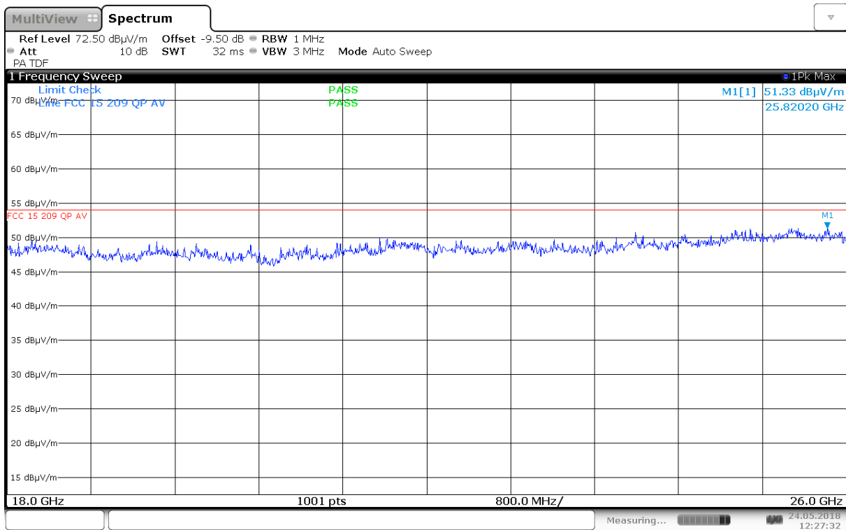
Radiated Emissions, 18.0 – 26.0GHz, 5300 MHz, 802.11n HT20, MIMO, VP, @1m
