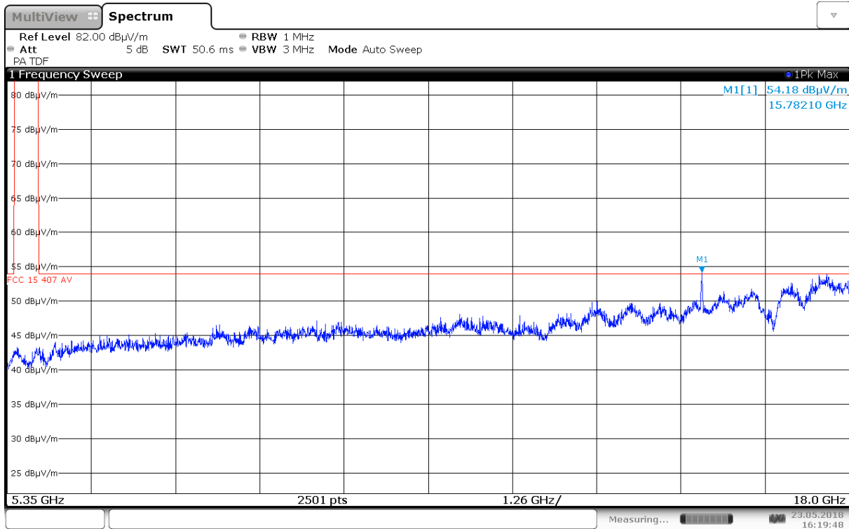
Radiated Emissions, 5350 – 18000 MHz, 5260 MHz, 802.11n HT20, MIMO, HP
