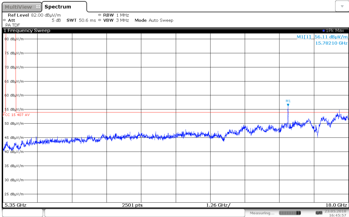
Radiated Emissions, 5350 – 18000 MHz, 5260 MHz, 802.11a 6M, Ant1, HP
