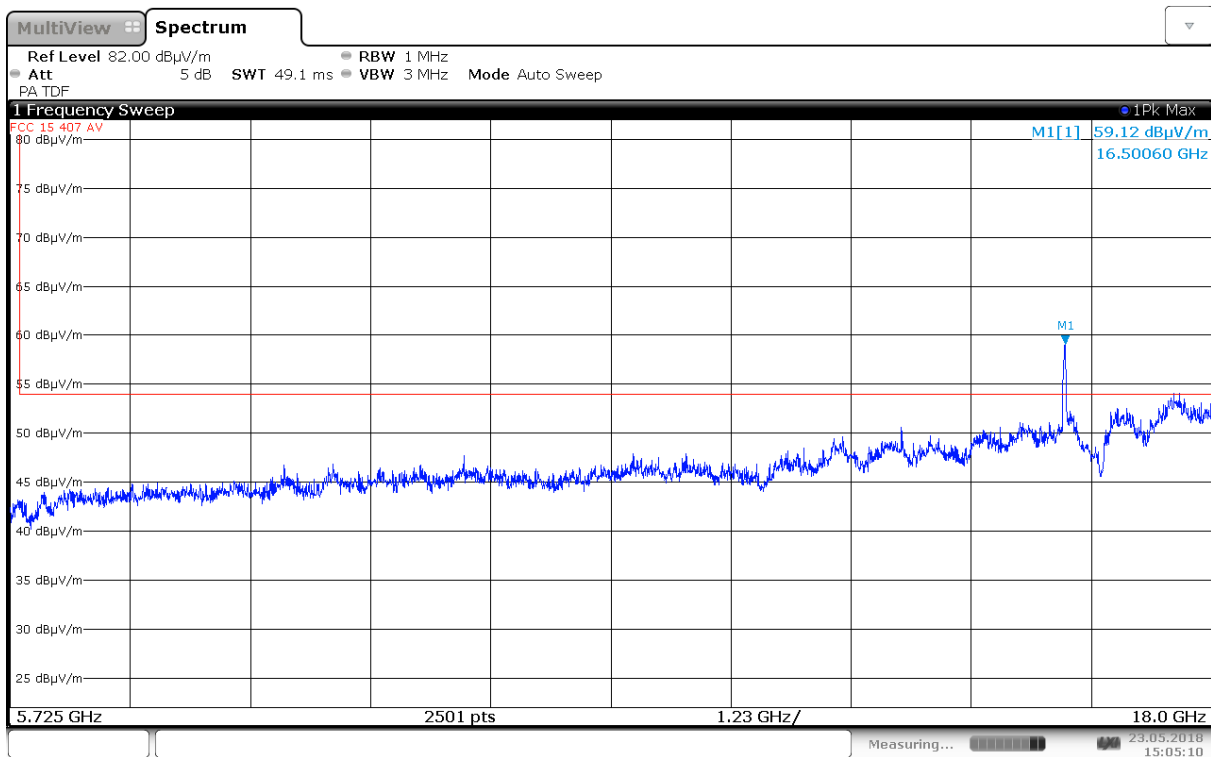
Radiated Emissions, 5725 – 18000 MHz, 5500 MHz, 802.11a 6M, Ant0, VP (Emission detected at 16.5 GHz is not in a Restricted Band)
