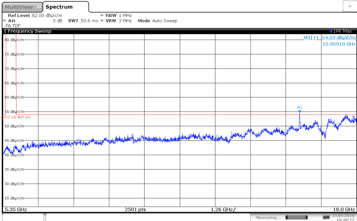
Radiated Emissions, 5350 – 18000 MHz, 5320 MHz, 802.11a 6M, Ant0, HP
