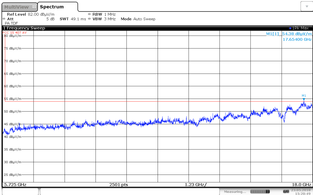
Radiated Emissions, 5725 – 18000 MHz, 5700 MHz, 802.11a 6M, Ant1, VP
