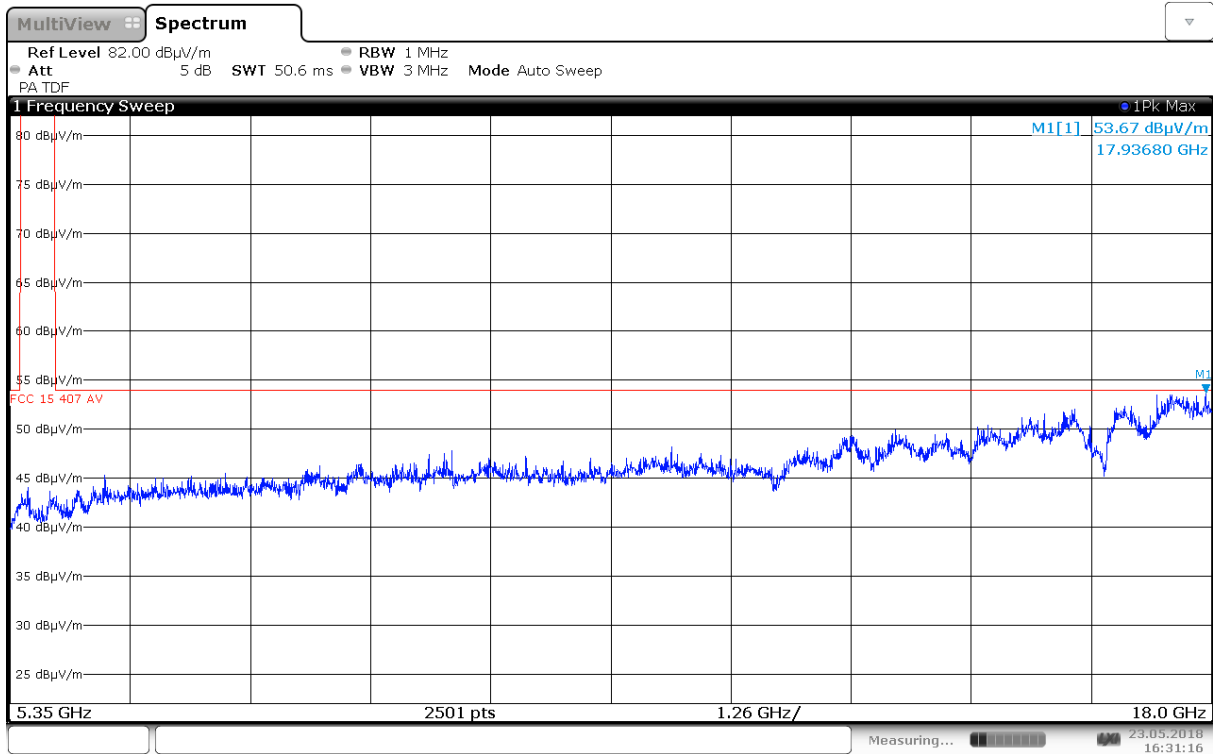
Radiated Emissions, 5350 – 18000 MHz, 5180 MHz, 802.11a 6M, Ant1, HP
