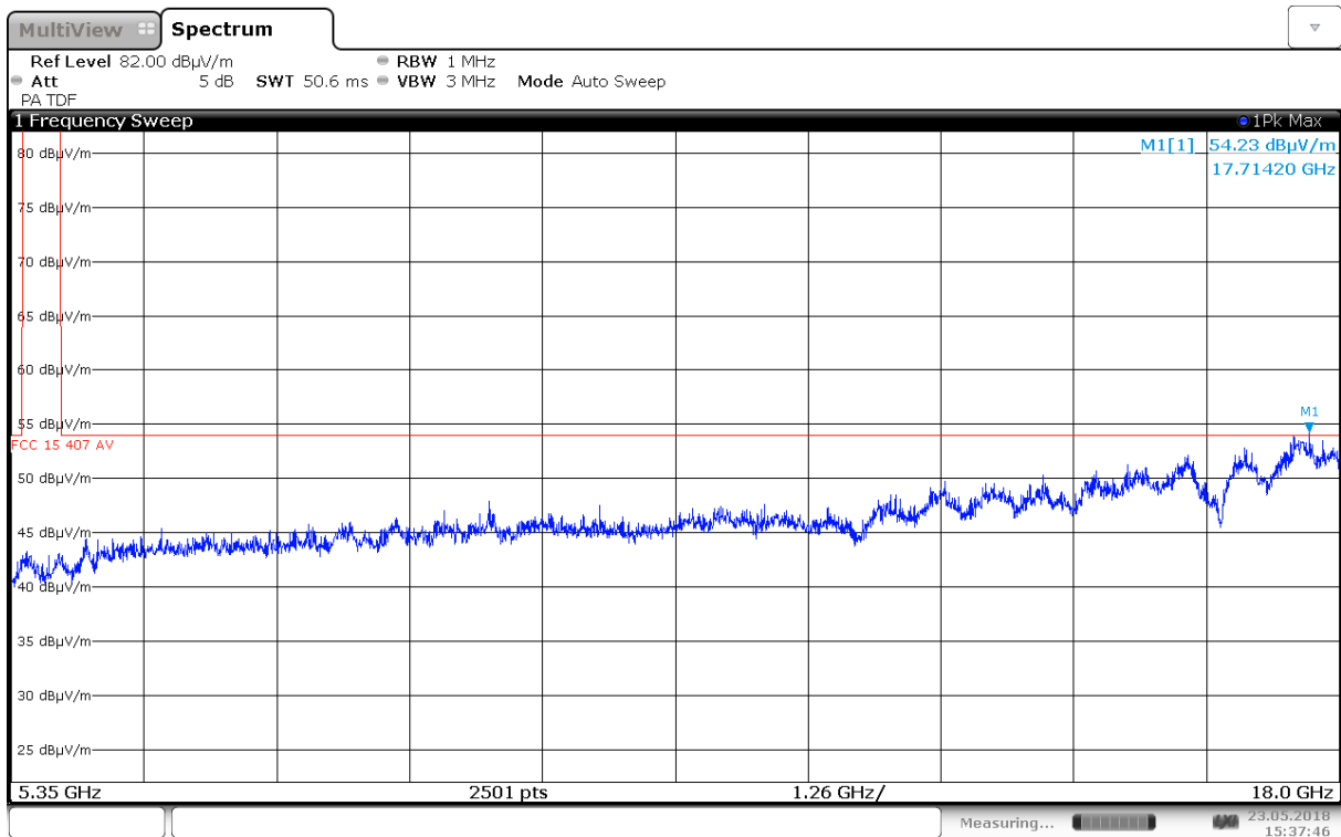
Radiated Emissions, 5350 – 18000 MHz, 5180 MHz, 802.11n HT20, MIMO, VP
