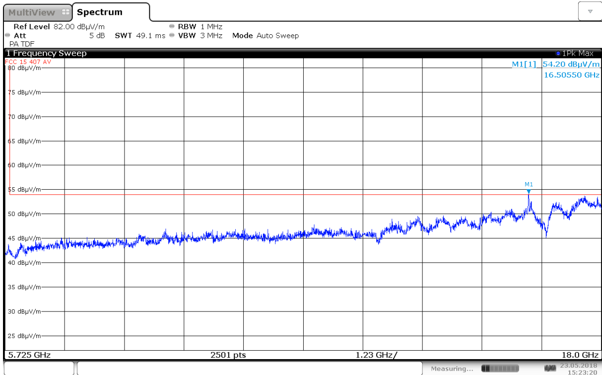
Radiated Emissions, 5725 – 18000 MHz, 5500 MHz, 802.11a 6M, Ant1, VP (Emission detected at 16.5 GHz is not in a Restricted Band)
