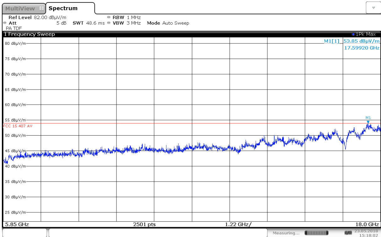
Radiated Emissions, 5850 – 18000 MHz, 5785 MHz, 802.11a 6M, Ant1, VP
