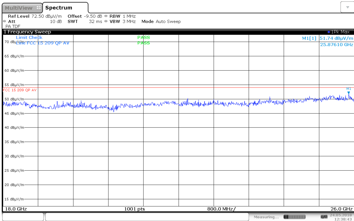
Radiated Emissions, 18.0 – 26.0GHz, 5580 MHz, 802.11a 6M, Ant 0, VP, @1m
