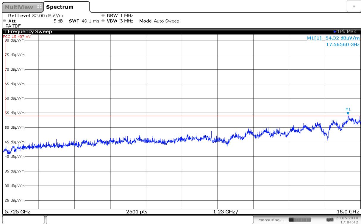
Radiated Emissions, 5725 – 18000 MHz, 5700 MHz, 802.11a 6M, Ant1, HP
