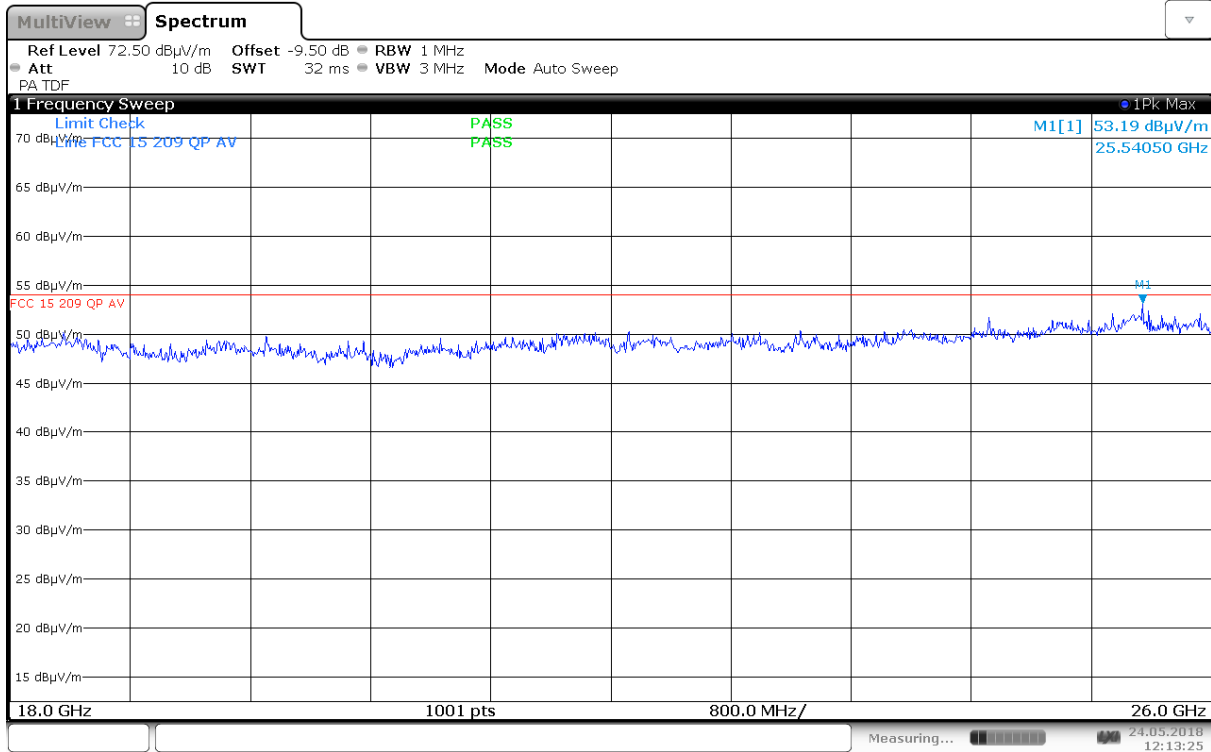
Radiated Emissions, 18.0 – 26.0GHz, 5300 MHz, 802.11a 6M, Ant 0, HP, @1m
