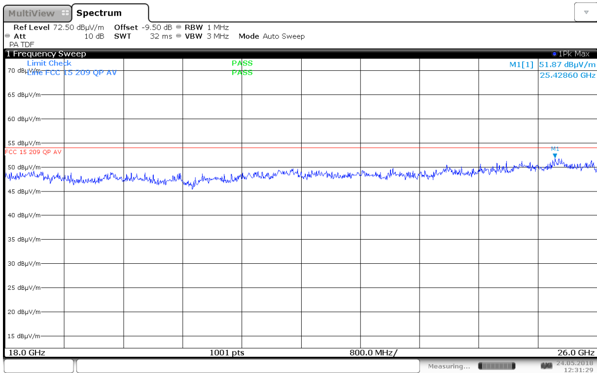
Radiated Emissions, 18.0 – 26.0GHz, 5580 MHz, 802.11n HT20, MIMO, VP, @1m
