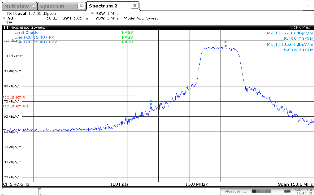
Unwanted Emissions, Band Edge, 5470MHz, ch100, 802.11n MCS0 HT20, MIMO
