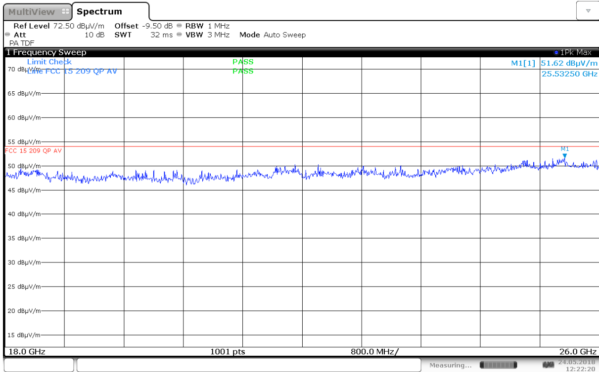
Radiated Emissions, 18.0 – 26.0GHz, 5300 MHz, 802.11a 6M, Ant 1, HP, @1m
