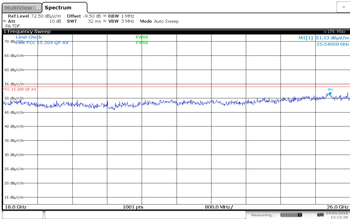
Radiated Emissions, 18.0 – 26.0GHz, 5300 MHz, 802.11a 6M, Ant 0, VP, @1m
