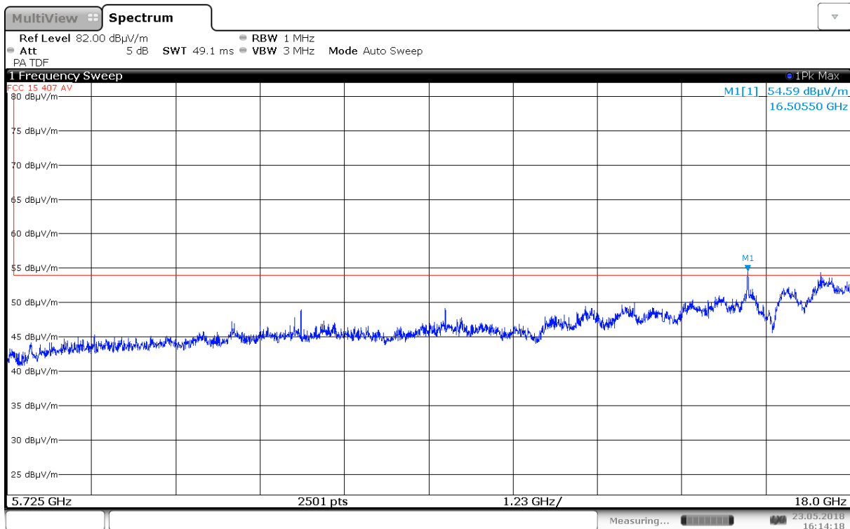
Radiated Emissions, 5725 – 18000 MHz, 5500 MHz, 802.11n HT20, MIMO, HP (Emission detected at 16.5 GHz is not in a Restricted Band)
