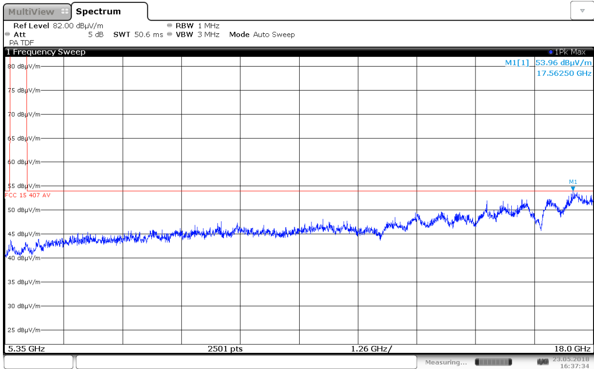
Radiated Emissions, 5350 – 18000 MHz, 5240 MHz, 802.11a 6M, Ant1, HP
