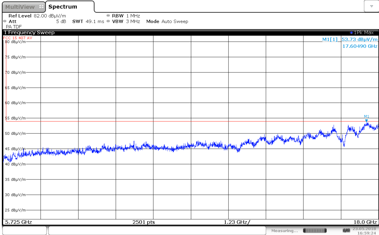
Radiated Emissions, 5725 – 18000 MHz, 5500 MHz, 802.11a 6M, Ant1, HP
