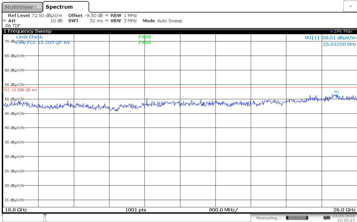
Radiated Emissions, 18.0 – 26.0GHz, 5300 MHz, 802.11n HT20, MIMO, HP, @1m
