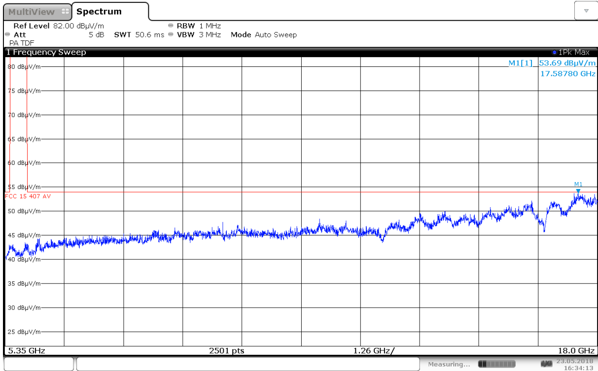
Radiated Emissions, 5350 – 18000 MHz, 5240 MHz, 802.11a 6M, Ant0, HP
