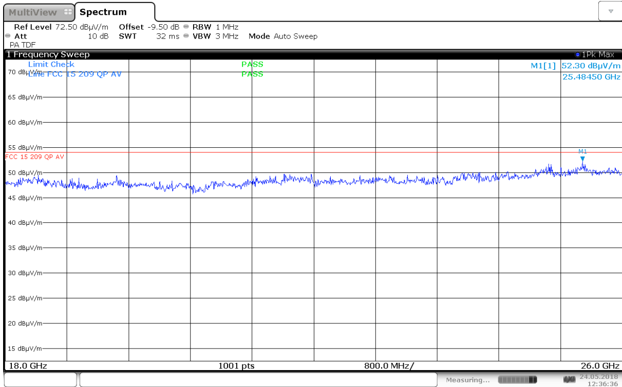
Radiated Emissions, 18.0 – 26.0GHz, 5580 MHz, 802.11a 6M, Ant 0, HP, @1m
