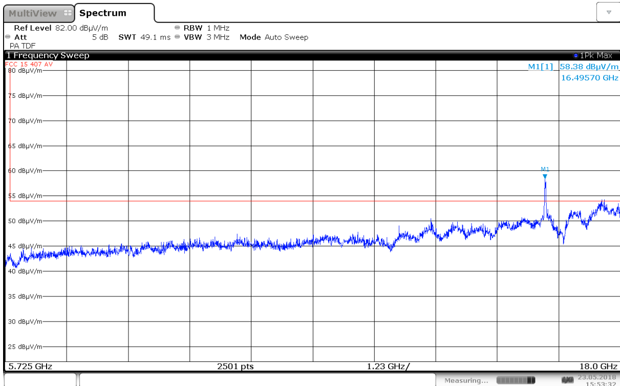
Radiated Emissions, 5725 – 18000 MHz, 5500 MHz, 802.11n HT20, MIMO, VP (Emission detected at 16.5 GHz is not in a Restricted Band)
