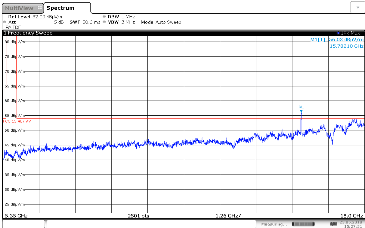
Radiated Emissions, 5350 – 18000 MHz, 5260 MHz, 802.11a 6M, Ant1, VP
