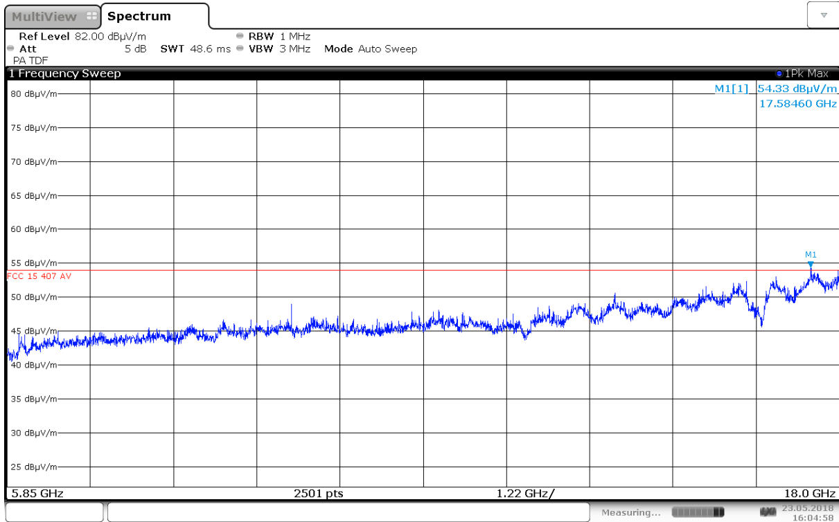
Radiated Emissions, 5850 – 18000 MHz, 5700 MHz, 802.11n HT20, MIMO, HP
