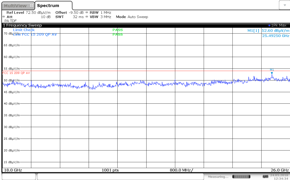
Radiated Emissions, 18.0 – 26.0GHz, 5580 MHz, 802.11n HT20, MIMO, HP, @1m
