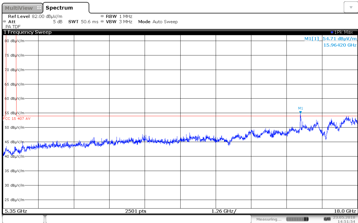
Radiated Emissions, 5350 – 18000 MHz, 5320 MHz, 802.11a 6M, Ant0, VP
