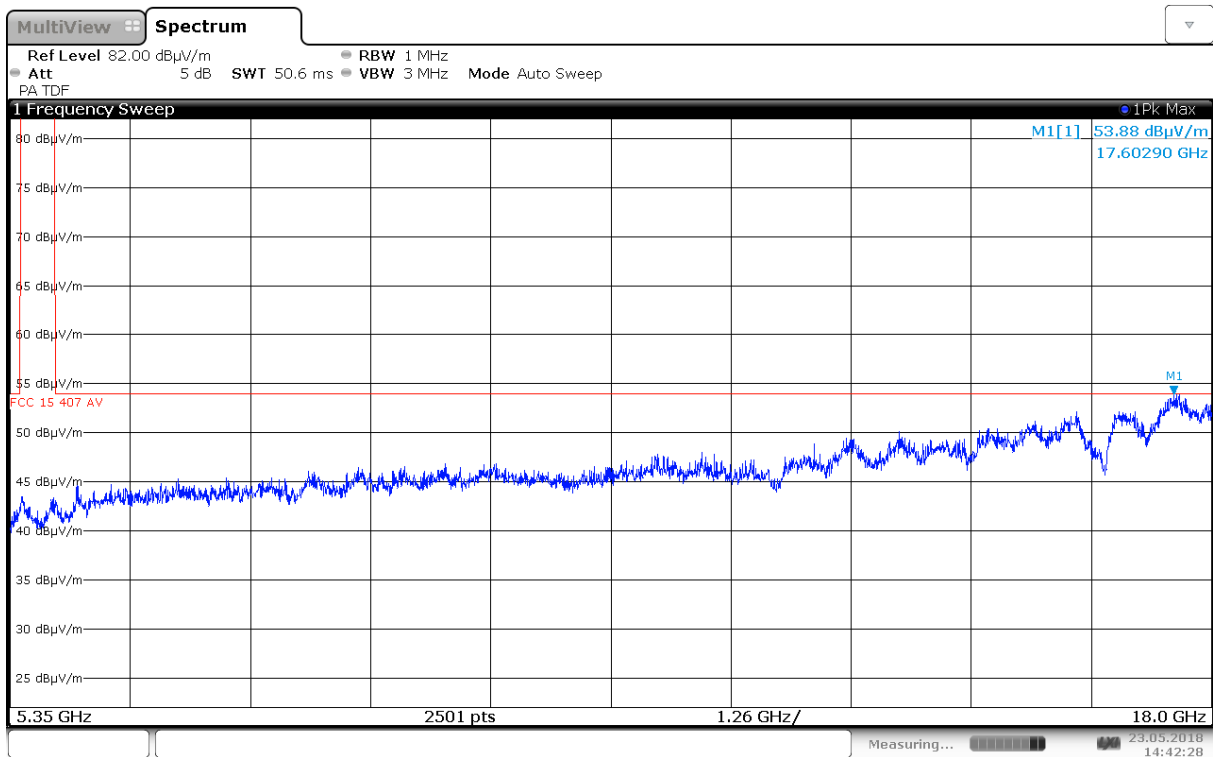
Radiated Emissions, 5350 – 18000 MHz, 5180 MHz, 802.11a 6M, Ant0, VP
