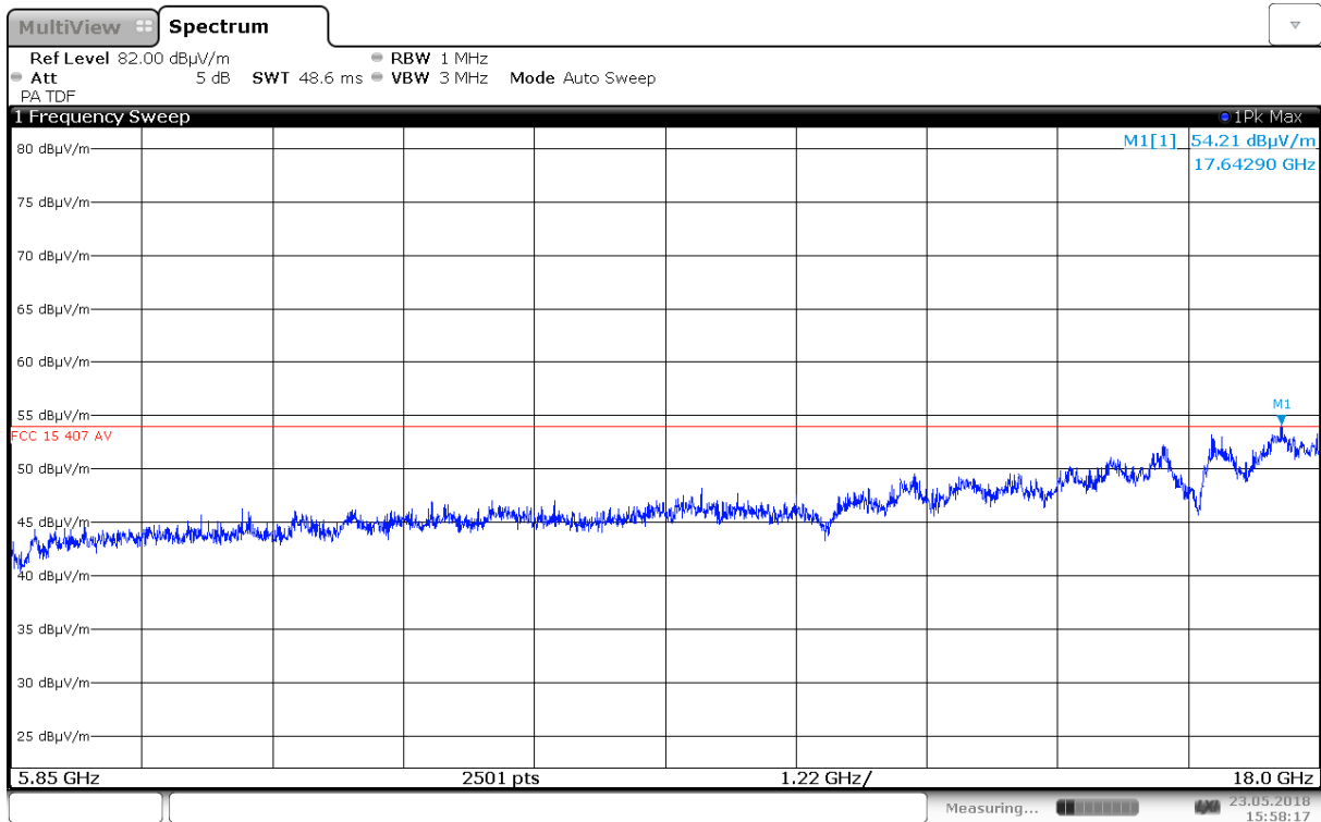
Radiated Emissions, 5850 – 18000 MHz, 5785 MHz, 802.11n HT20, MIMO, VP
