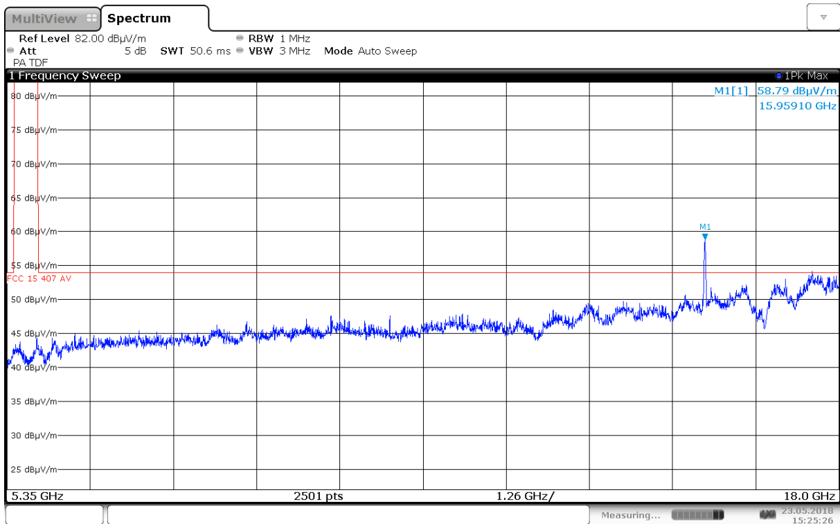
Radiated Emissions, 5350 – 18000 MHz, 5320 MHz, 802.11a 6M, Ant1, VP
