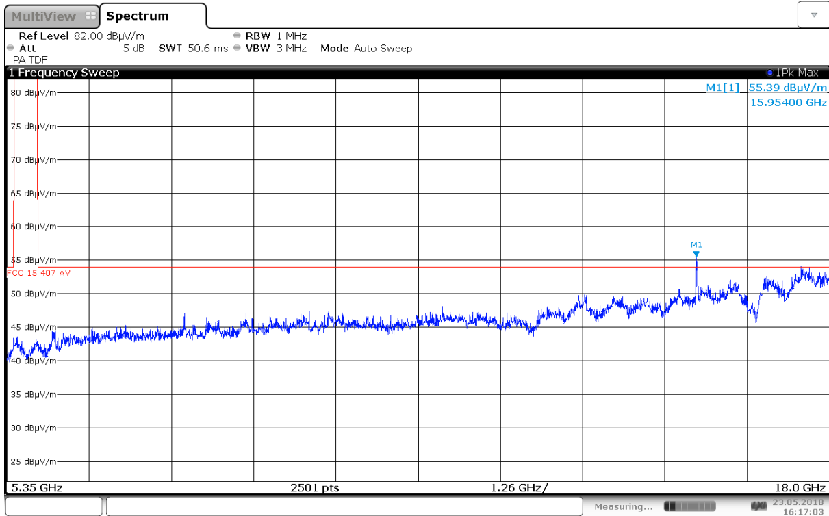
Radiated Emissions, 5350 – 18000 MHz, 5320 MHz, 802.11n HT20, MIMO, HP
