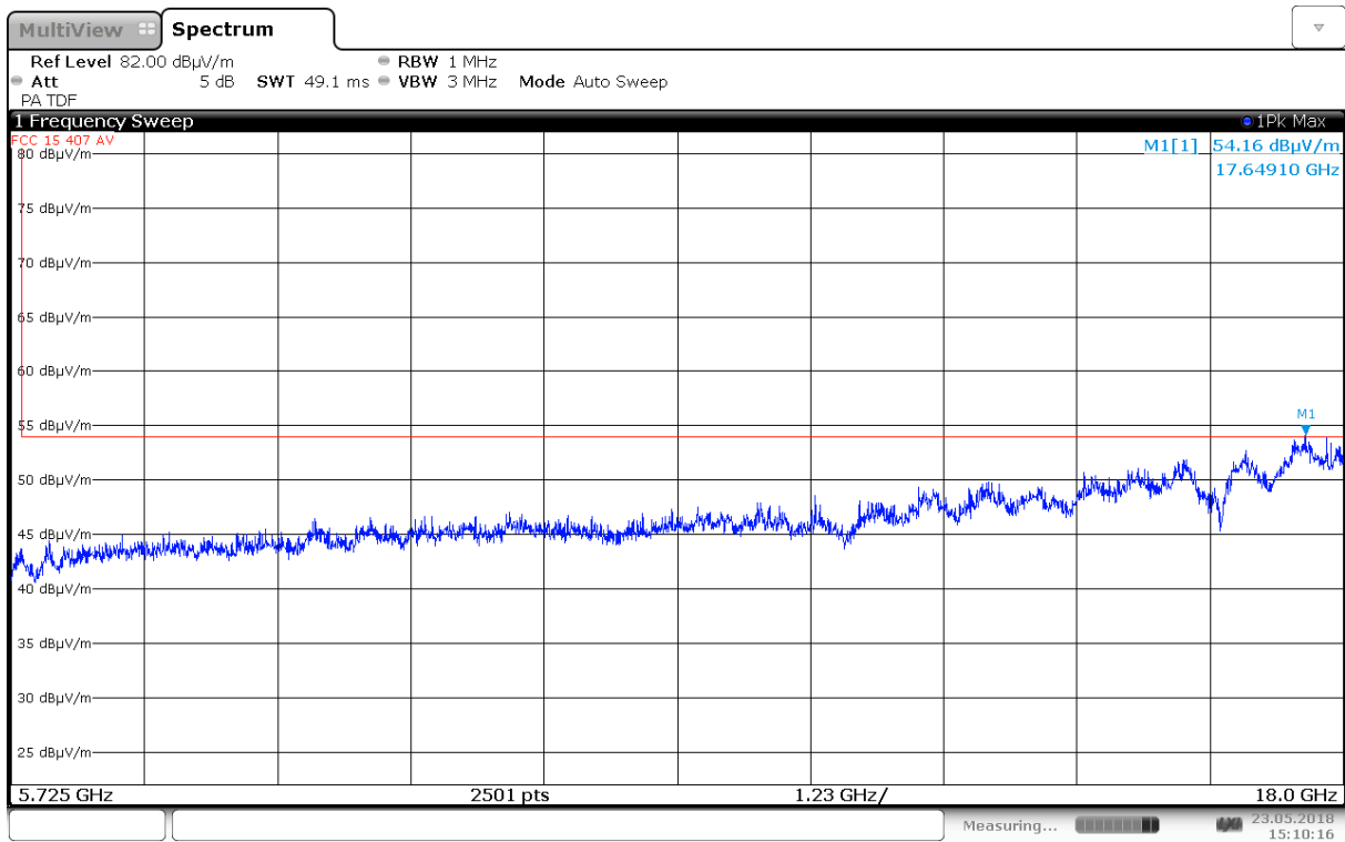
Radiated Emissions, 5725 – 18000 MHz, 5700 MHz, 802.11a 6M, Ant0, VP
