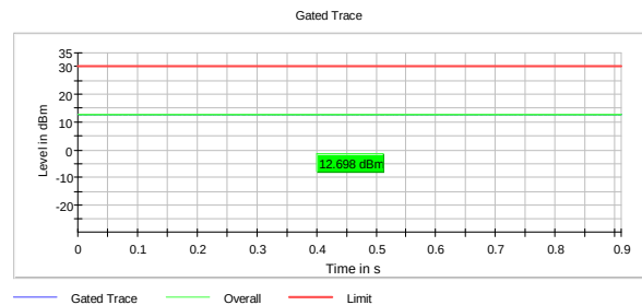
Output Power, 2437 MHz, 802.11ax MCS0, MIMO
