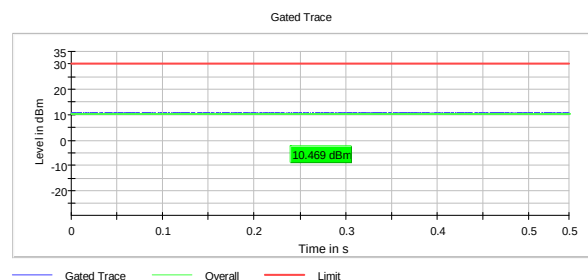
Output Power, 2462 MHz, 802.11ax MCS11, MIMO
