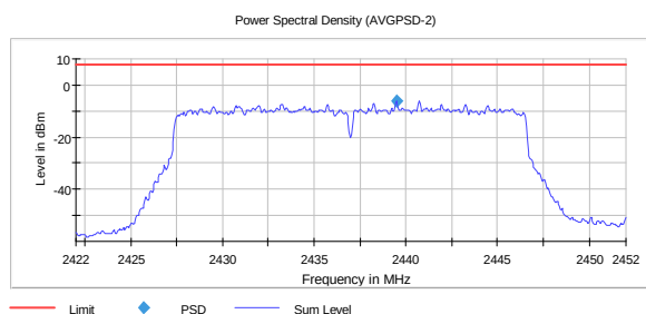
PSD, 2437 MHz, 802.11ax MCS11 SISO -6.1
