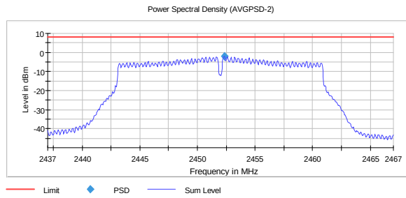
PSD, 2452 MHz, 802.11n MCS0 SISO -2.0
