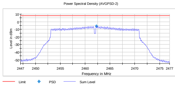
PSD, 2462 MHz, 802.11n MCS0 SISO -6.0
