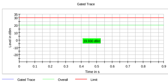
Output Power, 2442 MHz, 802.11g 6M
