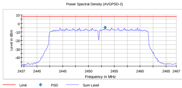
PSD, 2452 MHz, 802.11ax MCS8 SISO -4.8
