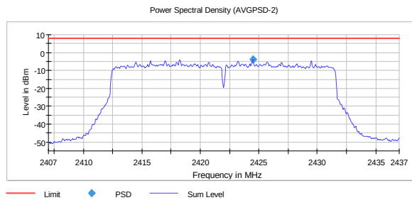
PSD, 2422 MHz, 802.11ax MCS8 SISO -3.8
