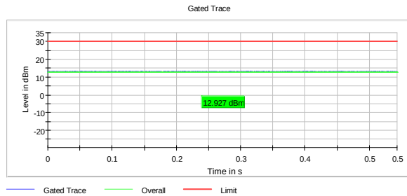
Output Power, 2422 MHz, 802.11ax MCS11
