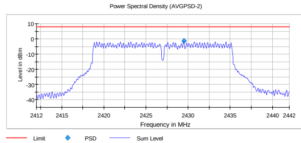
PSD, 2427 MHz, 802.11g 54M -1.2
