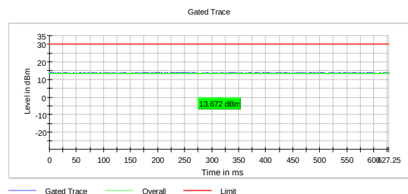
Output Power, 2462 MHz, 802.11n MCS7
