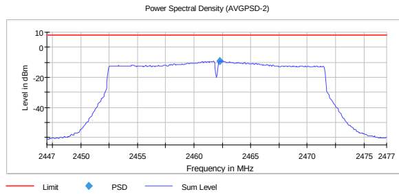
PSD, 2462 MHz, 802.11ax MCS0 SISO -9.3
