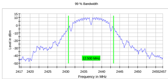
99% Occupied BW, 802.11b 1M
