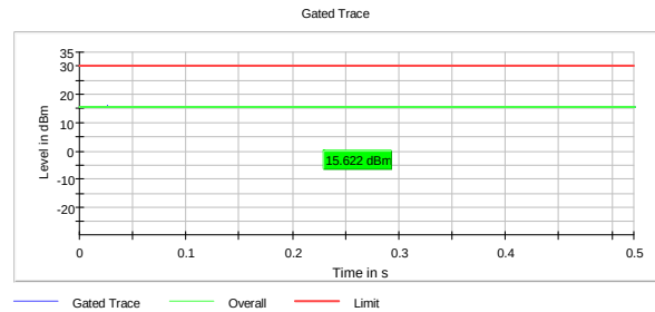
Output Power, 2422 MHz, 802.11n MCS15, MIMO
