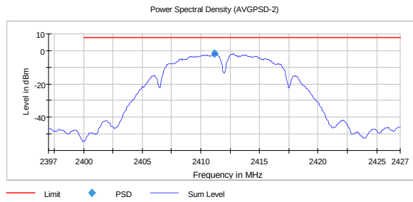
PSD, 2412 MHz, 802.11b 1M -1.9
