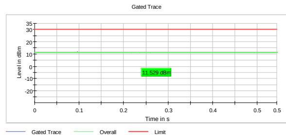
Output Power, 2437 MHz, 802.11ax MCS11, MIMO
