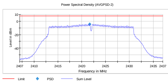
PSD, 2422 MHz, 802.11n MCS8 MIMO -4.4
