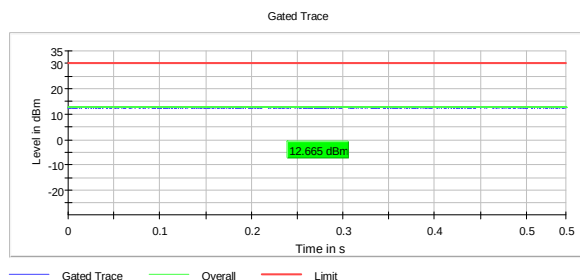
Output Power, 2452 MHz, 802.11ax MCS11
