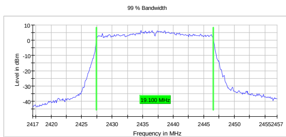
99% Occupied BW, 802.11ax MCS0, SISO
