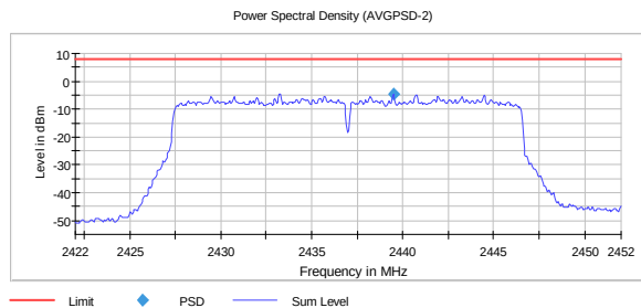
PSD, 2437 MHz, 802.11ax MCS8 SISO -4.6
