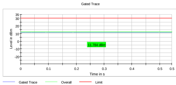
Output Power, 2412 MHz, 802.11ax MCS11
