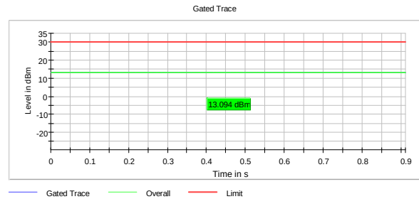
Output Power, 2422 MHz, 802.11ax MCS0, MIMO
