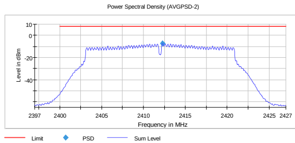
PSD, 2412 MHz, 802.11n MCS8 MIMO -7.4
