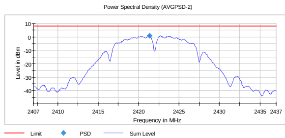
PSD, 2422 MHz, 802.11b 1M 1.1
