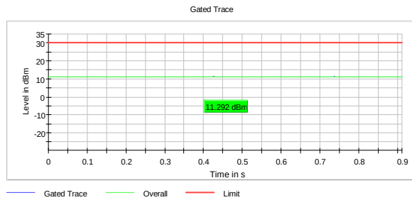
Output Power, 2412 MHz, 802.11ax MCS0
