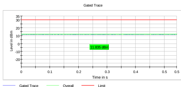
Output Power, 2462 MHz, 802.11ax MCS11
