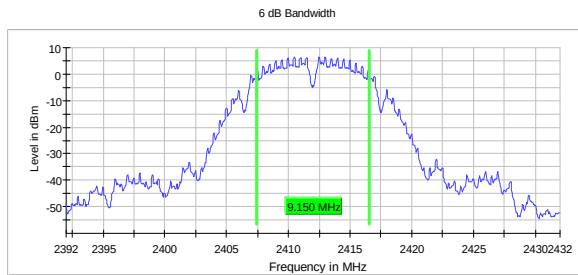
DTS BW, 2412 MHz, 802.11b 1M
