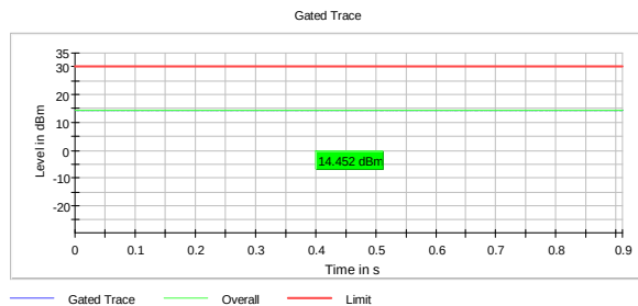
Output Power, 2437 MHz, 802.11ax MCS0
