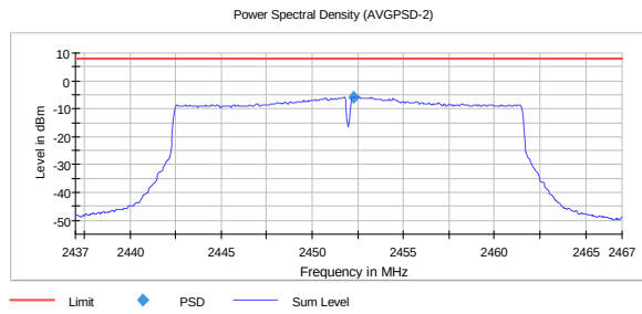
PSD, 2452 MHz, 802.11ax MCS0 SISO -5.7
