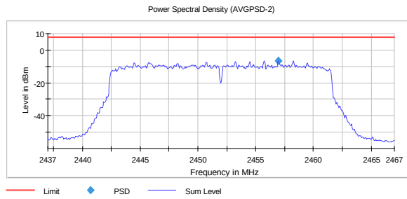
PSD, 2452 MHz, 802.11ax MCS11 SISO -6.6
