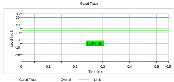
Output Power, 2422 MHz, 802.11ax MCS11, MIMO
