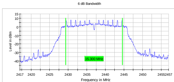
DTS BW, 2437 MHz, 802.11n MCS0, SISO
