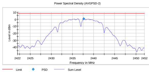
PSD, 2437 MHz, 802.11b 1M 0.6
