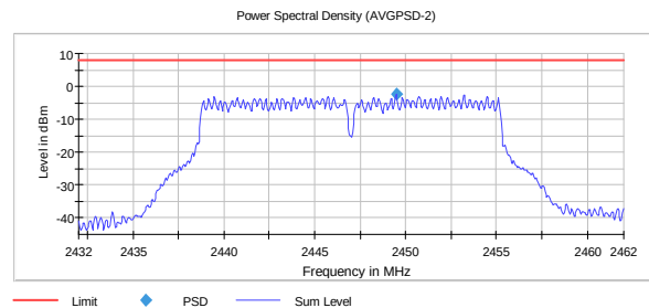
PSD, 2447 MHz, 802.11g 54M -2.4
