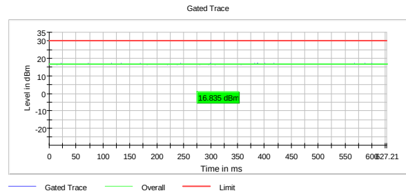
Output Power, 2437 MHz, 802.11n MCS7
