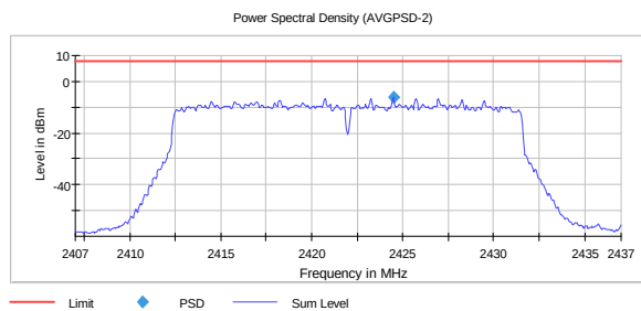
PSD, 2422 MHz, 802.11ax MCS11 SISO -6.3
