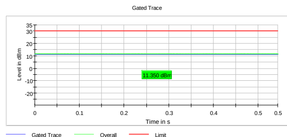
Output Power, 2452 MHz, 802.11ax MCS11, MIMO
