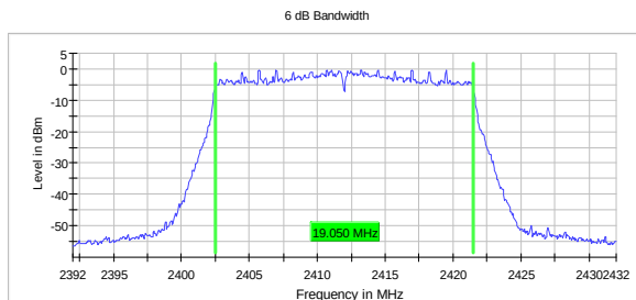
DTS BW, 2412 MHz, 802.11ax MCS0, SISO
