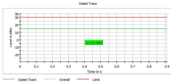
Output Power, 2422 MHz, 802.11ax MCS0
