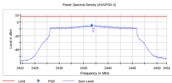
PSD, 2437 MHz, 802.11n MCS8 MIMO -4.8
