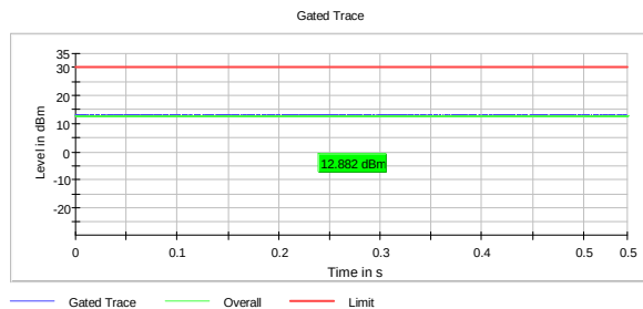
Output Power, 2437 MHz, 802.11ax MCS11
