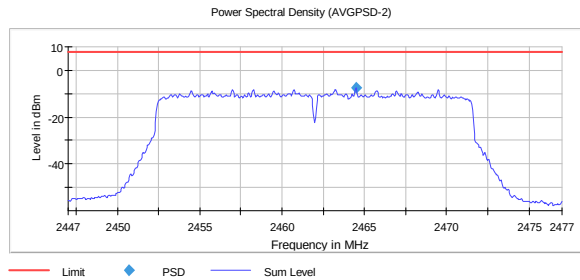
PSD, 2462 MHz, 802.11ax MCS8 SISO -7.4
