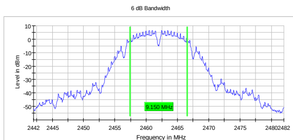
DTS BW, 2462 MHz, 802.11b 1M
