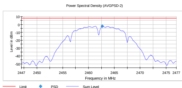
PSD, 2462 MHz, 802.11b 1M -2.0
