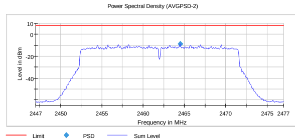
PSD, 2462 MHz, 802.11ax MCS8 MIMO -8.7
