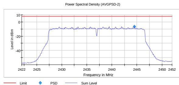
PSD, 2437 MHz, 802.11ax MCS8 MIMO -6.5
