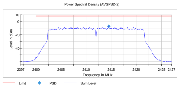
PSD, 2412 MHz, 802.11ax MCS8 SISO -7.3
