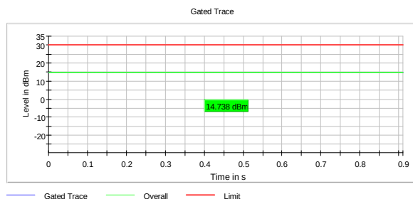
Output Power, 2452 MHz, 802.11ax MCS0
