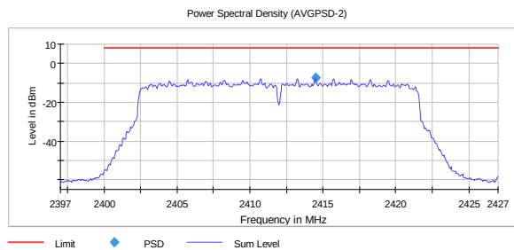
PSD, 2412 MHz, 802.11ax MCS11 SISO -7.4
