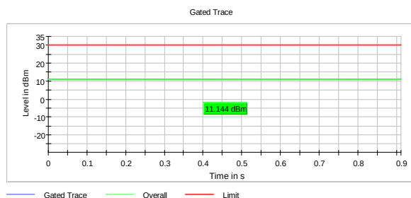
Output Power, 2462 MHz, 802.11ax MCS0
