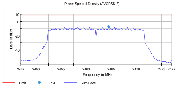
PSD, 2462 MHz, 802.11ax MCS11 SISO -7.5
