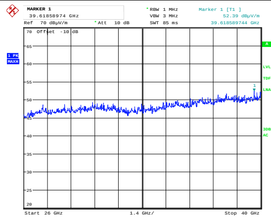
Radiated Emissions 26-40 GHz, Ch45, 802.11ax HT20 Ant1, 10cm
