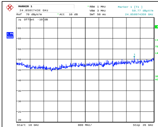
Radiated Emissions 18-26 GHz, Ch45, 802.11ax HT20 Ant1, 10cm
