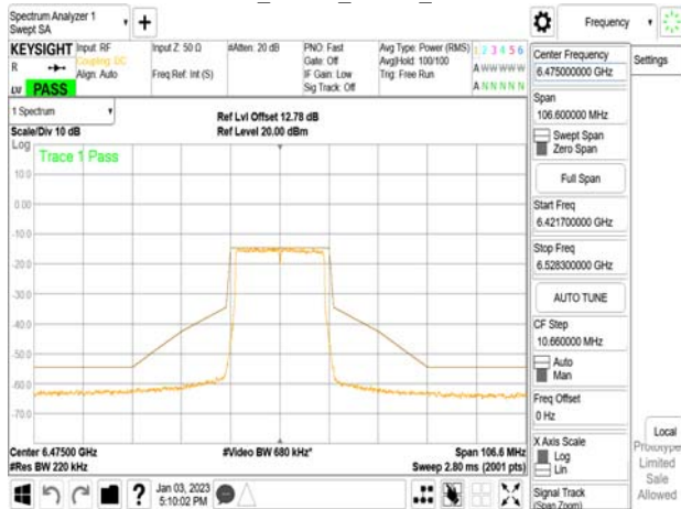
802.11ax_20MHz_Chain1_6475MHz
