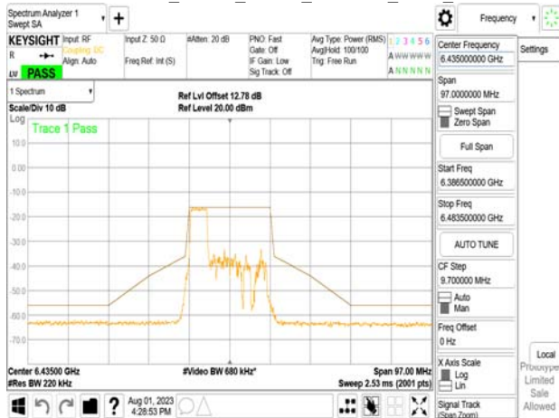
802.11ax_20MHz_Chain1_6435MHz_RU106_53
