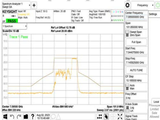
802.11ax_20MHz_Chain0_7095MHz_RU106_54
