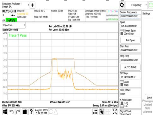
802.11ax_20MHz_Chain0_6895MHz_RU106_53
