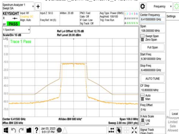
802.11ax_20MHz_Chain0_6415MHz_RU26_8
