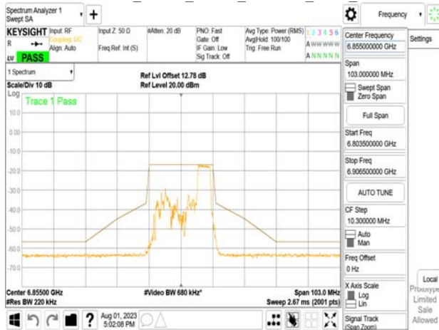
802.11ax_20MHz_Chain0_6855MHz_RU106_54
