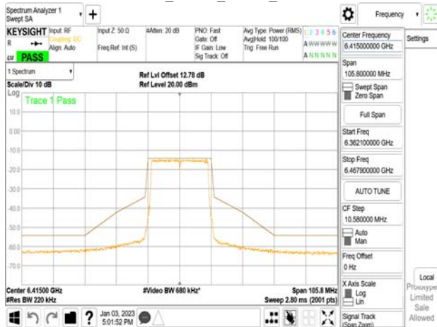
802.11ax_20MHz_Chain1_6415MHz_RU26_8
