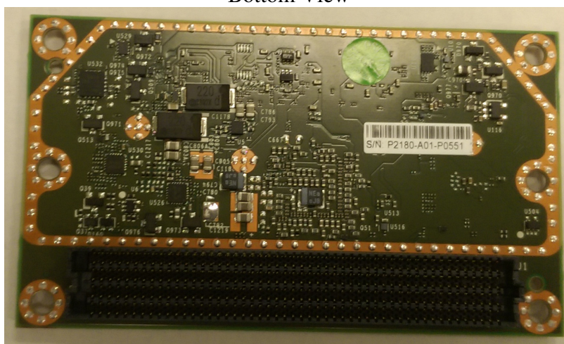
Bottom View
