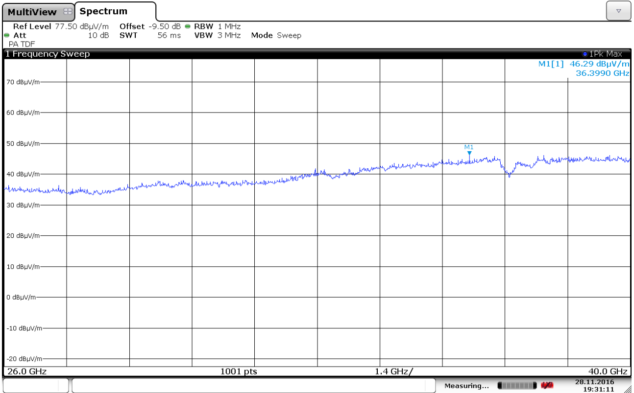
Radiated Emissions, 26.0 – 40.0 GHz, 5660 MHz, 802.11a 6M, Ant 1, HP
