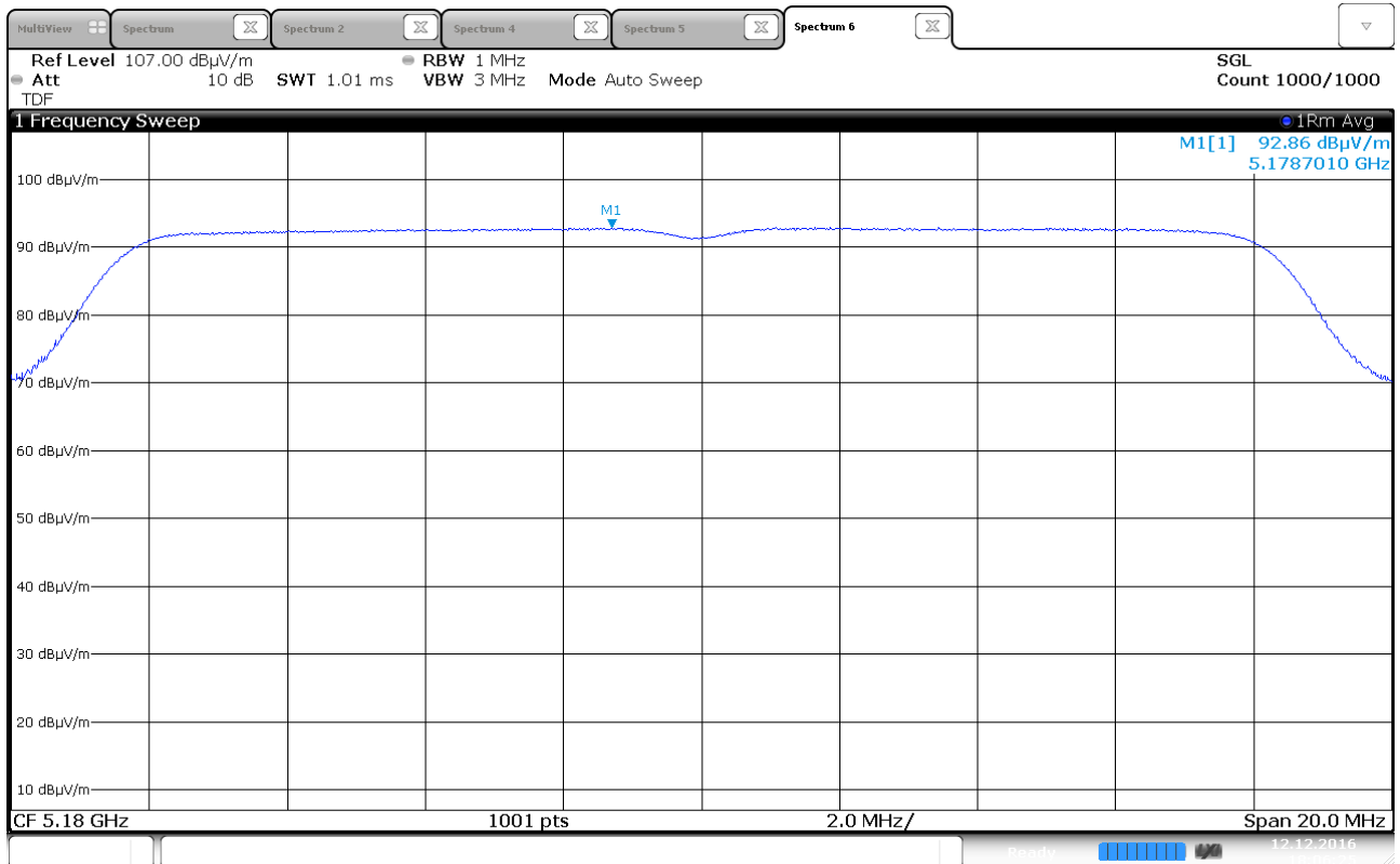
Power Spectral Density, 5180 MHz, 802.11a 6Mbps, Ant 0
