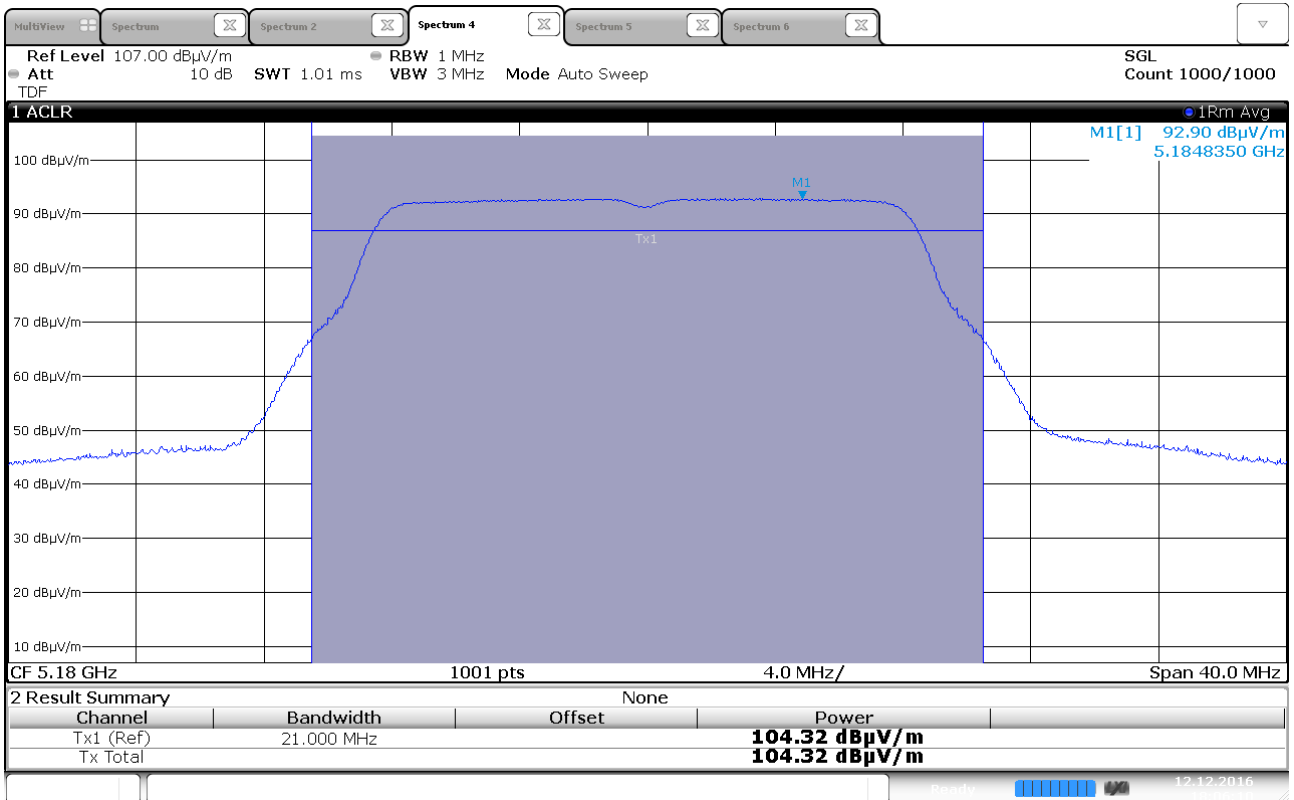
Maximum EIRP, 5180 MHz, 802.11a 6Mbps, Ant 0
