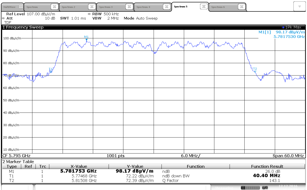
Emission Bandwidth B, 5795 MHz, 802.11n HT40, MIMO
