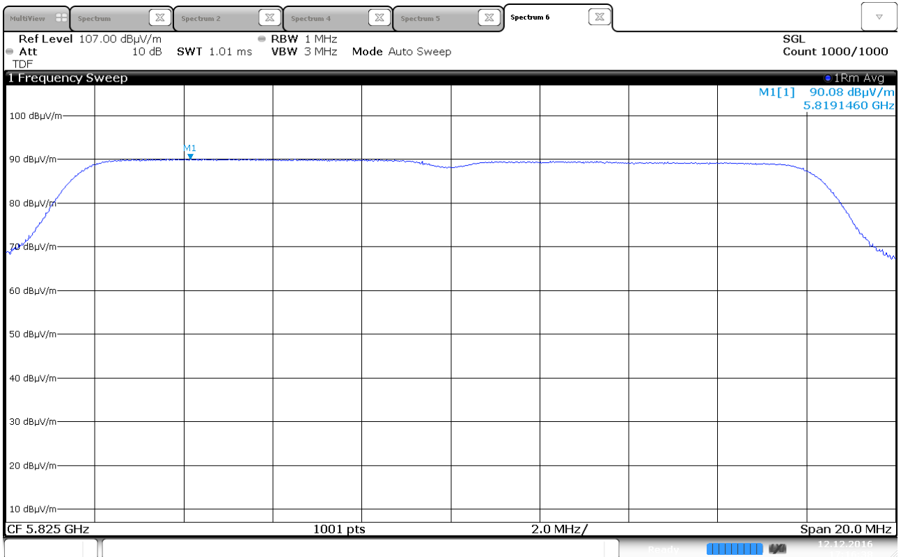
Power Spectral Density, 5825 MHz, 802.11a 6Mbps, Ant 0
