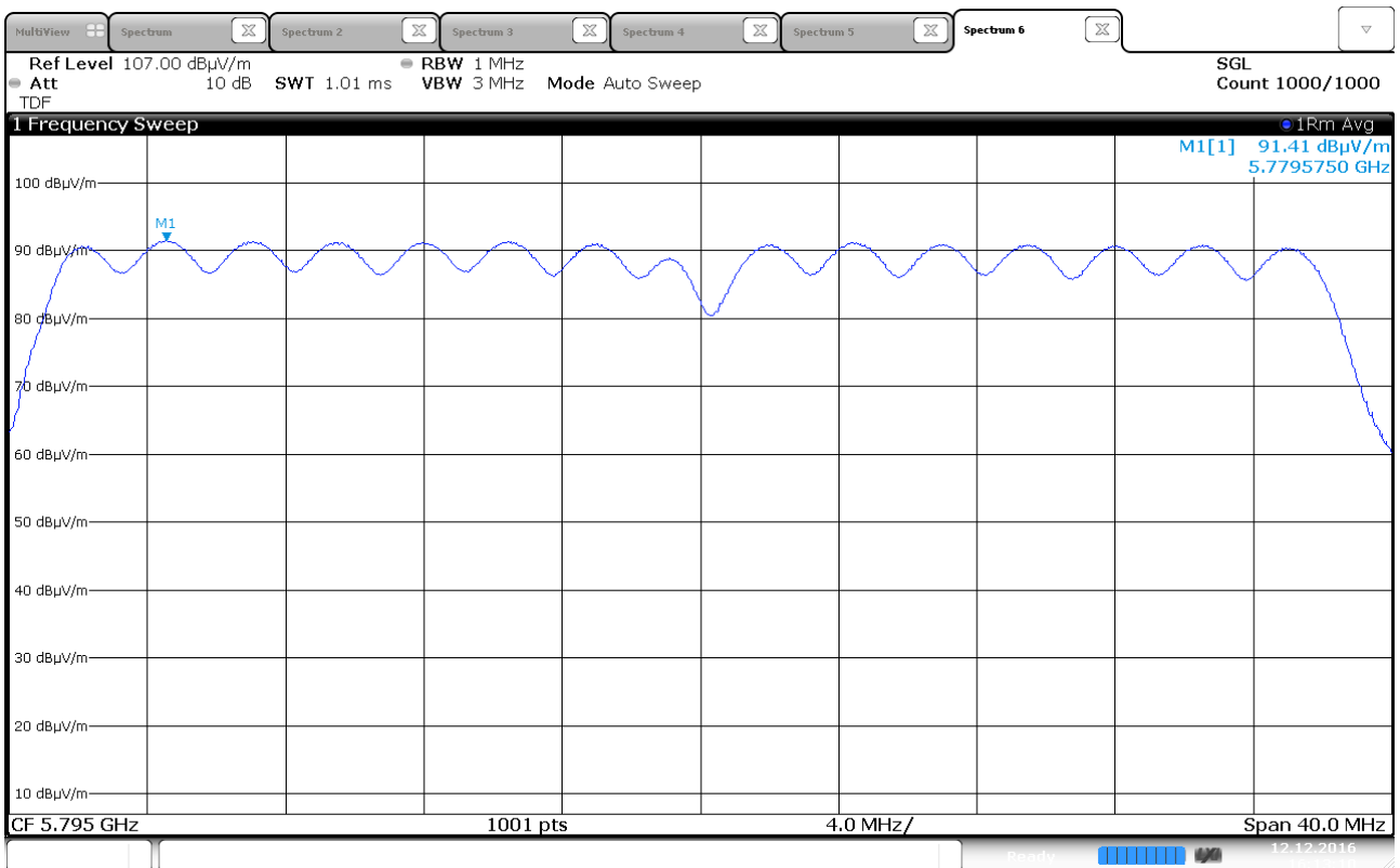
Power Spectral Density, 5795 MHz, 802.11n HT40, MIMO
