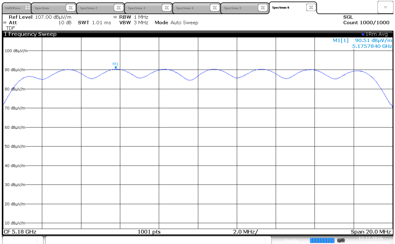
Power Spectral Density, 5180 MHz, 802.11n HT20, MIMO
