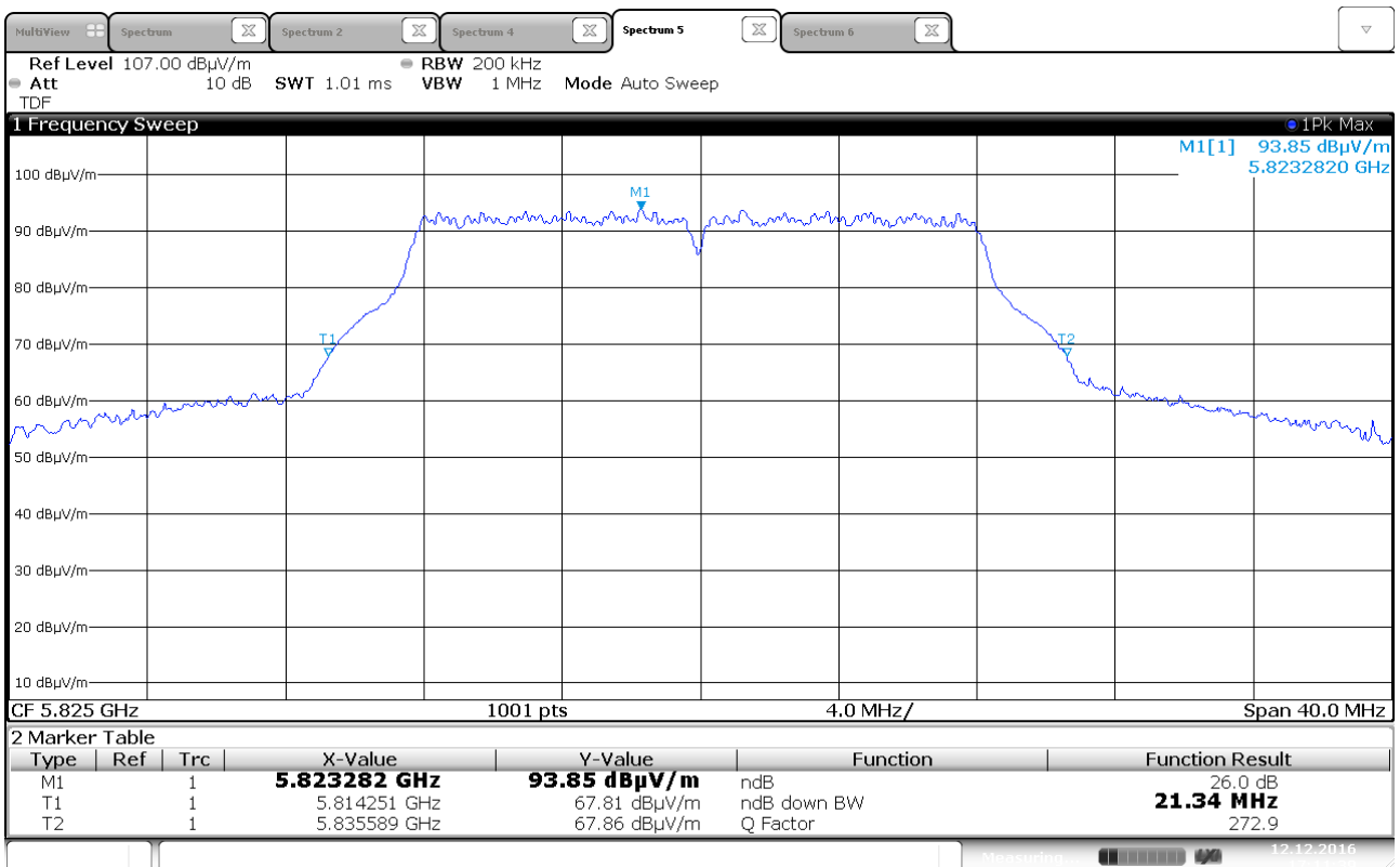
Emission Bandwidth B, 5825 MHz, 802.11a 6Mbps, Ant 1
