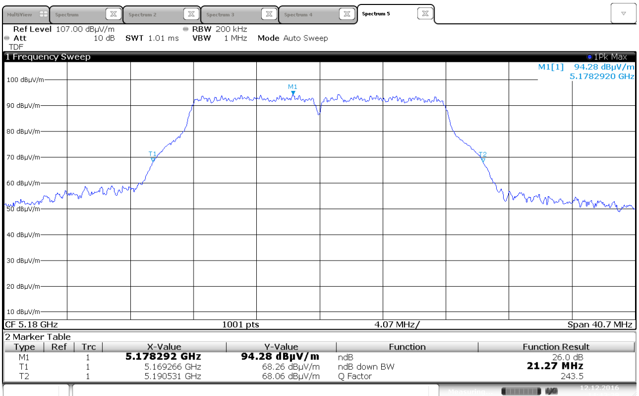
Emission Bandwidth B, 5180 MHz, 802.11a 6Mbps, Ant 1
