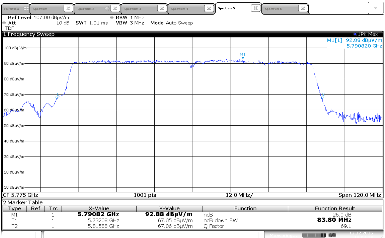
Emission Bandwidth B, 5775 MHz, 802.11n HT80, MIMO
