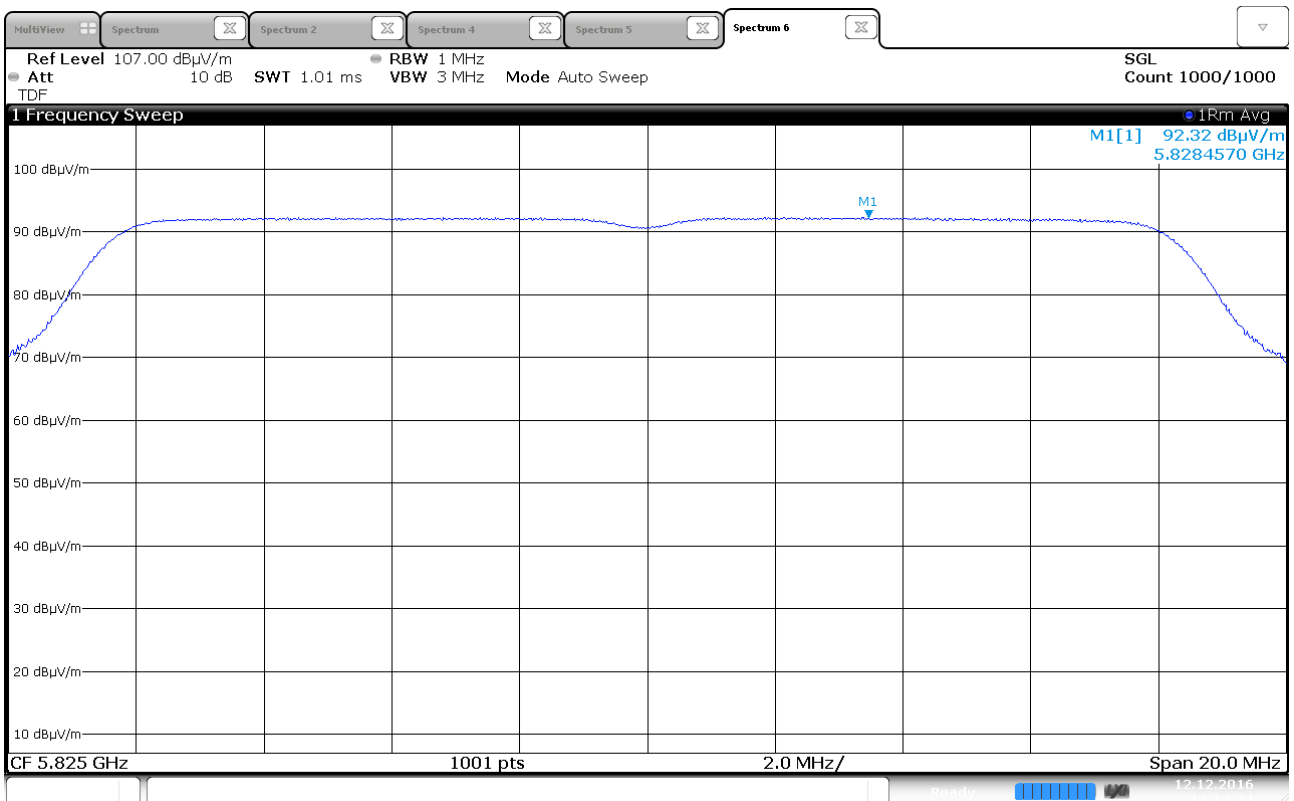
Power Spectral Density, 5825 MHz, 802.11a 6Mbps, Ant 1
