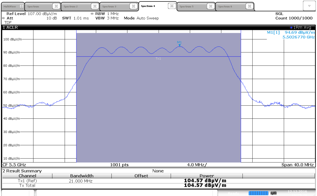
Maximum EIRP, 5500 MHz, 802.11n HT20, MIMO
