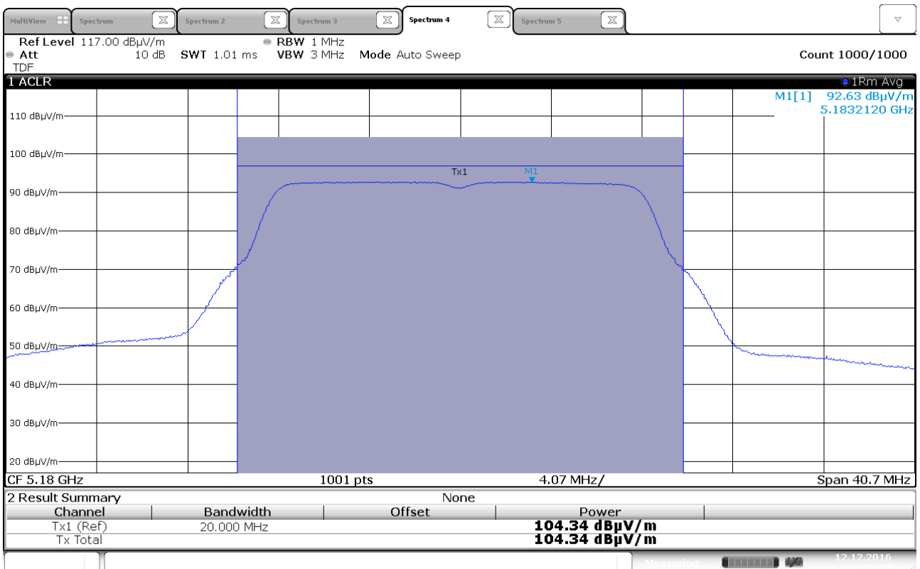
Maximum EIRP, 5180 MHz, 802.11a 6Mbps, Ant 1
