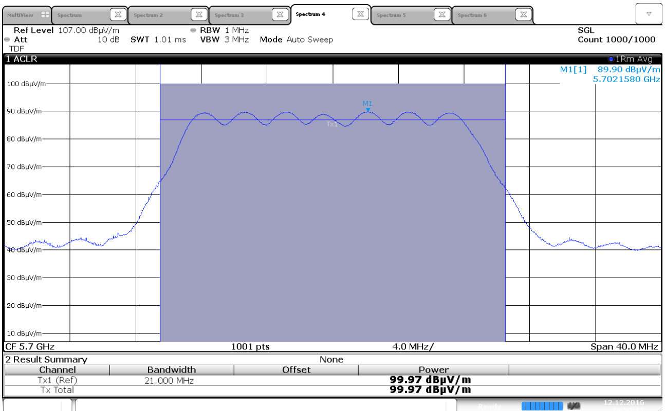
Maximum EIRP, 5700 MHz, 802.11n HT20, MIMO
