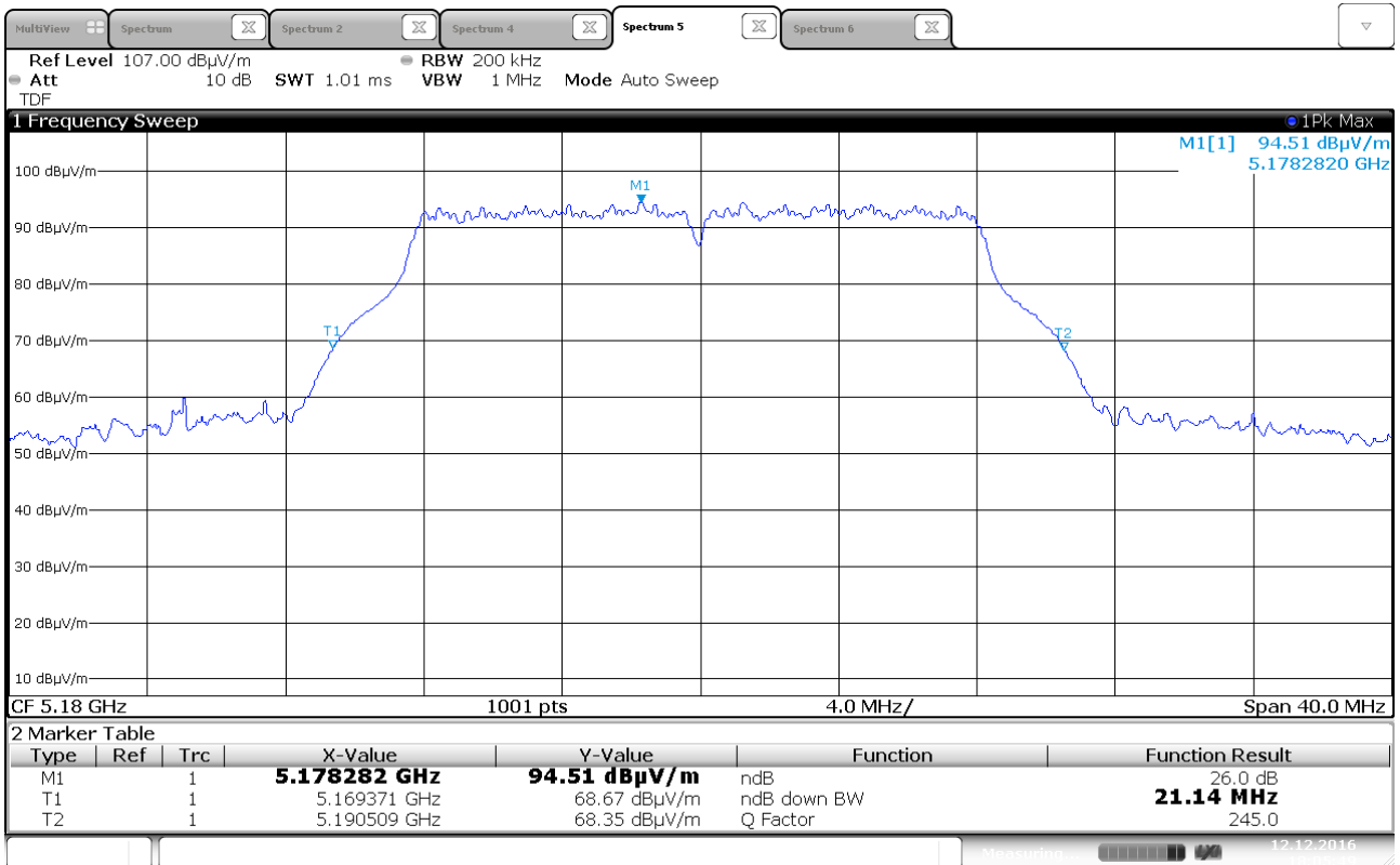
Emission Bandwidth B, 5180 MHz, 802.11a 6Mbps, Ant 0
