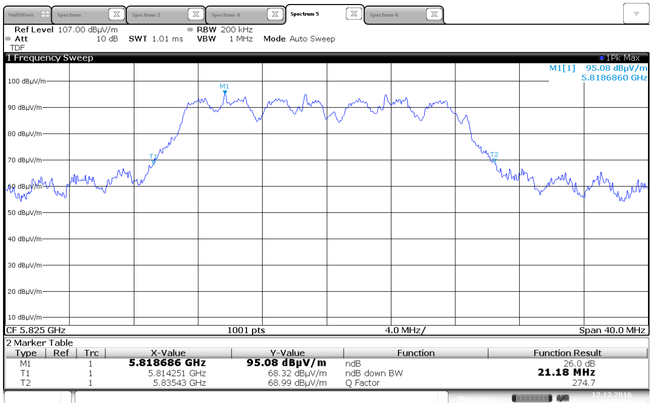
Emission Bandwidth B, 5825 MHz, 802.11n HT20, MIMO
