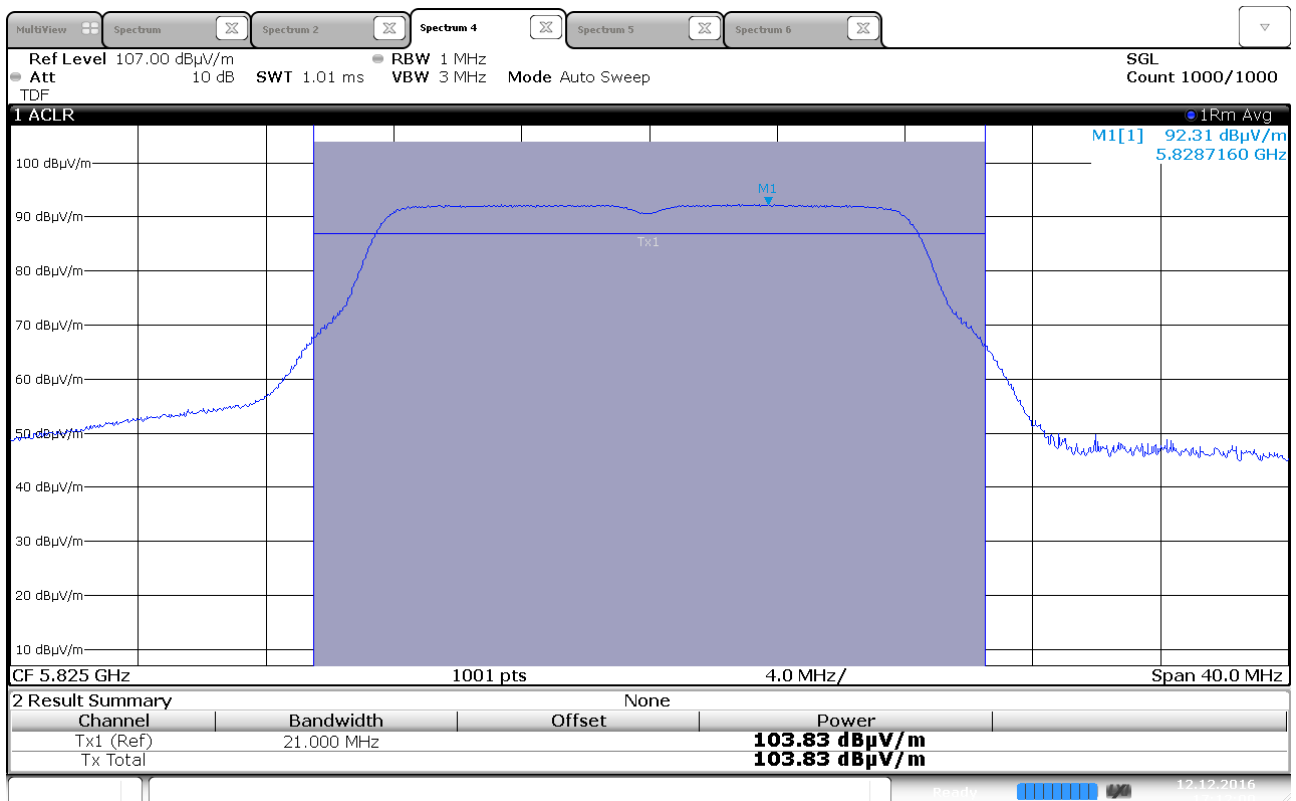
Maximum EIRP, 5825 MHz, 802.11a 6Mbps, Ant 1
