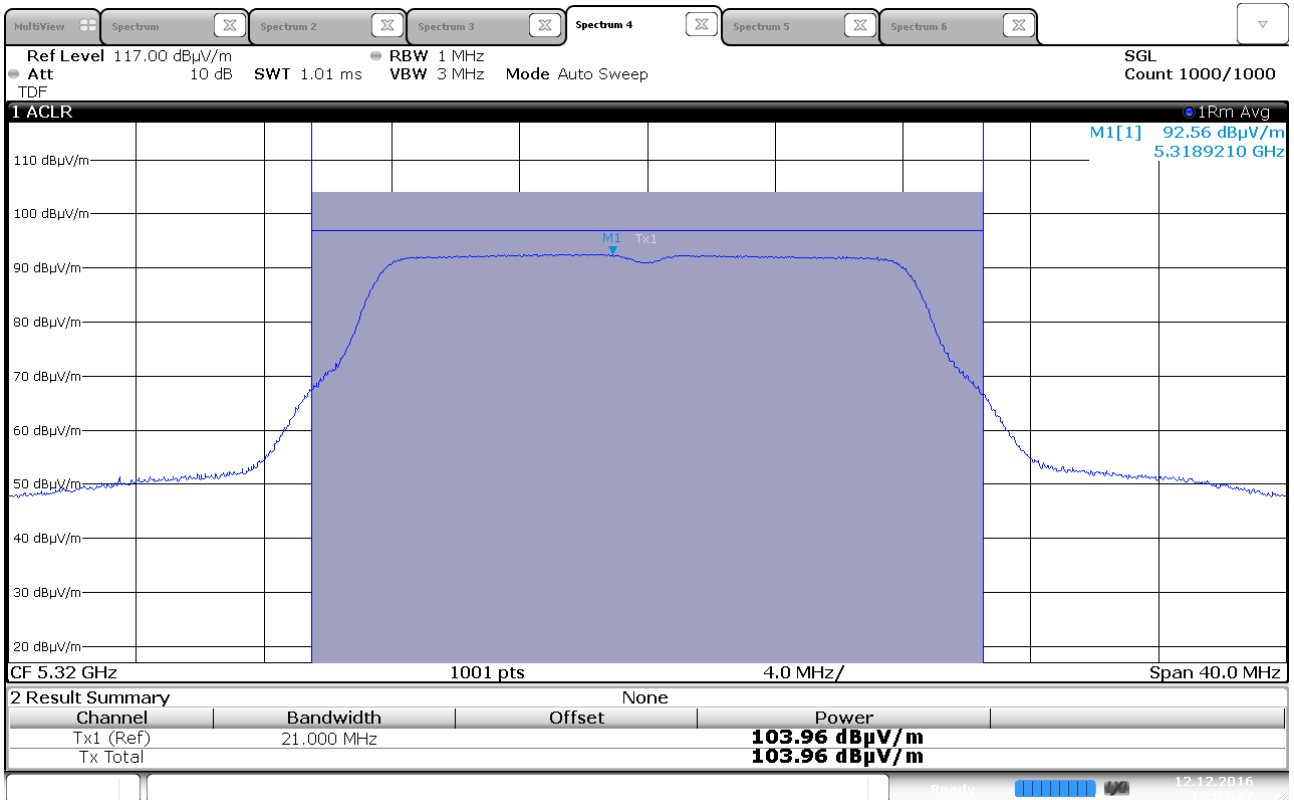
Maximum EIRP, 5320 MHz, 802.11a 6Mbps, Ant 0
