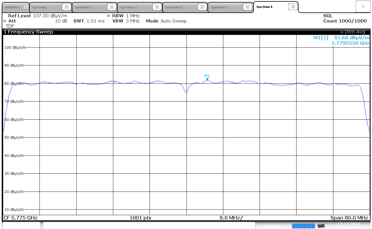
Power Spectral Density, 5775 MHz, 802.11n HT80, MIMO
