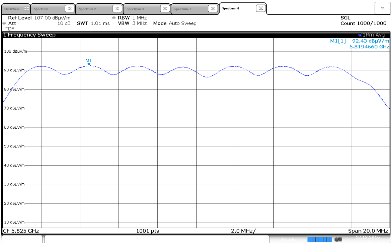
Power Spectral Density, 5825 MHz, 802.11n HT20, MIMO
