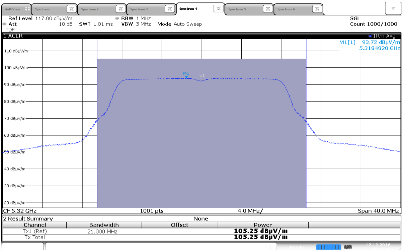
Maximum EIRP, 5320 MHz, 802.11a 6Mbps, Ant 1
