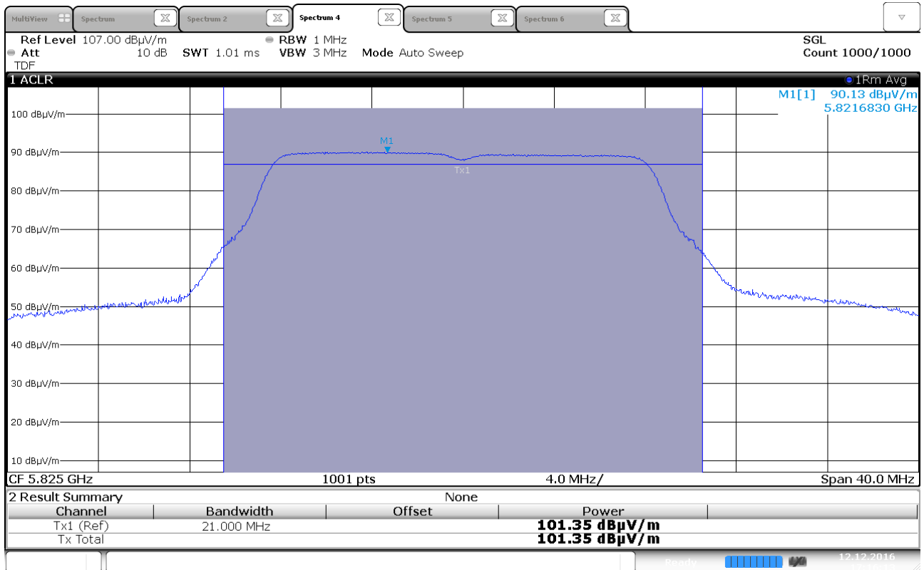
Maximum EIRP, 5825 MHz, 802.11a 6Mbps, Ant 0
