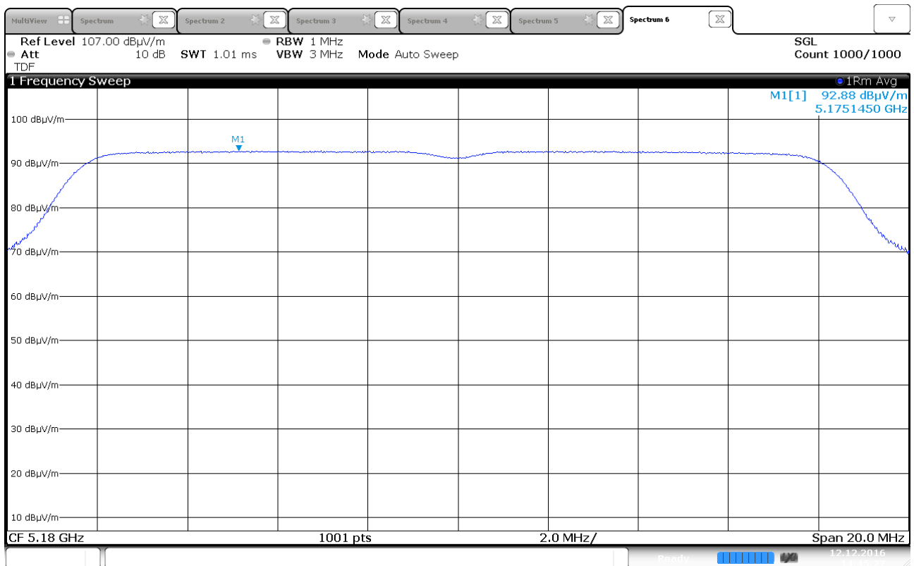
Power Spectral Density, 5180 MHz, 802.11a 6Mbps, Ant 1
