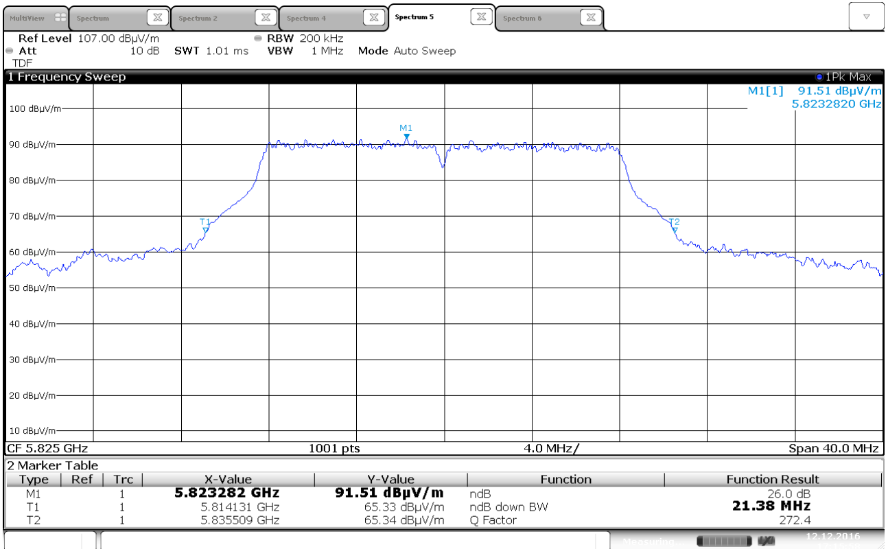
Emission Bandwidth B, 5825 MHz, 802.11a 6Mbps, Ant 0
