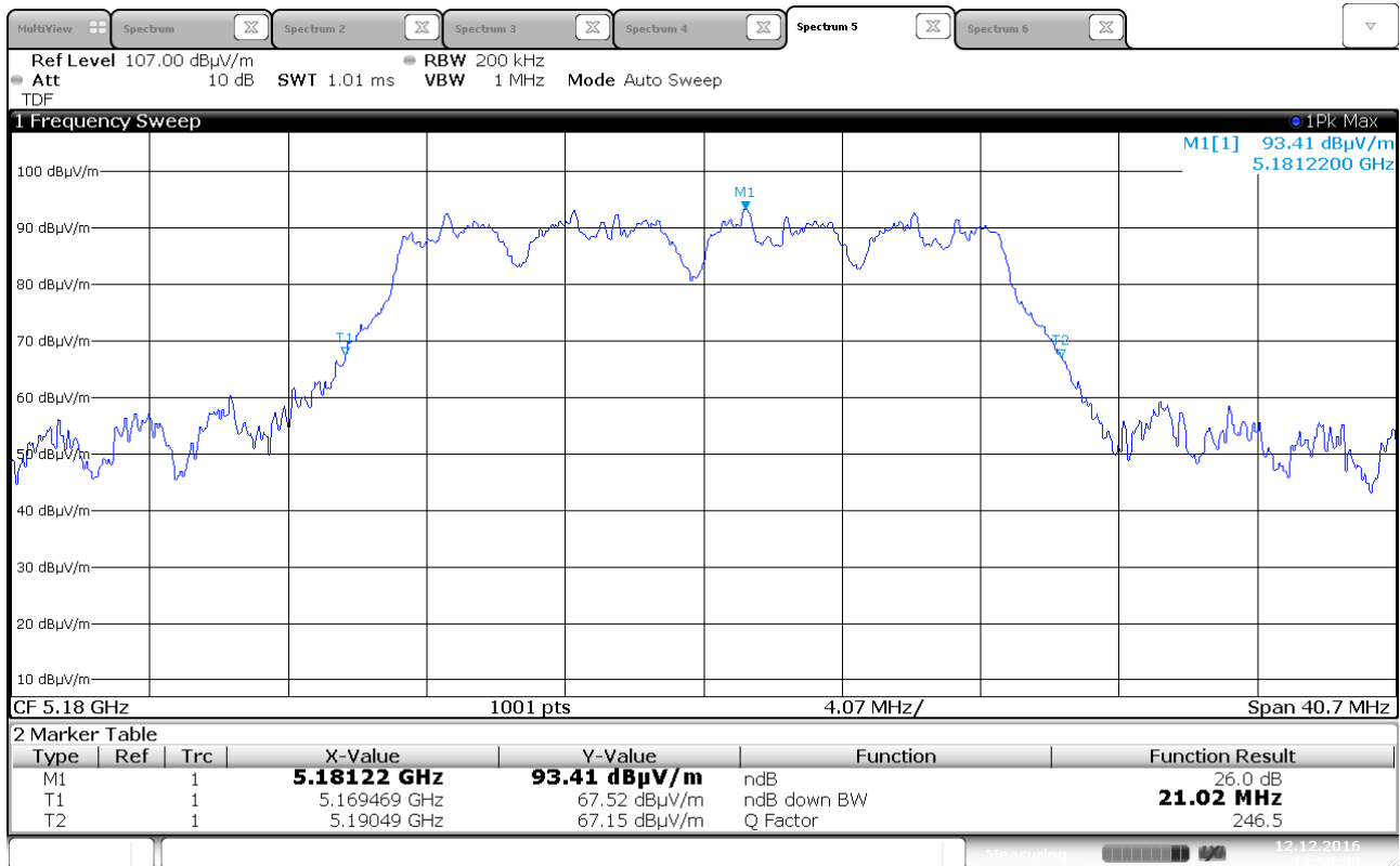
Emission Bandwidth B, 5180 MHz, 802.11n HT20, MIMO
