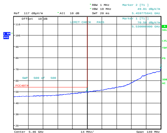
Band Edge, 5460 MHz, Ch102, 802.11n HT40 MIMO, AV, Max
