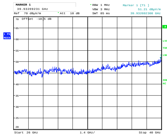
Emissions 26-40 GHz, Ch052, 802.11a 6M, Ant1, VP, @1m
