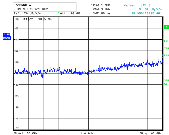
Emissions 26-40 GHz, Ch052, 802.11a 6M, Ant1, HP, @1m
