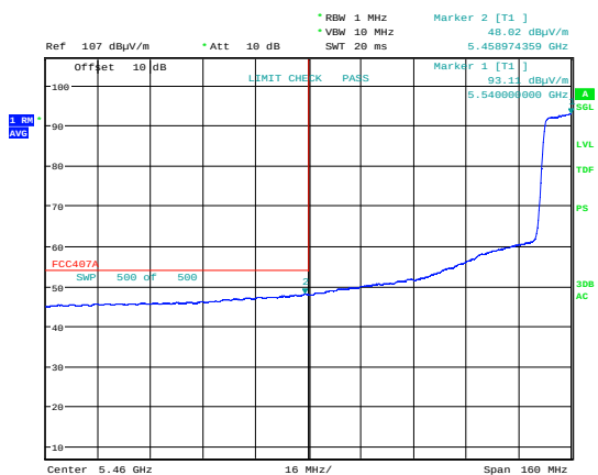
Band Edge, 5460 MHz, Ch102, 802.11n HT40 SISO, AV, Max
