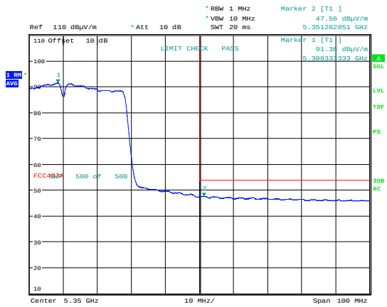
Band Edge, 5350 MHz, Ch062, 802.11n HT40 SISO, AV, Max
