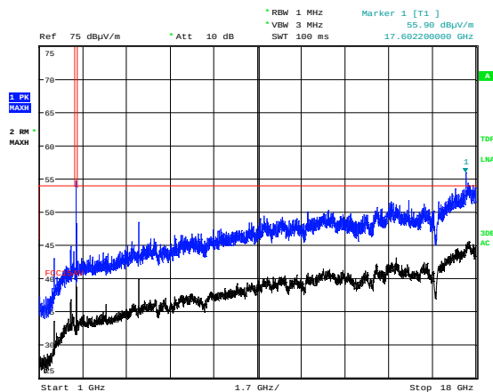
Radiated Emissions 1 - 18 GHz, 2437 MHz, 802.11n SISO, HP, Ant1
