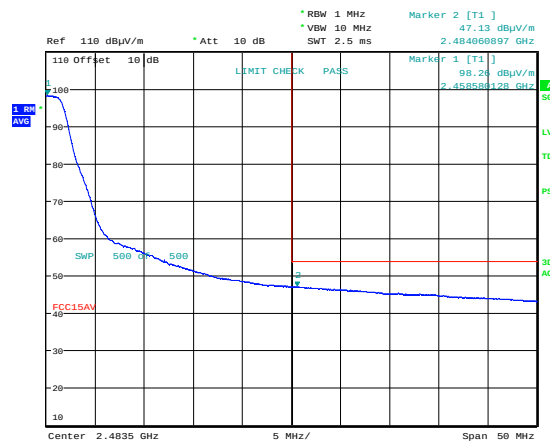
Upper Band Edge, 2447 MHz, 802.11n MIMO, Average
