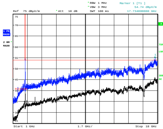
Radiated Emissions 1 - 18 GHz, 2437 MHz, 802.11g 6M, HP, Ant2
