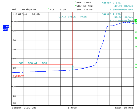
Lower Band Edge, 2412 MHz, 802.11b 11M, Average
