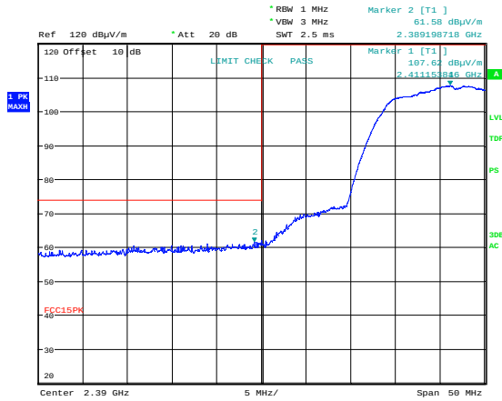
Lower Band Edge, 2412 MHz, 802.11b 11M, Peak
