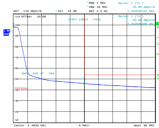
Upper Band Edge, 2427 MHz, 802.11n MIMO, Average
