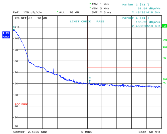
Upper Band Edge, 2447 MHz, 802.11n MIMO, Peak
