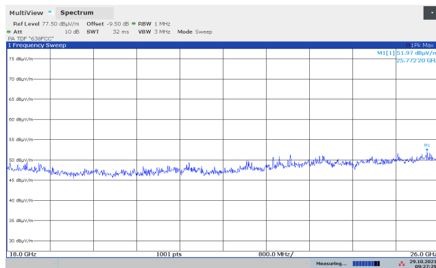
Prescan 18 - 26 GHz, 2440 MHz, 1Mb, HP, @1m
