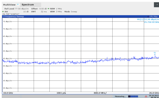
Prescan 18 - 26 GHz, 2440 MHz, 1Mb, VP, @1m
