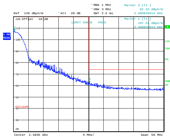
Upper Band Edge, 2452 MHz, 802.11g 6M, Peak, Ant 0
