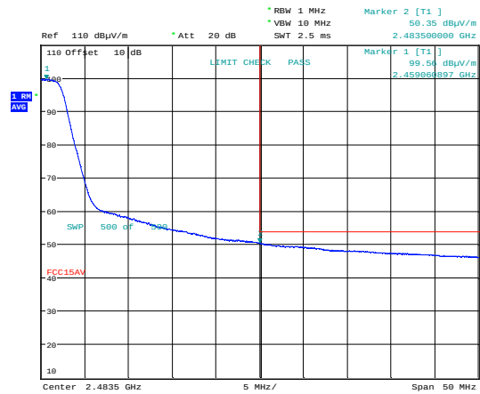
Upper Band Edge, 2452 MHz, 802.11n MIMO, Average, Ant 0
