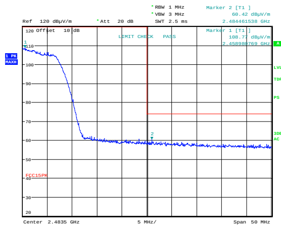
Upper Band Edge, 2457 MHz, 802.11n SISO, Peak, Ant 0
