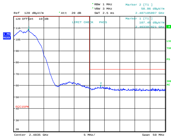
Upper Band Edge, 2457 MHz, 802.11n MIMO, Peak, Ant 0
