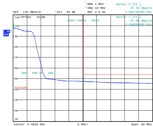
Upper Band Edge, 2457 MHz, 802.11n SISO, Average, Ant 0
