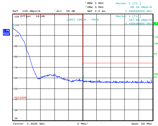
Upper Band Edge, 2452 MHz, 802.11n MIMO, Peak, Ant 0
