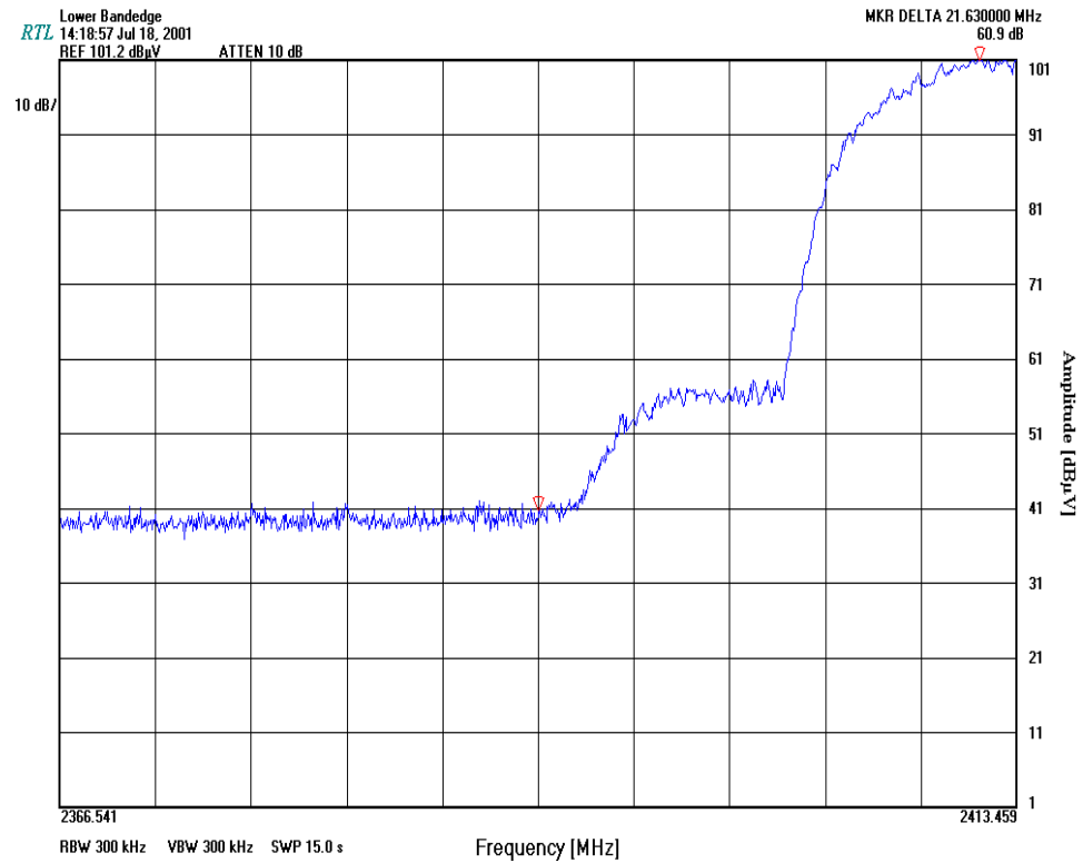
PLOT 9-1: BANEDGE: LOWER BAND EDGE (60.9dB) CHANNEL 1 (ITRONIX IX250)
