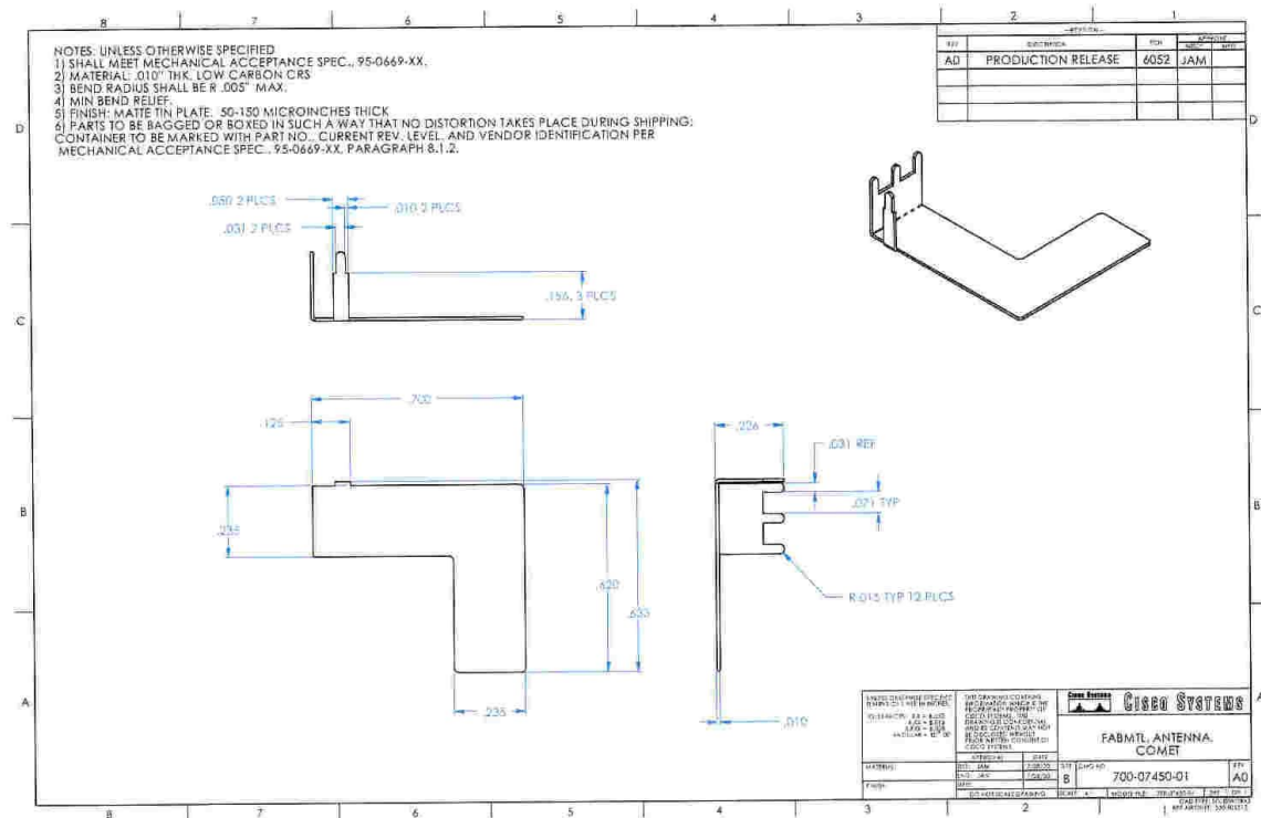
Figure 1. Mechanical Drawing of the Comet Inverted-F Antenna
