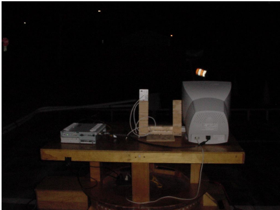
PHOTOGRAPH 16: RADIATED EMISSION REAR AIR-ANT5959
