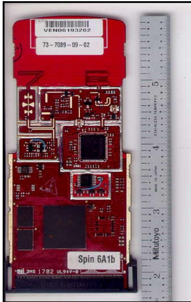
PHOTOGRAPH 10: UNSHIELDED BOTTOM
