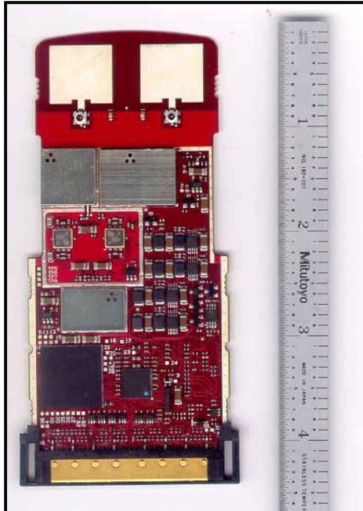
PHOTOGRAPH 7: SHIELDED TOP
