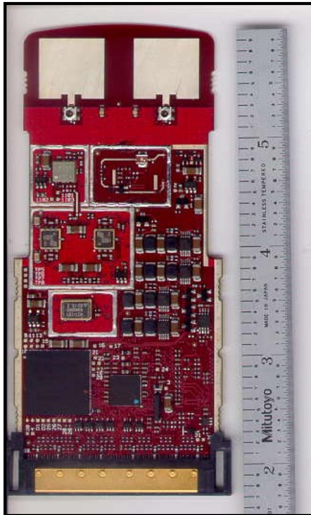
PHOTOGRAPH 9: UNSHIELDED TOP
