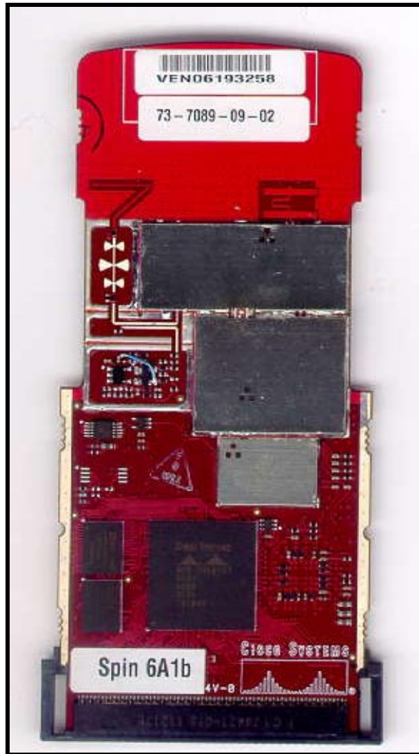
PHOTOGRAPH 8: SHIELDED BOTTOM
