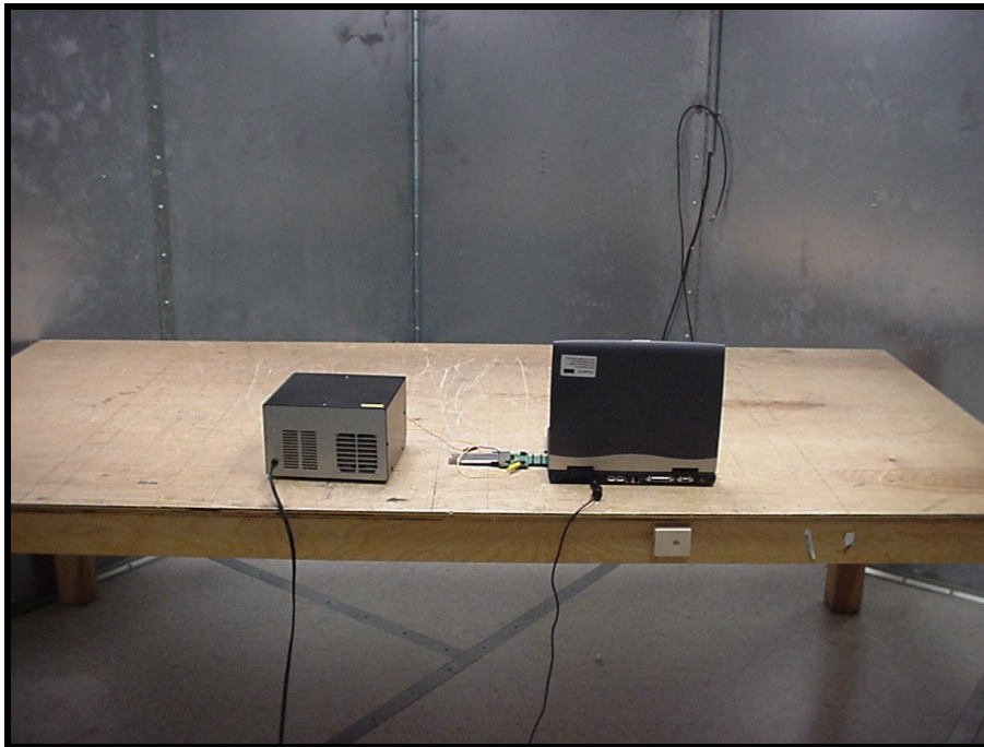
PHOTOGRAPH 4: CONDUCTED EMISSION REAR VIEW
