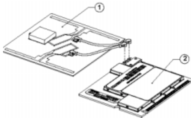
Figure 7-3 Antenna Wires
