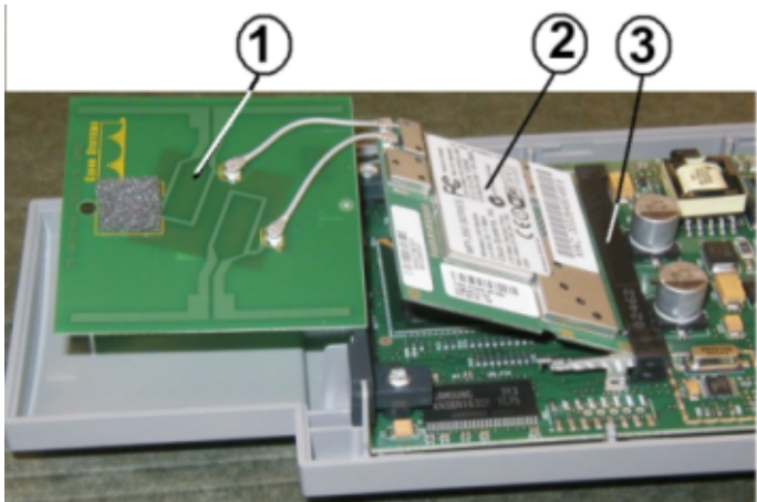
Figure 7-4 Inserting Radio Card in Mini-PCI Connector
