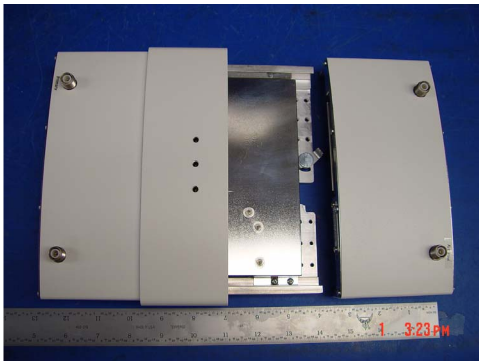
AIR-RM23A-A-K9 Radio Module prior to installation in AIR-AP1250 (with collocated AIR-RM23G-A-K9)
