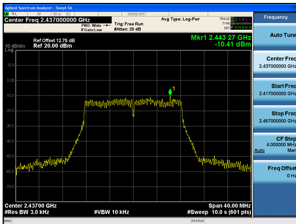
Power Spectral Density, 2437 MHz, HT-20 STBC, M0 to M7
