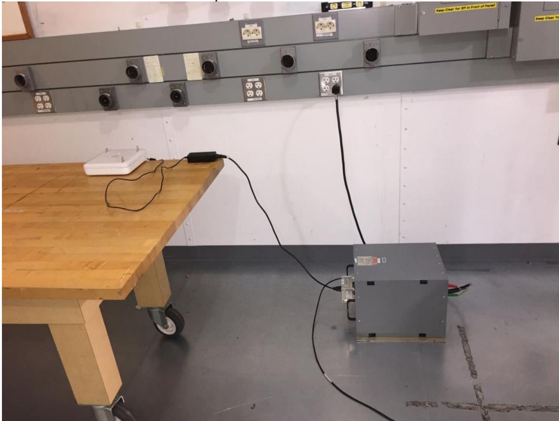
AC Mains Conducted Emissions setup
