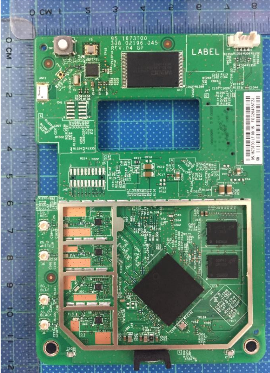
Top Side Board without Shields
