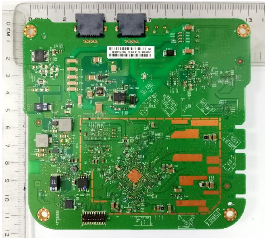
Bottom Side RF Board
