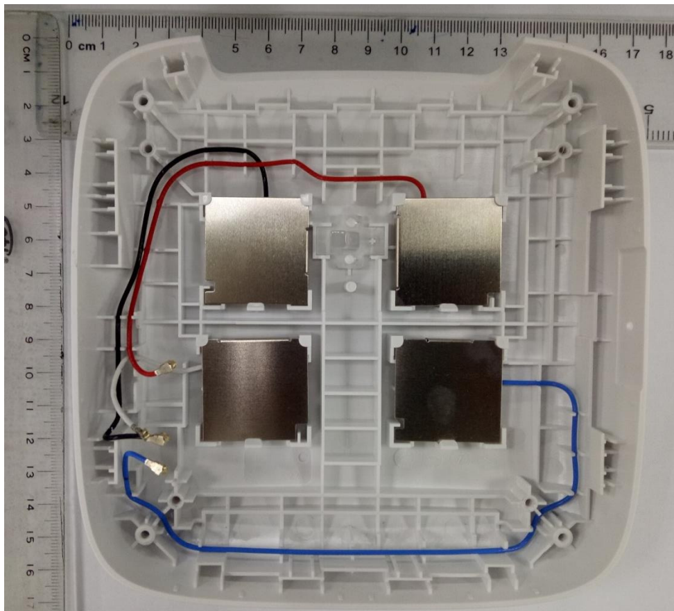
Antenna View
