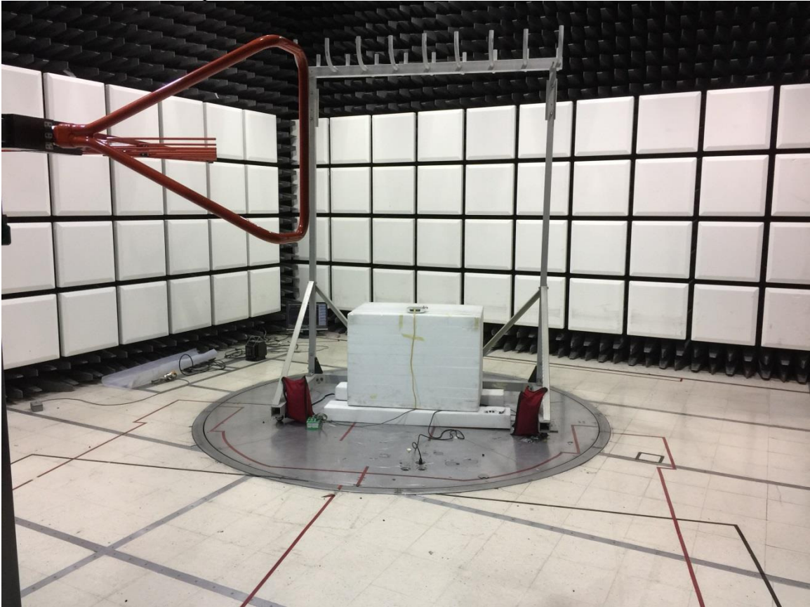
Radiated Emissions setup 30MHz – 1GHz
