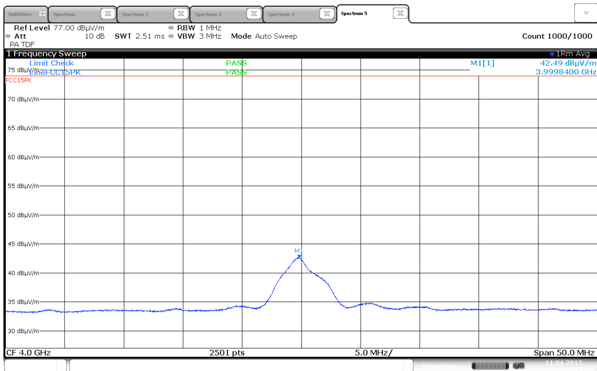
Radiated Emissions, 4000MHz RMS, 2440MHz, GFSK (Max: VP)
