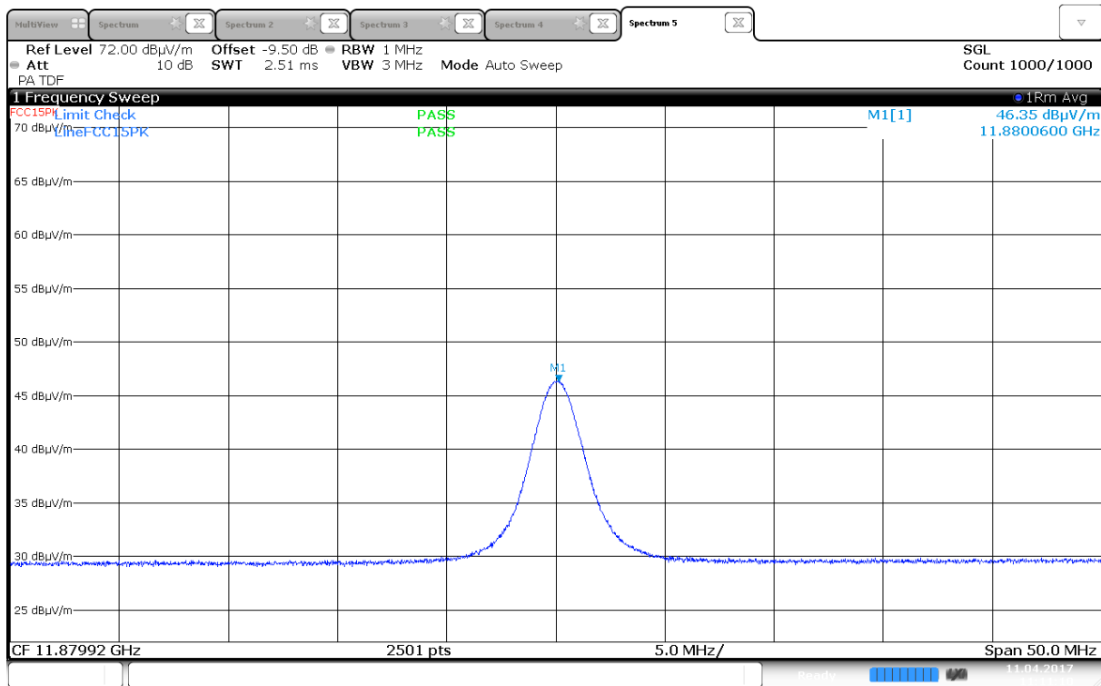
Radiated Emissions RMS, 11880MHz, 2440MHz, GFSK (Max: HP)
