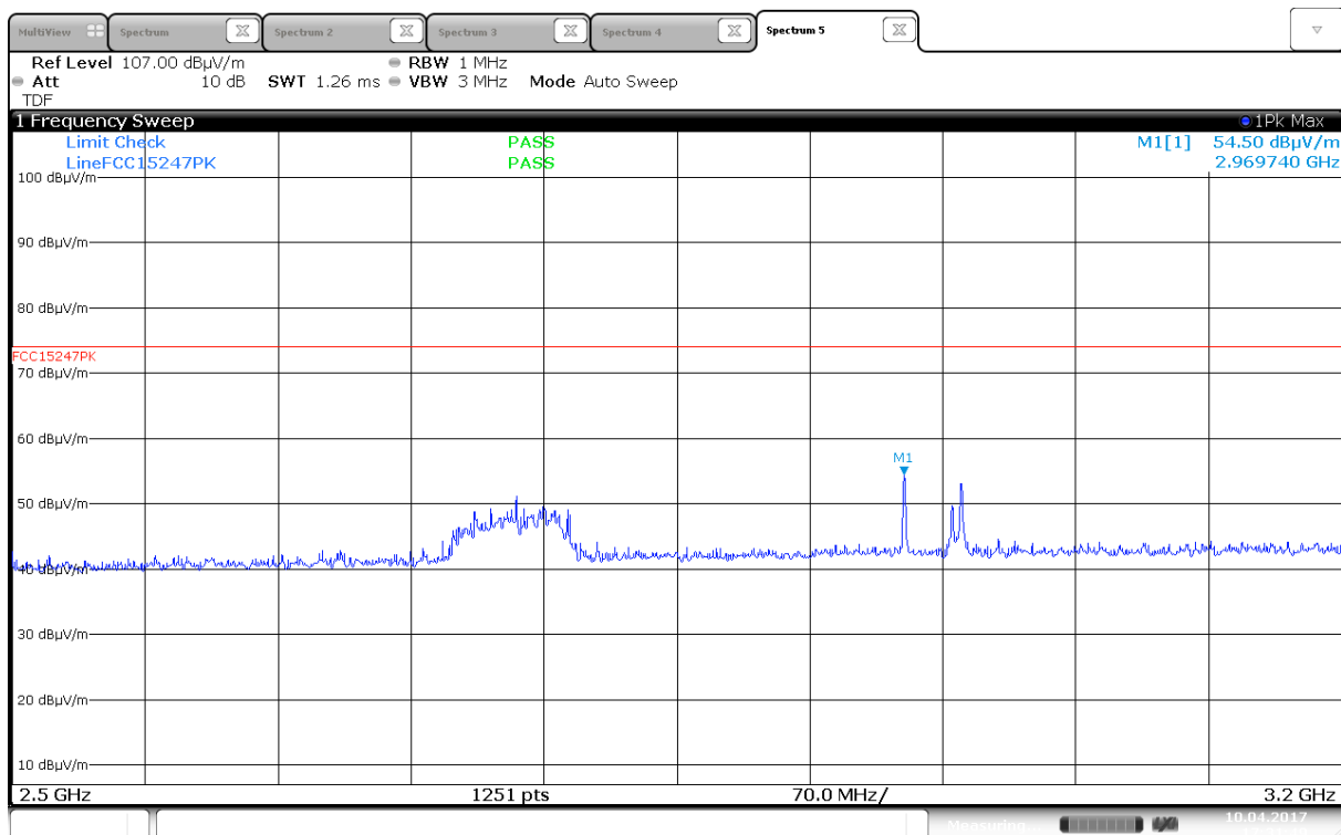
Radiated Emissions, 2500 -3200 MHz, 2462MHz, 802.11n, MCS0, MIMO, VP
