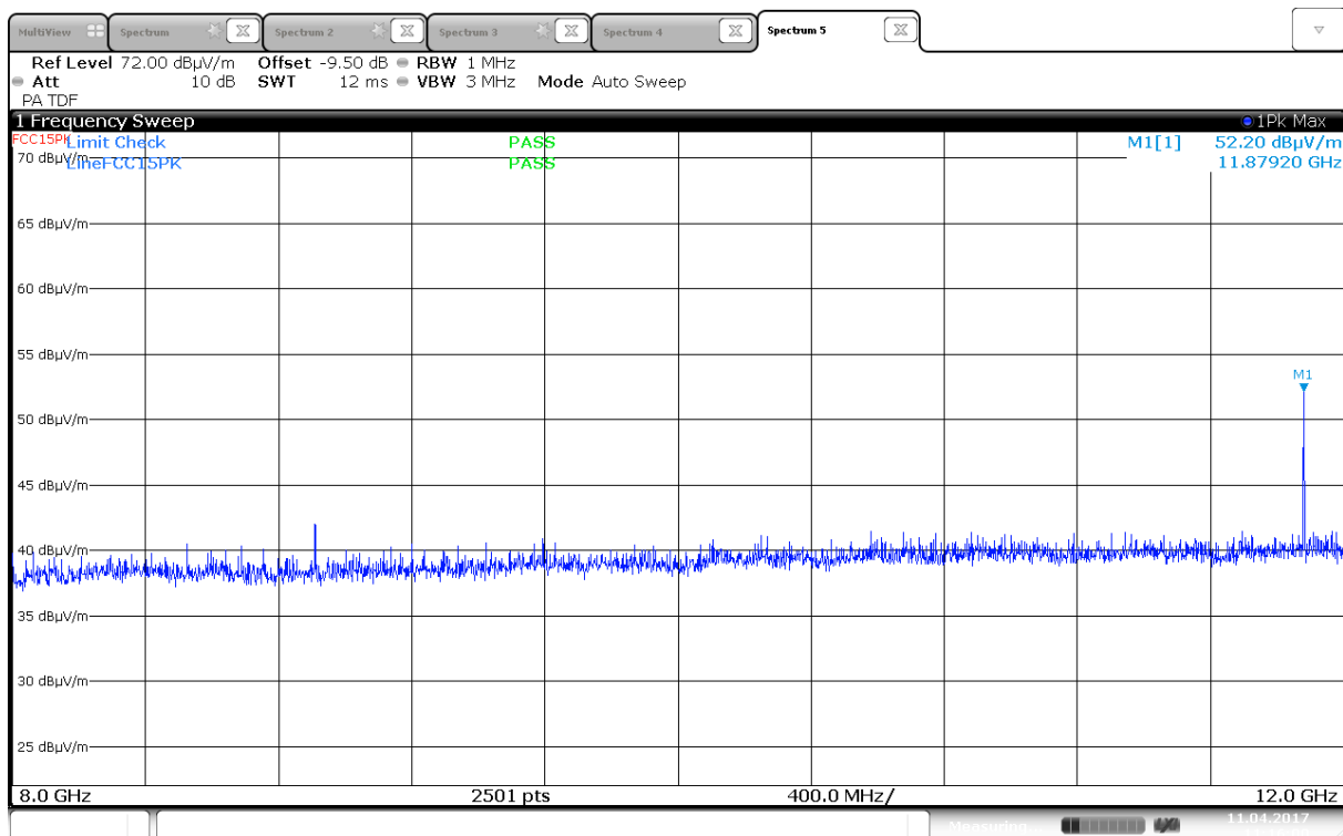
Radiated Emissions, 8000 -12000 MHz, 2437MHz, 802.11n, HT20, MIMO, VP, @1m
