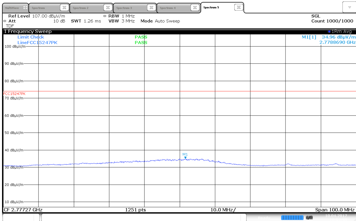
Radiated Emissions Av, 2779MHz, 2452MHz (Max: HP) (Same for all RF-modulations and frequencies)
