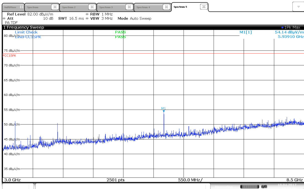
Radiated Emissions, 3000 -8500 MHz, 2437MHz, 802.11b, 1Mbps, Ant0, VP
