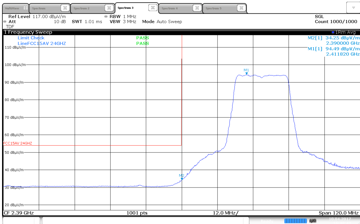
Lower Band Edge, Average, 2417 MHz, 802.11n, MCS0, MIMO (Max: HP)
