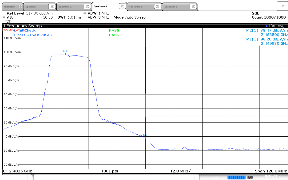
Upper Band Edge, Average, 2452 MHz, 802.11g, 6Mbps, (Max: Ant 0, HP)
