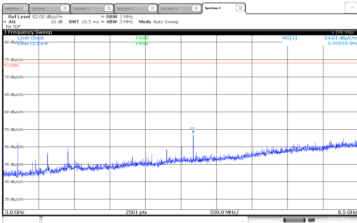
Radiated Emissions, 3000 -8500 MHz, 2437MHz, 802.11n, HT20, MIMO, VP
