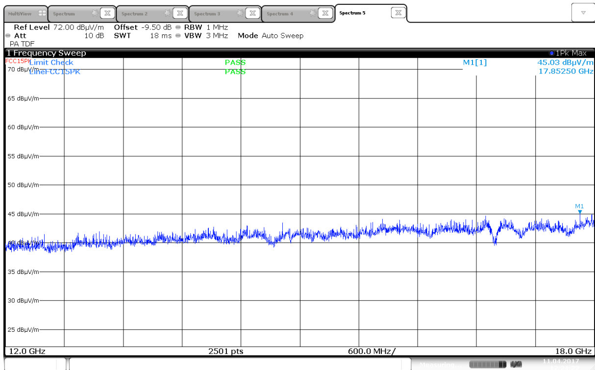
Radiated Emissions, 12000 -18000 MHz, 2437MHz, 802.11n, MCS0, MIMO, HP, @1m
