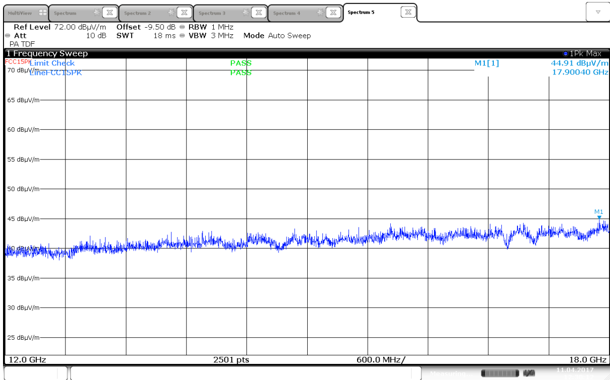
Radiated Emissions, 12000 -18000 MHz, 2437MHz, 802.11b, 1Mbps, Ant0, HP, @1m
