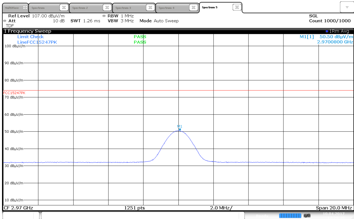
Radiated Emissions Av, 2970MHz, 2462MHz (Max: HP) (Same for all RF-modulations and frequencies)
