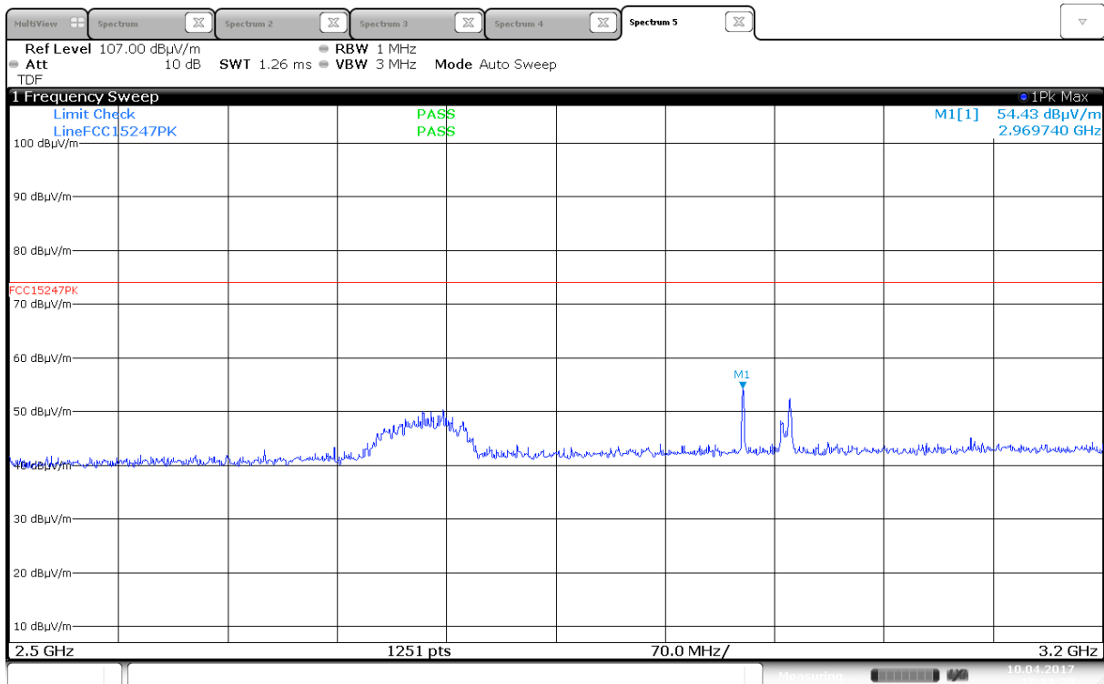
Radiated Emissions, 2500 -3200 MHz, 2462MHz, 802.11b, 1Mbps, Ant0, VP
