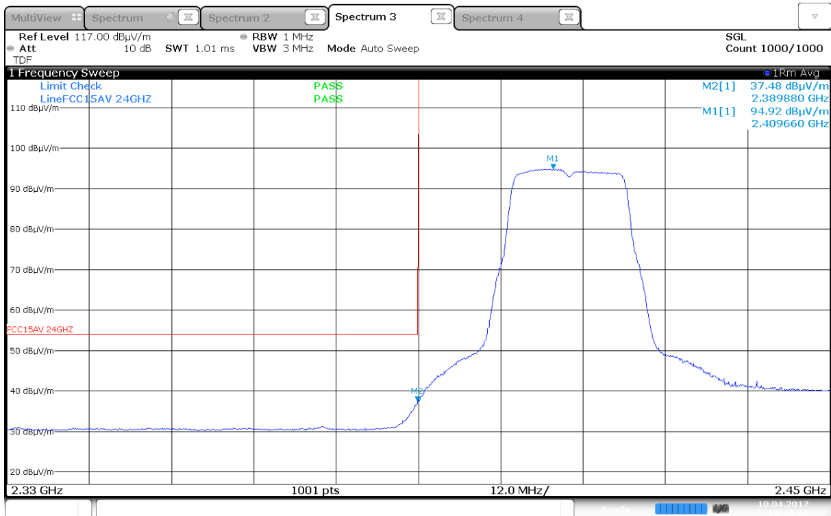
Lower Band Edge, Average, 2412 MHz, 802.11g, 6Mbps, (Max: Ant 0, HP)
