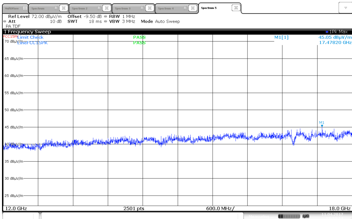
Radiated Emissions, 12000 -18000 MHz, 2437MHz, 802.11b, 1Mbps, Ant1, VP, @1m
