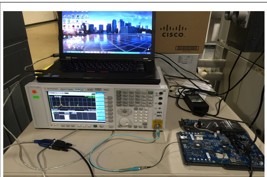
Title: RF Conducted Test Setup
