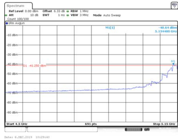
non HT80, 6 to 54 Mbps 5210 MHz Average
