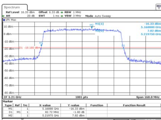
HE80, M0 to M11 5210 MHz 26dB BW
