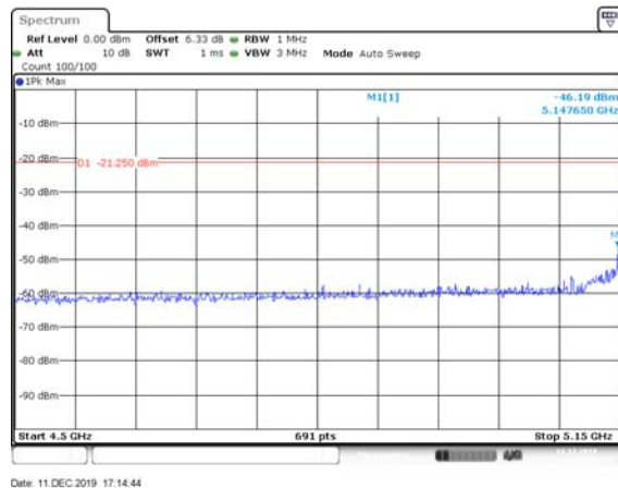
HE80, M0.1 to M11.1-BF 5210 MHz Peak
