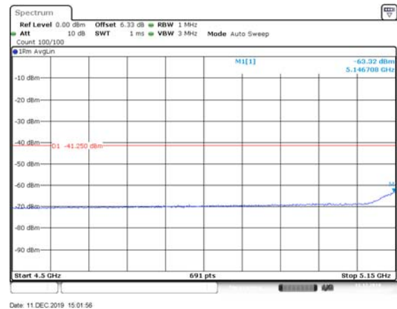
HE80, M0.1 to M11.1-BF 5210 MHz Average
