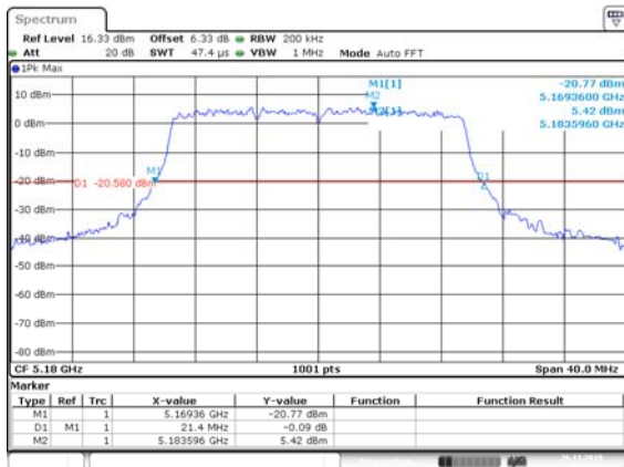
HE20, M0 to M11 5180 MHz 26dB BW
