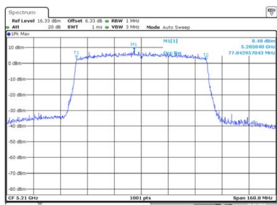
HE80, M0 to M11 5210 MHz 99% OBW
