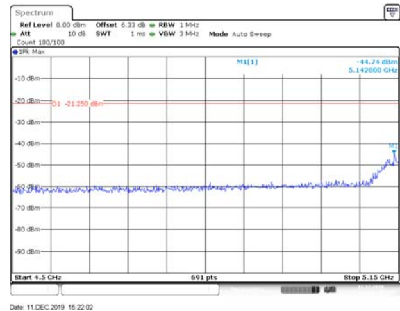
VHT80, M0.1 to M9.1 5210 MHz Average
