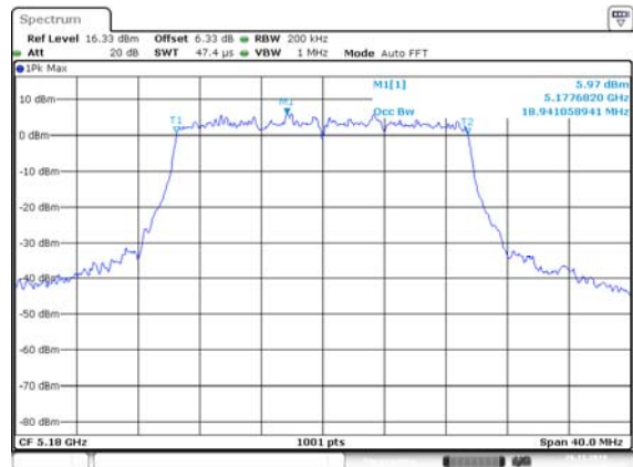
HE20, M0 to M11 5180 MHz 99% OBW
