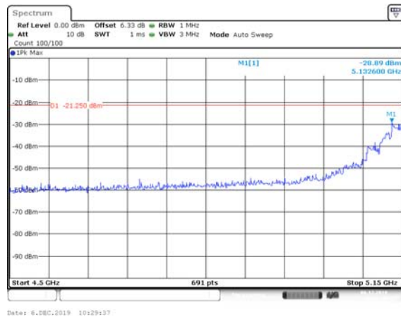
non HT80, 6 to 54 Mbps 5210 MHz Peak
