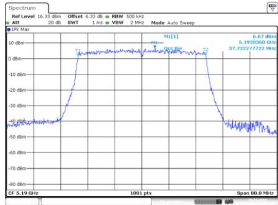
HE40, M0 to M11 5190 MHz 99% OBW
