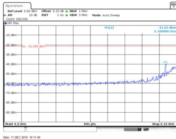
VHT80, M0.1 to M9.1 5210 MHz Peak
