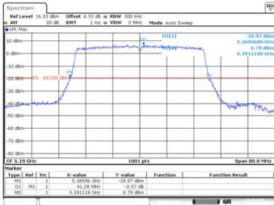
HE40, M0 to M11 5190 MHz 26dB BW
