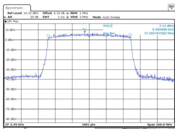
HE80, M0 to M11 5290 MHz 99% OBW
