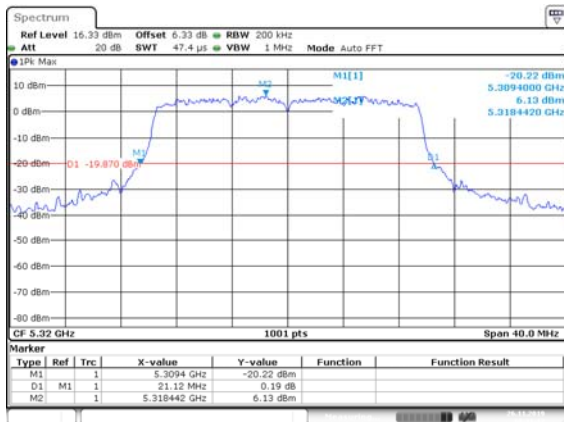
HE20, M0 to M11 5320 MHz 26dB BW
