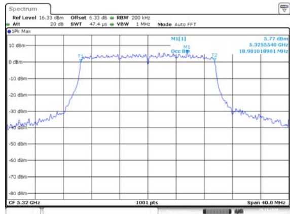
HE20, M0 to M11 5320 MHz 99% OBW
