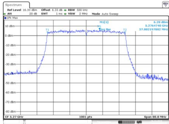
HE40, M0 to M11 5270 MHz 99% OBW
