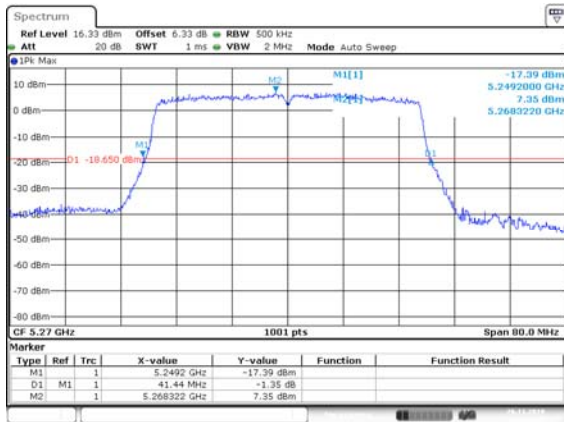
HE40, M0 to M11 5270 MHz 26dB BW
