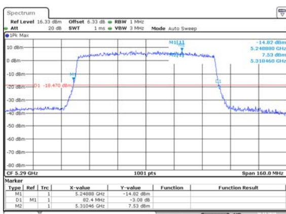
HE80, M0 to M11 5290 MHz 26dB BW
