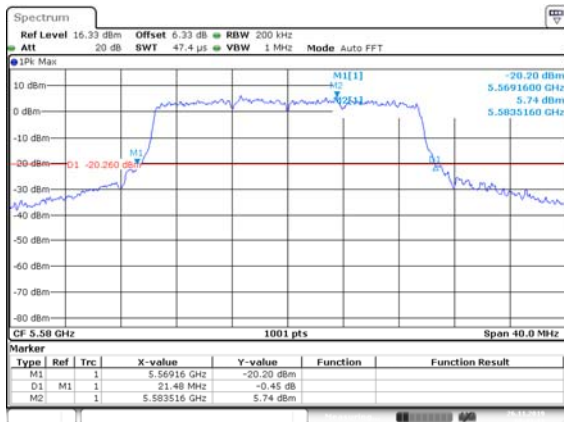
HE20, M0 to M11 5580 MHz 26dB BW
