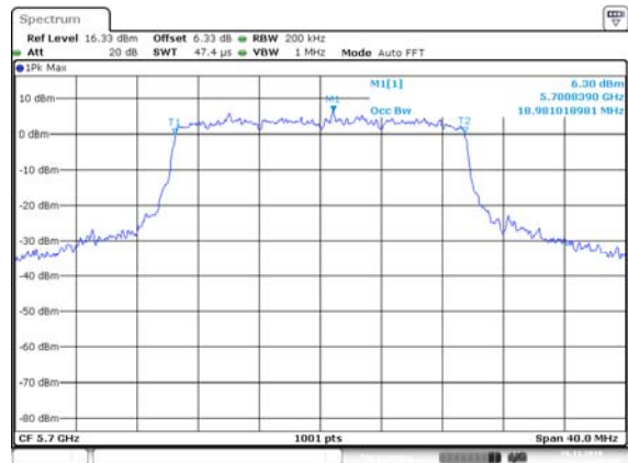
HE20, M0 to M11 5700 MHz 99% OBW
