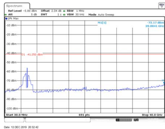
VHT80, M0.1 to M9.1 5690 MHz Average
