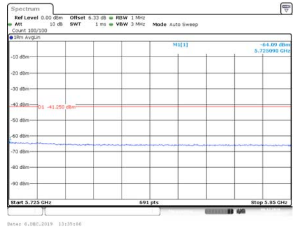
HE80, M0.1 to M11.1-BF 5610 MHz Average
