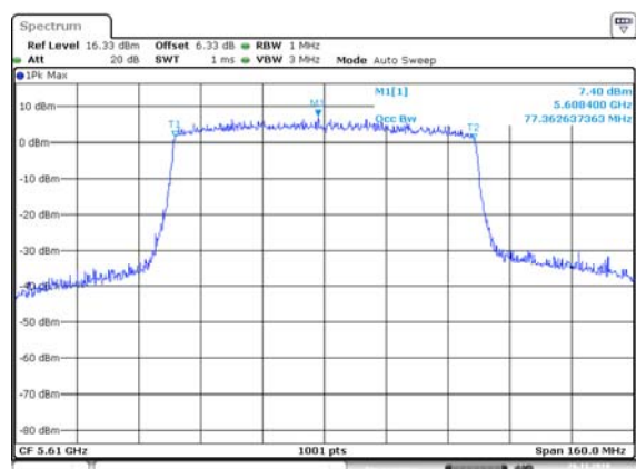
VHT80, M1 to M9 ss=1 5610 MHz 99% OBW
