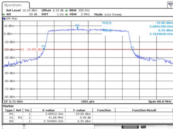
non HT40, 6 to 54 Mbps 5710 MHz 26dB BW
