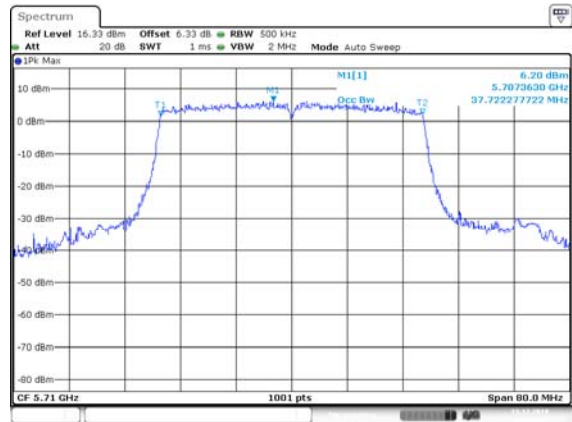
non HT40, 6 to 54 Mbps 5710 MHz 99% OBW
