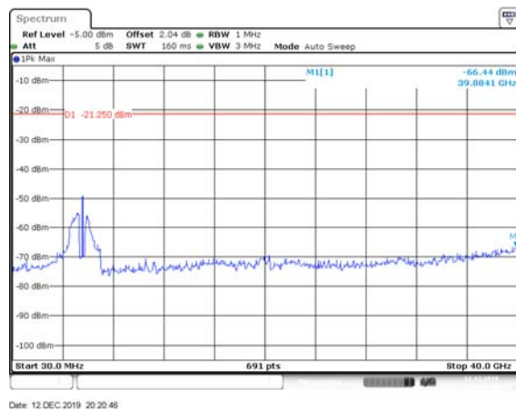
VHT80, M0.1 to M9.1 5690 MHz Peak
