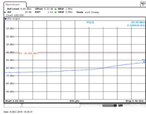
VHT80, M0.1 to M9.1 5530 MHz Average
