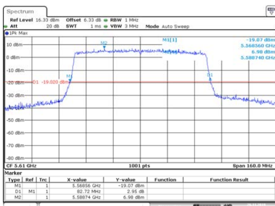
VHT80, M1 to M9 ss=1 5610 MHz 26dB BW
