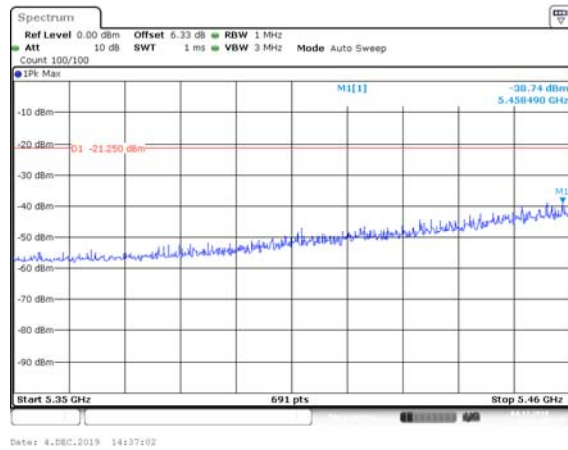
HE80, M0.1 to M11.1-BF 5530 MHz Peak
