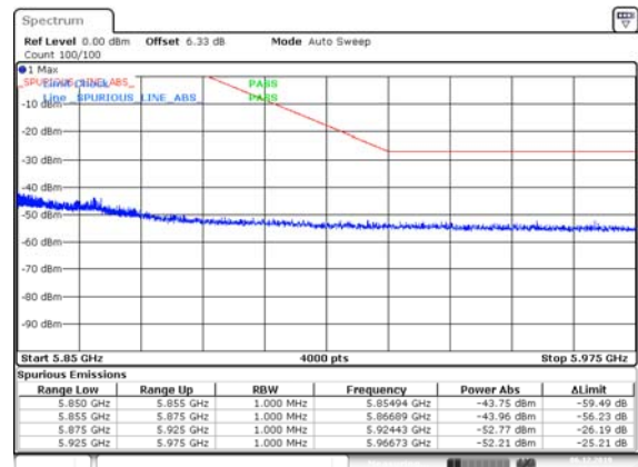
VHT80, M0.1 to M9.1 Right
