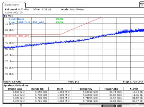
VHT80, M0.1 to M9.1 Left
