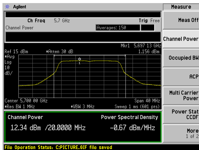
Ant-4
