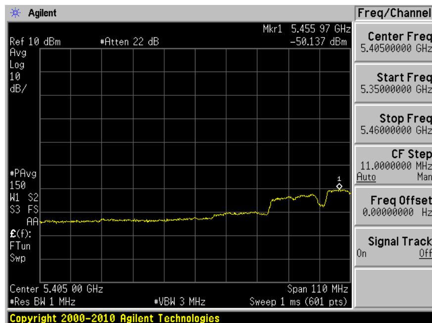
Ant-2
