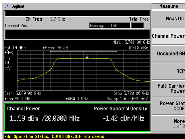
Ant-2
