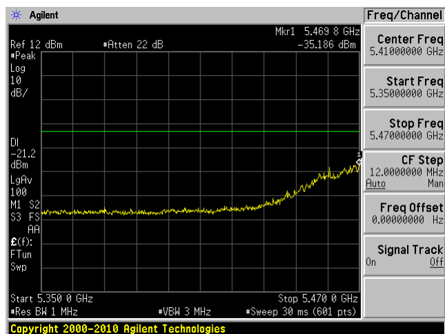
Ant-b
