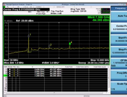
Antenna D
