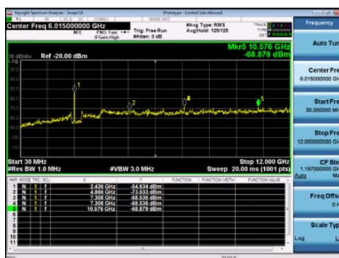
Antenna D
