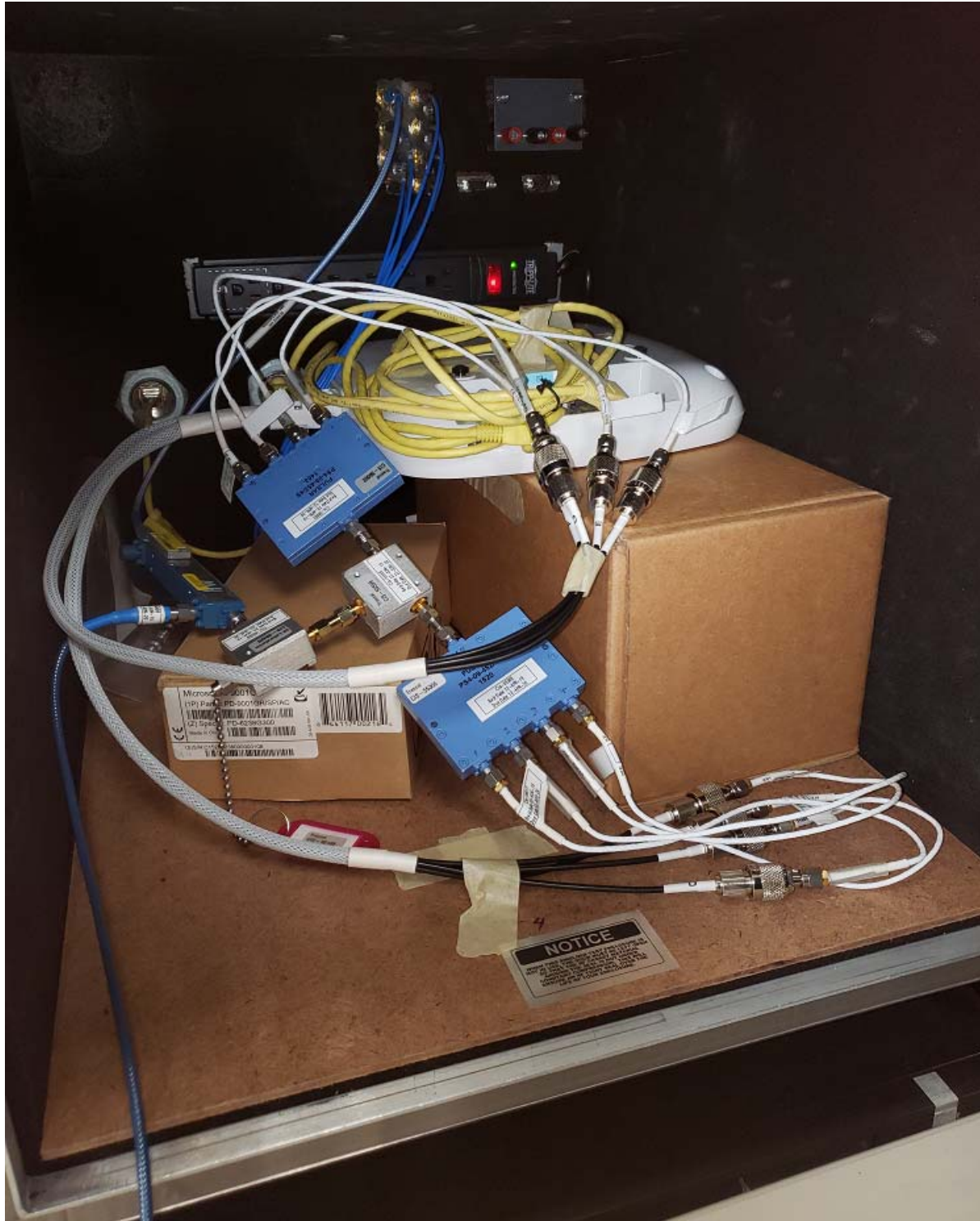
Title: Radio Conducted DFS Test Setup
