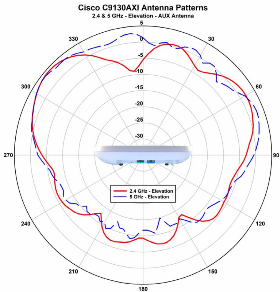
Figure 3-8 C9130AXI - AUX Antenna radiation pattern (2.4 GHz and 5 GHz Elevation)
