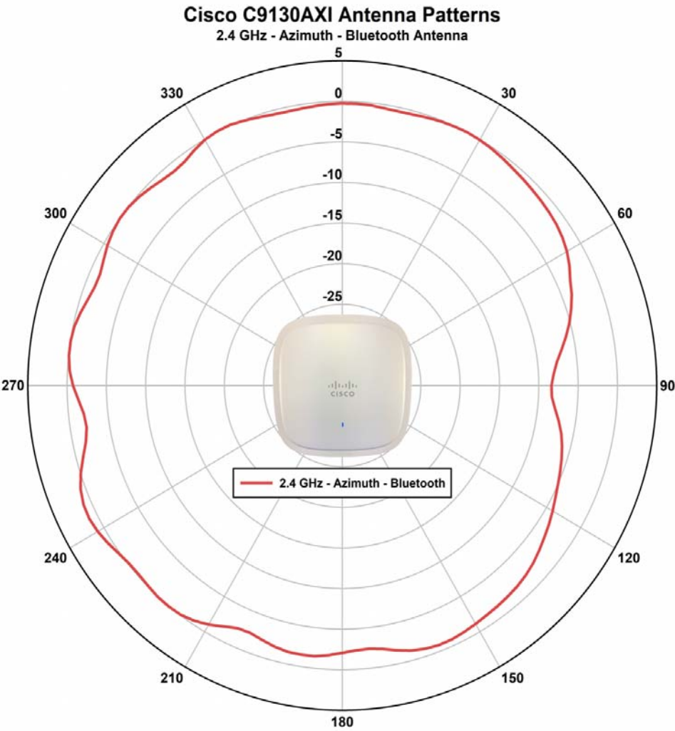
Figure 3-9 C9130AXI - Bluetooth Antenna radiation pattern (2.4 GHz Azimuth)
