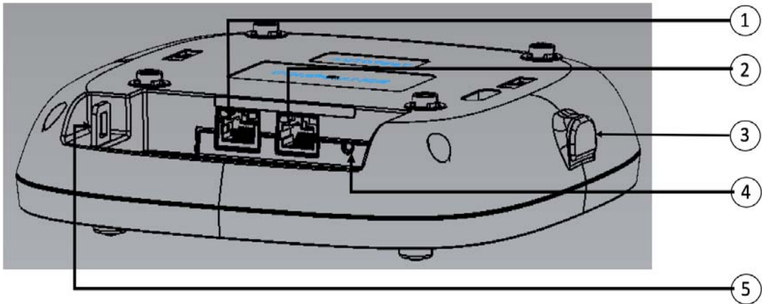
Figure 4 Ports and Connections on the Head of the 9130AXE Model
