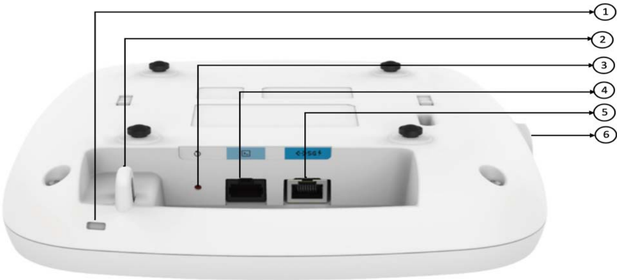
Figure 2 Ports and Connectors on the Head of the 9130AXI Model
