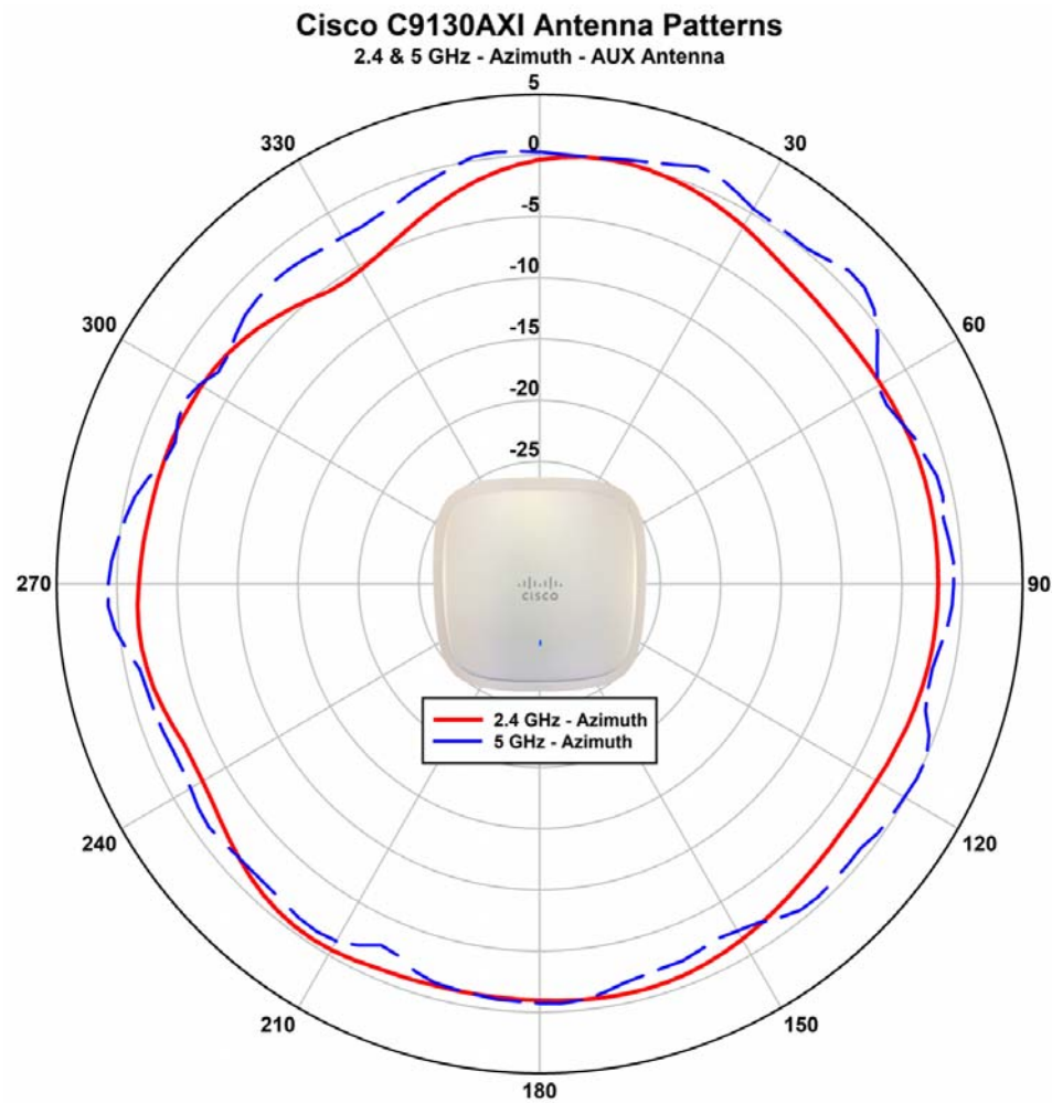
Figure 3-7 C9130AXI - AUX Antenna radiation pattern (2.4 GHz and 5 GHz Azimuth)
