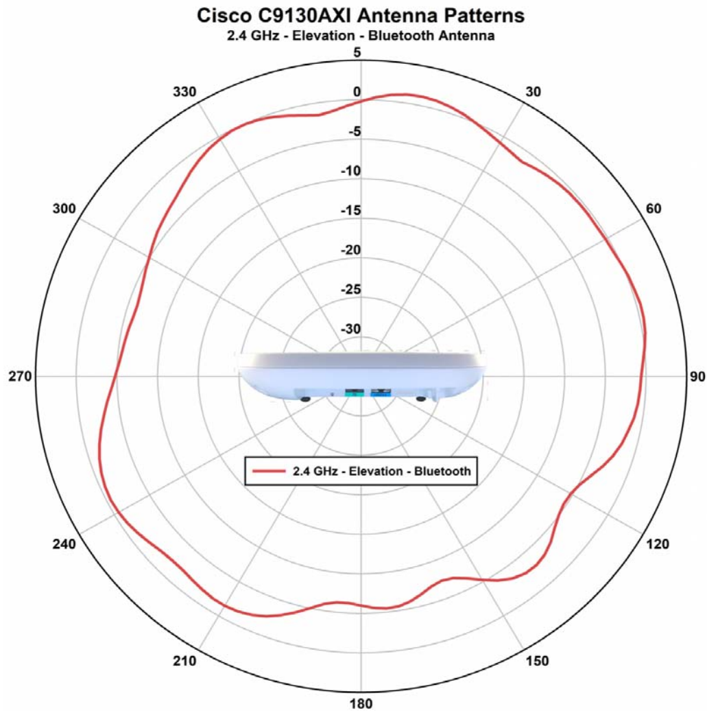
Figure 3-10 C9130AXI - Bluetooth Antenna radiation pattern (2.4 GHz Elevation)
