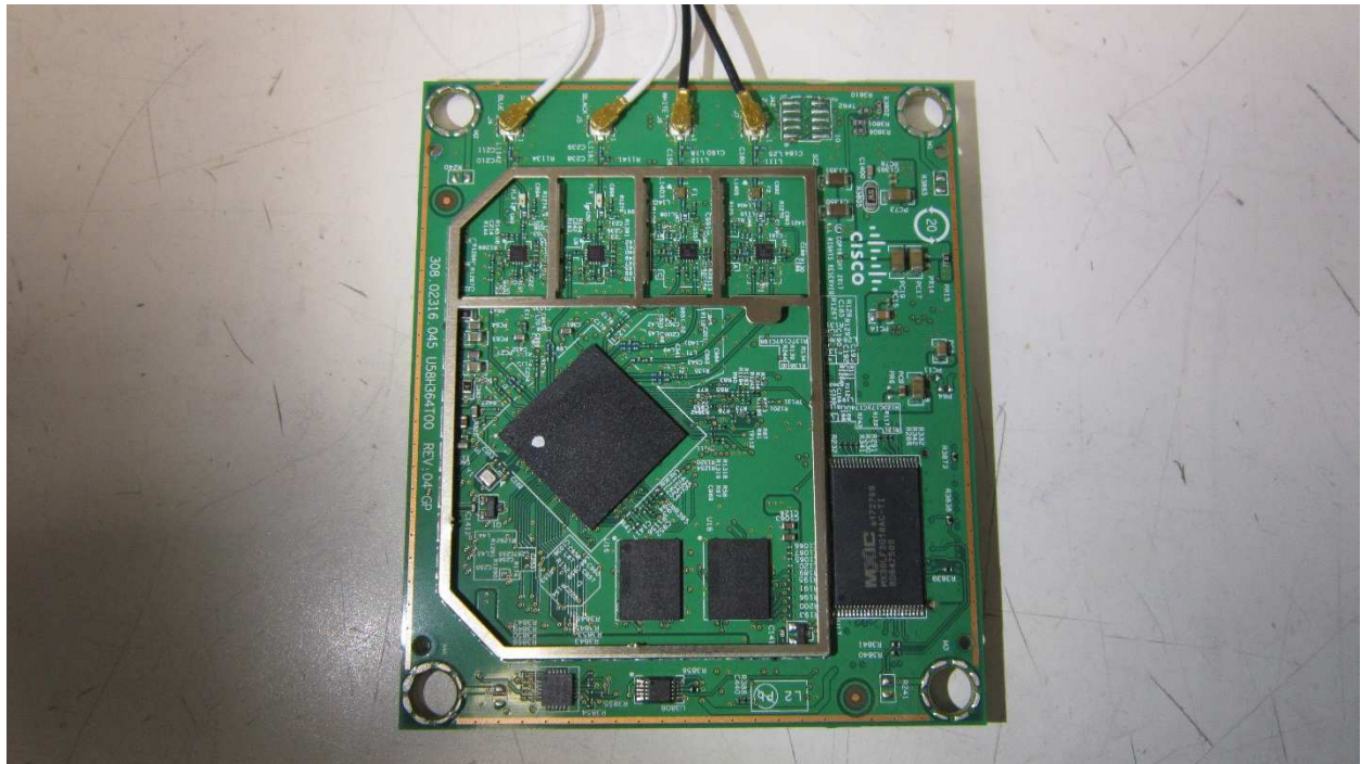
EUT Internal-Top View
