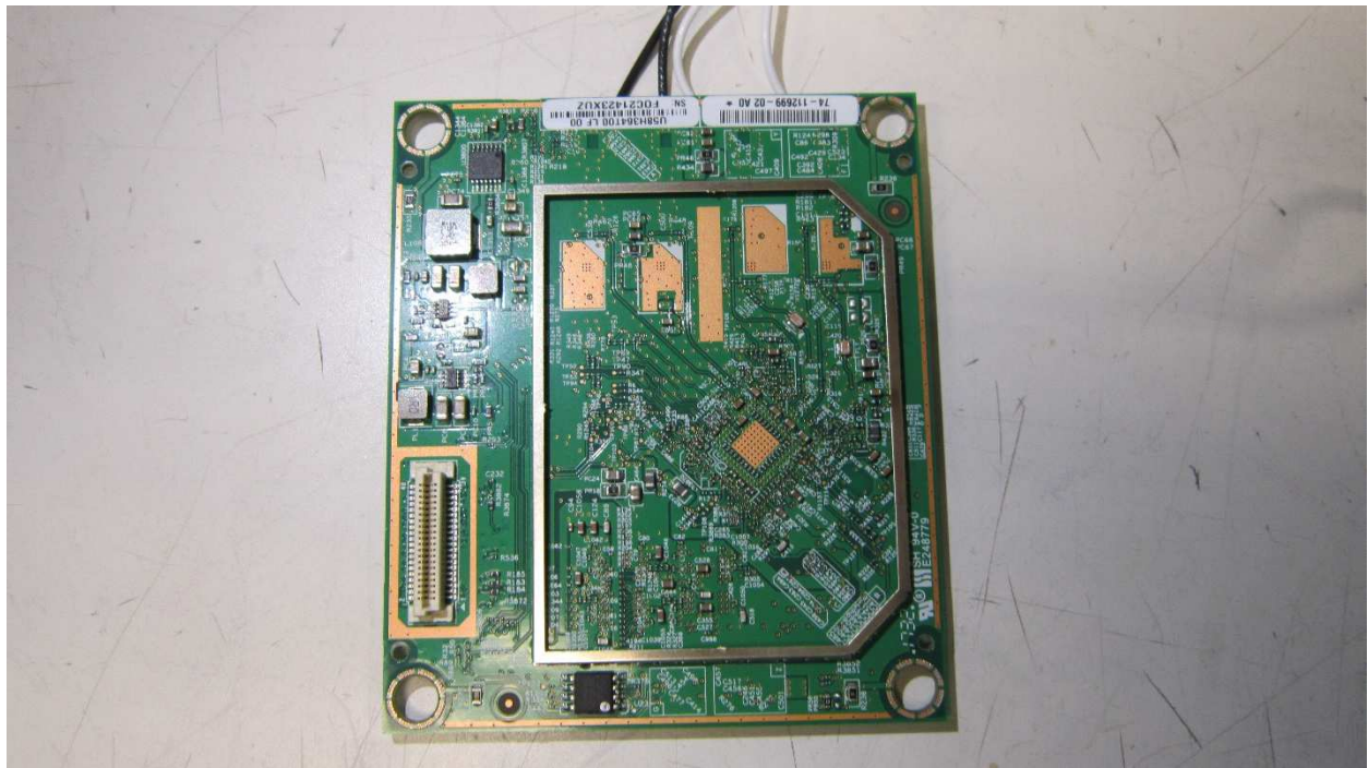
EUT Internal-Bottom View
