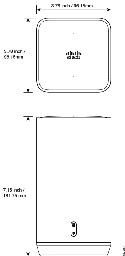
Figure 12: Product Dimensions
