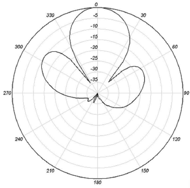
Figure 5: 2.4 GHz Ports BandD Elevation Plane
