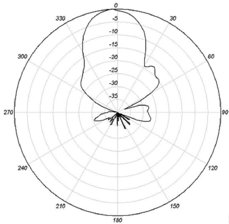
Figure 7: 5 GHz Ports AandC Elevation Plane
