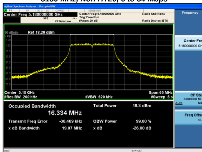
26dB-99% BW, 5180 MHz, Non HT20, 6 to 54 Mbps
