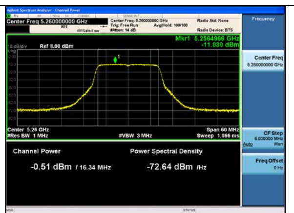
Antenna B
