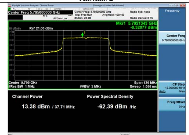
Antenna D
