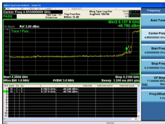
Antenna C
