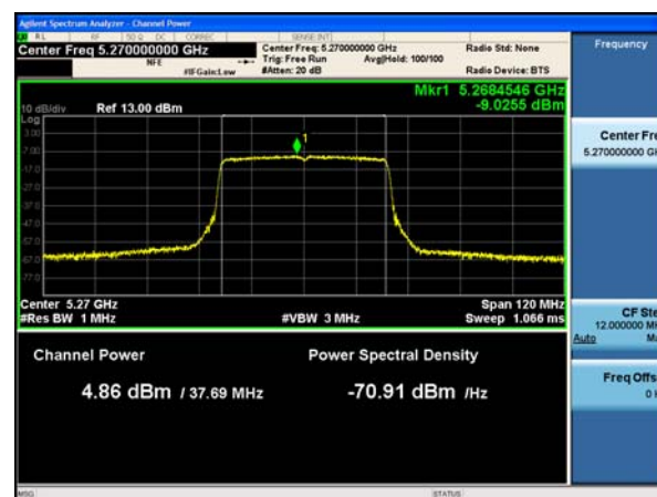
Antenna D
