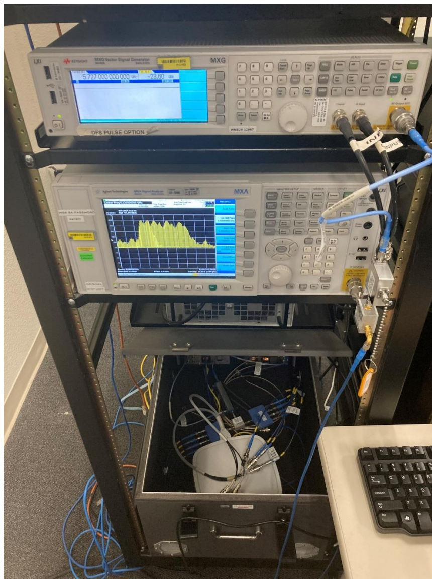
Photo from Zero Wait DFS testing
