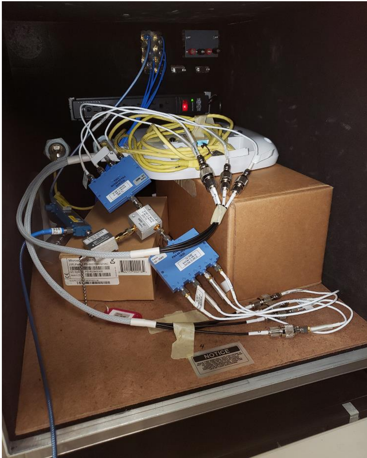
Title: Radio Conducted DFS Test Setup
