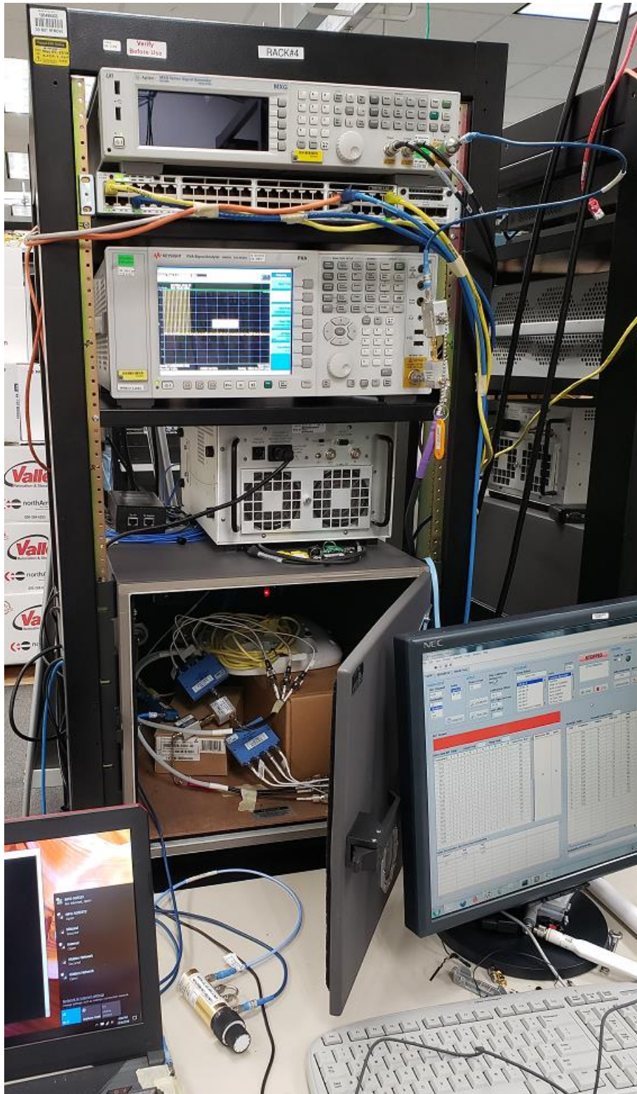
Title: Radio Conducted DFS Test Setup
