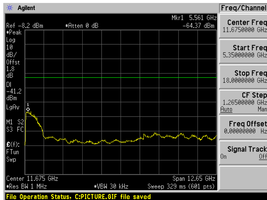
Ant-d-2
