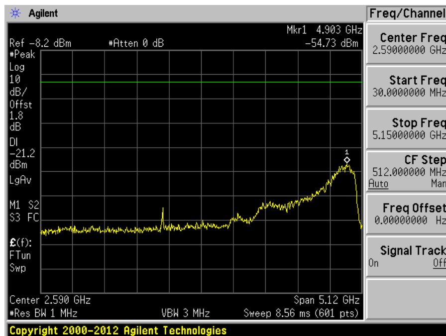
Ant-d-1
