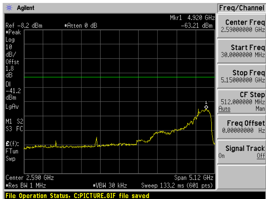
Ant-d-1
